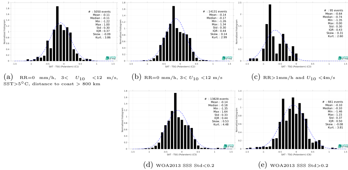
Figure 15: Normalized histogram of \Delta\text{SSS} (Aquarius SSS L2 OR v5 (NASA-GSFC) - TSG (Polarstern)) for 5 different subdatasets corresponding to: RR=0 mm/h, 3 < U_{10} < 12 m/s, SST > 5^\circ\text{C} , distance to coast > 800 km (a), RR=0 mm/h, 3 < U_{10} < 12 m/s (b), RR > 1 mm/h and U_{10} < 4 m/s (c), WOA2013 SSS Std < 0.2 (d), WOA2013 SSS Std > 0.2 (e).
