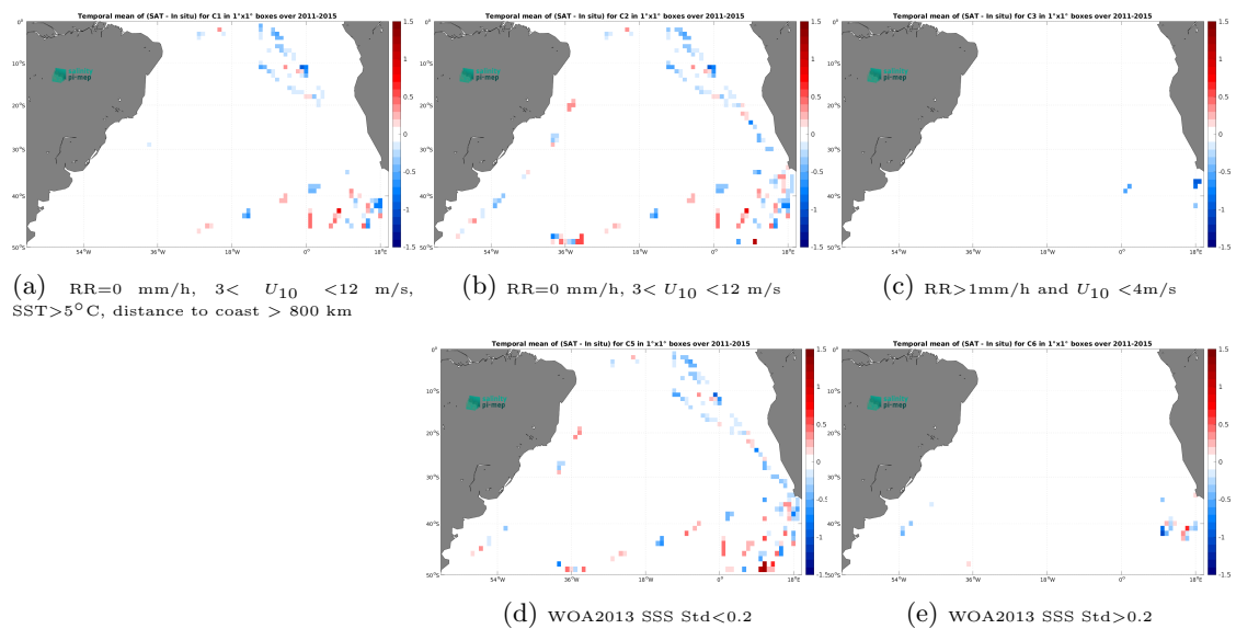
Figure 14: Temporal mean gridded over spatial boxes of size 1^\circ \times 1^\circ of \Delta\text{SSS} (Aquarius SSS L2 OR v5 (NASA-GSFC) - TSG (Polarstern)) for 5 different subdatasets corresponding to:RR=0 mm/h, 3 < U_{10} < 12 m/s, SST >5^\circ\text{C} , distance to coast > 800 km (a), RR=0 mm/h, 3 < U_{10} < 12 m/s (b), RR >1 mm/h and U_{10} < 4 m/s (c), WOA2013 SSS Std <0.2 (d), WOA2013 SSS Std >0.2 (e).
