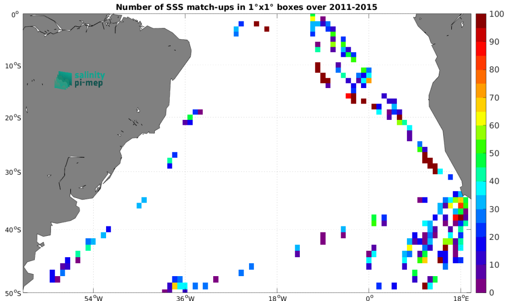
Figure 5: Number of SSS match-ups between TSG (Polarstern) SSS and the Aquarius SSS L2 OR v5 (NASA-GSFC) SSS product for the South Atlantic Ocean Pi-MEP region over 1^\circ \times 1^\circ boxes and for the full satellite product period.
