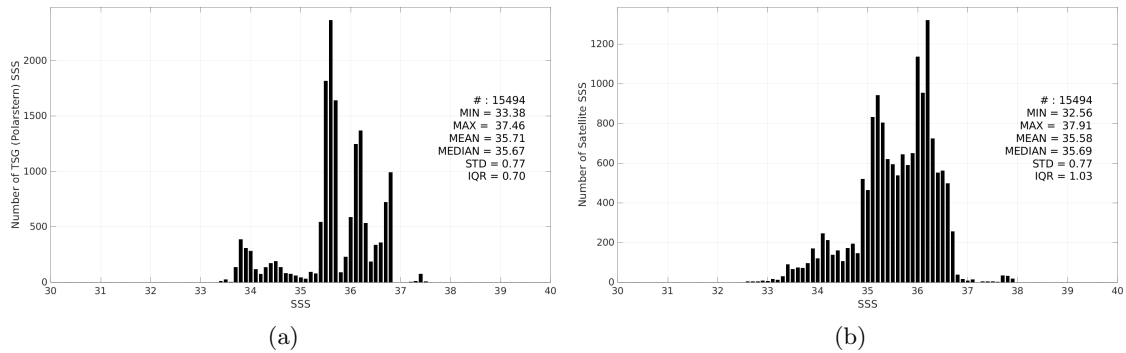
Figure 3: Histograms of SSS from TSG (Polarstern) (a) and Aquarius SSS L2 OR v5 (NASA-GSFC) (b) considering all match-up pairs per bins of 0.1 over the South Atlantic Ocean Pi-MEP region and for the full satellite product period.
