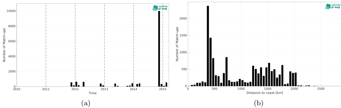
Figure 2: Number of match-ups between TSG (Polarstern) and Aquarius SSS L2 OR v5 (NASA-GSFC) SSS as a function of time (a) and as function of the distance to coast (b) over the South Atlantic Ocean Pi-MEP region and for the full satellite product period.
