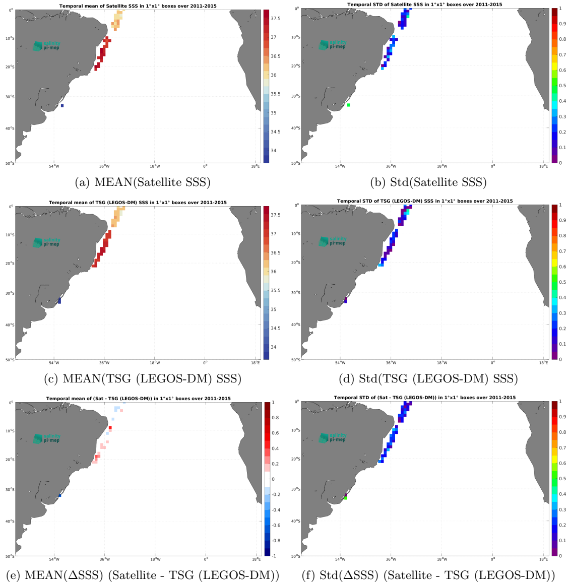
Figure 7: Temporal mean (left) and Std (right) of SSS from Aquarius SSS L2 OR v5 (NASA-GSFC) (top), TSG (LEGOS-DM) ( in situ ) dataset (middle), and of \Delta SSS (Satellite - TSG (LEGOS-DM)). Only match-up pairs are used to generate these maps.
