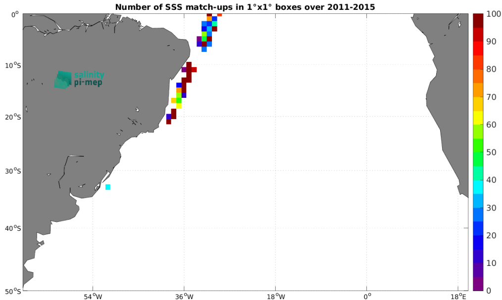
Figure 5: Number of SSS match-ups between TSG (LEGOS-DM) SSS and the Aquarius SSS L2 OR v5 (NASA-GSFC) SSS product for the South Atlantic Ocean Pi-MEP region over 1^\circ \times 1^\circ boxes and for the full satellite product period.
