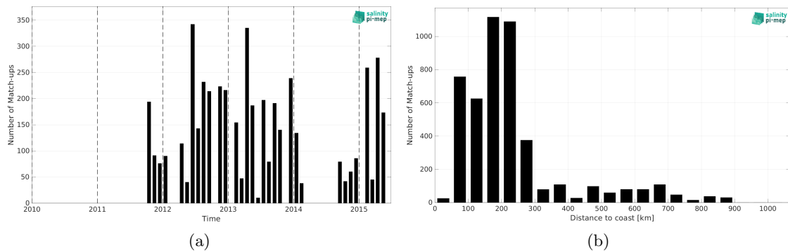
Figure 2: Number of match-ups between TSG (LEGOS-DM) and Aquarius SSS L2 OR v5 (NASA-GSFC) SSS as a function of time (a) and as function of the distance to coast (b) over the South Atlantic Ocean Pi-MEP region and for the full satellite product period.
