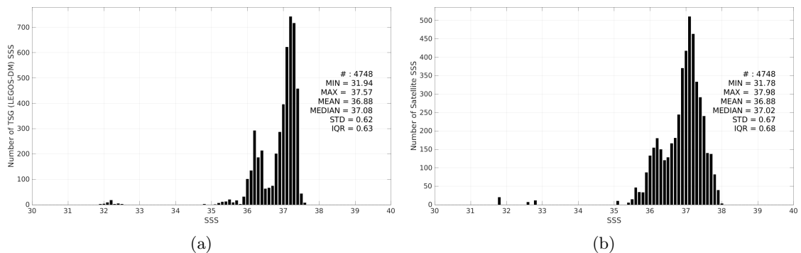
Figure 3: Histograms of SSS from TSG (LEGOS-DM) (a) and Aquarius SSS L2 OR v5 (NASA-GSFC) (b) considering all match-up pairs per bins of 0.1 over the South Atlantic Ocean Pi-MEP region and for the full satellite product period.
