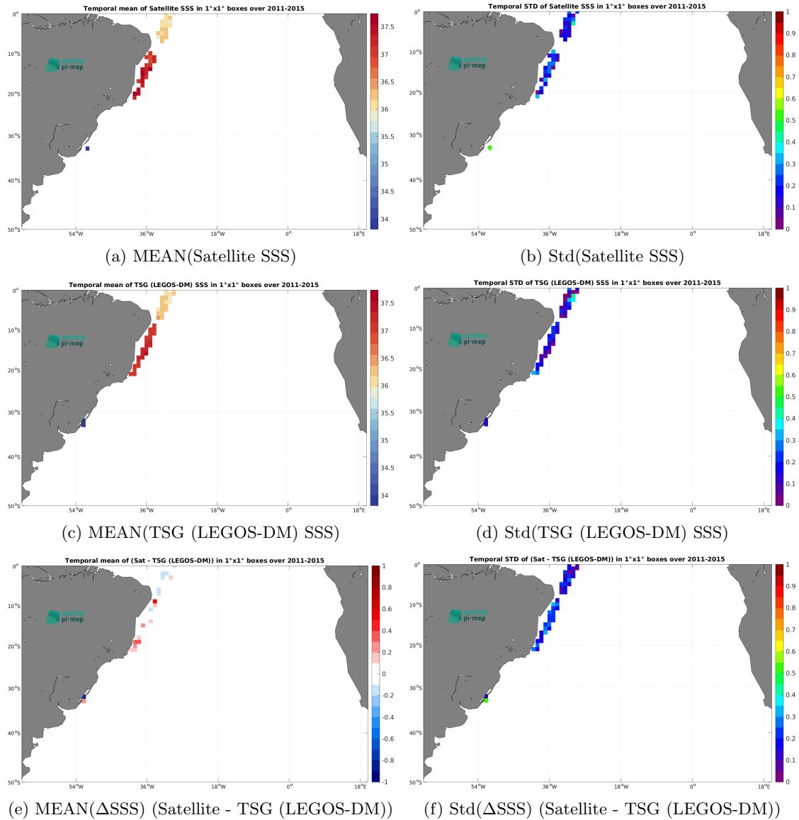
Figure 6: Temporal mean (left) and Std (right) of SSS from Aquarius SSS L2 OR v5 (NASA-GSFC) (top), TSG (LEGOS-DM) ( in situ ) dataset (middle), and of \Delta SSS (Satellite - TSG (LEGOS-DM)). Only match-up pairs are used to generate these maps.
