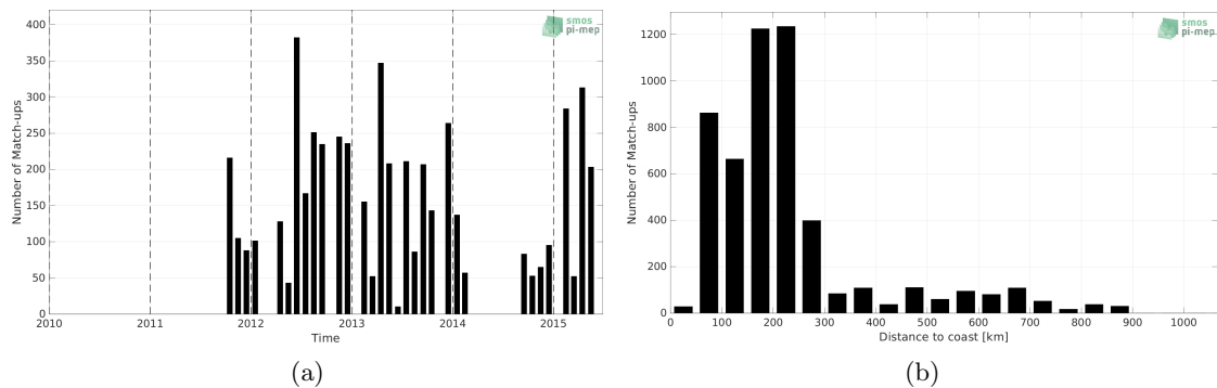
Figure 1: Number of match-ups between TSG (LEGOS-DM) and Aquarius SSS L2 OR v5 (NASA-GSFC) SSS as a function of time (a) and as function of the distance to coast (b) over the South Atlantic Ocean Pi-MEP region and for the full satellite product period.
