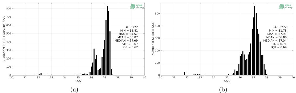
Figure 2: Histograms of SSS from TSG (LEGOS-DM) (a) and Aquarius SSS L2 OR v5 (NASA-GSFC) (b) considering all match-up pairs per bins of 0.1 over the South Atlantic Ocean Pi-MEP region and for the full satellite product period.
