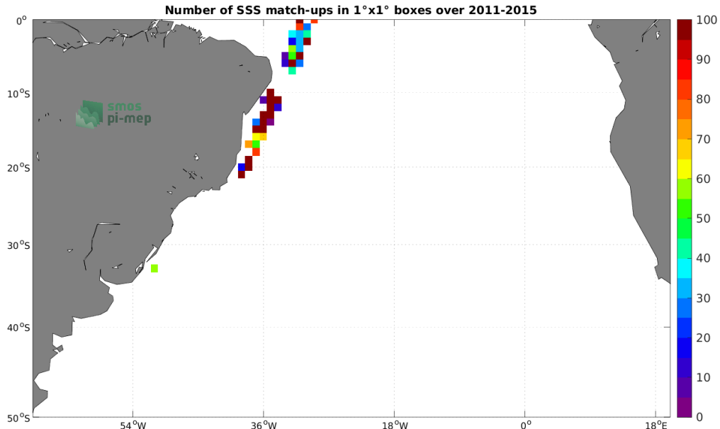
Figure 4: Number of SSS match-ups between TSG (LEGOS-DM) SSS and the Aquarius SSS L2 OR v5 (NASA-GSFC) SSS product for the South Atlantic Ocean Pi-MEP region over 1^\circ \times 1^\circ boxes and for the full satellite product period.
