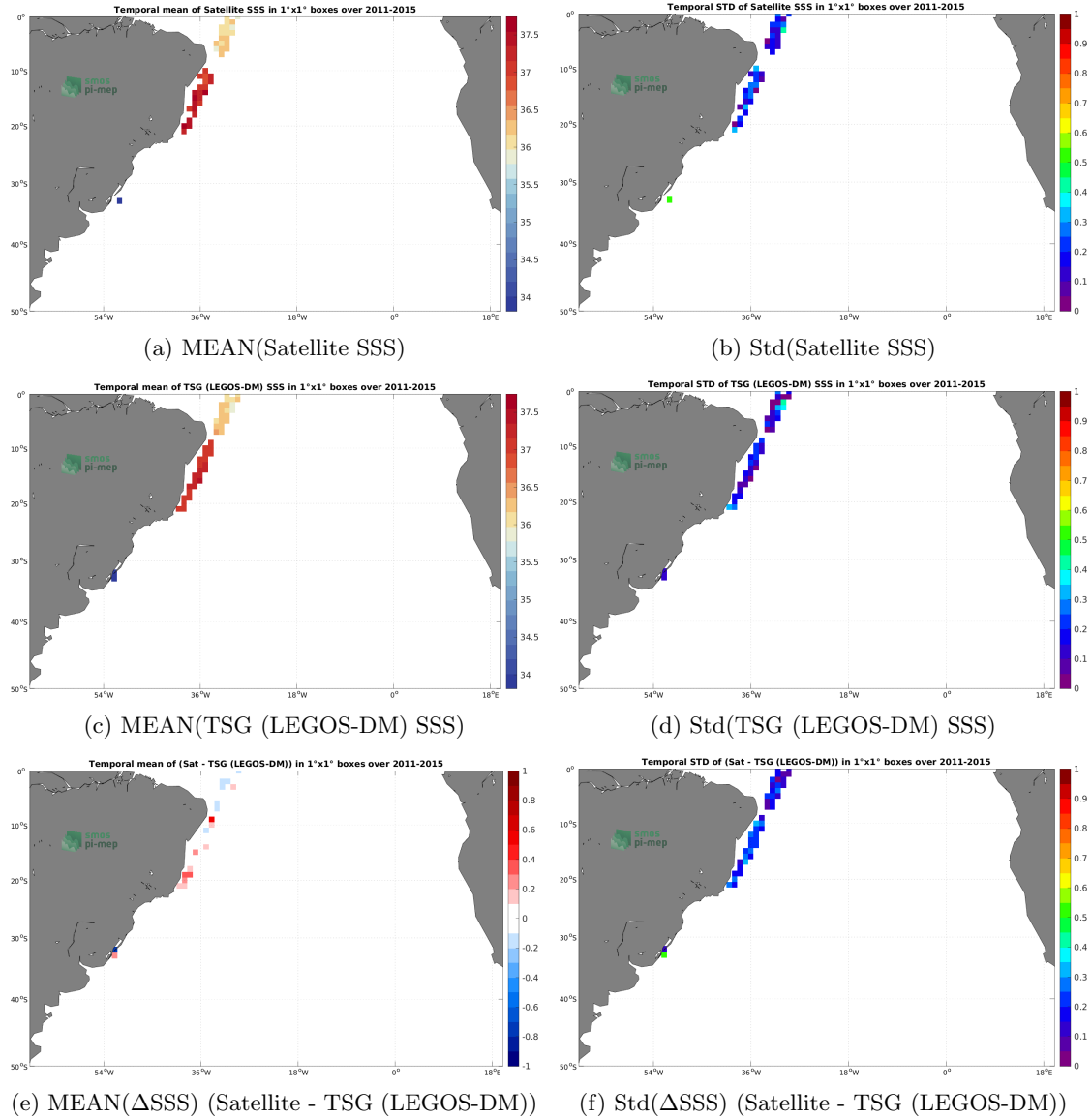
Figure 6: Temporal mean (left) and Std (right) of SSS from Aquarius SSS L2 OR v5 (NASA-GSFC) (top), TSG (LEGOS-DM) ( in situ ) dataset (middle), and of \Delta SSS (Satellite - TSG (LEGOS-DM)). Only match-up pairs are used to generate these maps.
