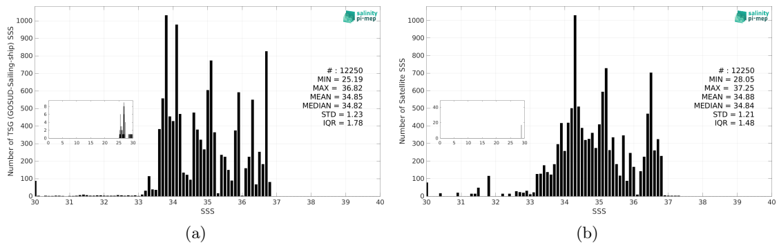
Figure 3: Histograms of SSS from TSG (GOSUD-Sailing-ship) (a) and Aquarius SSS L2 OR v5 (NASA-GSFC) (b) considering all match-up pairs per bins of 0.1 over the South Atlantic Ocean Pi-MEP region and for the full satellite product period.
