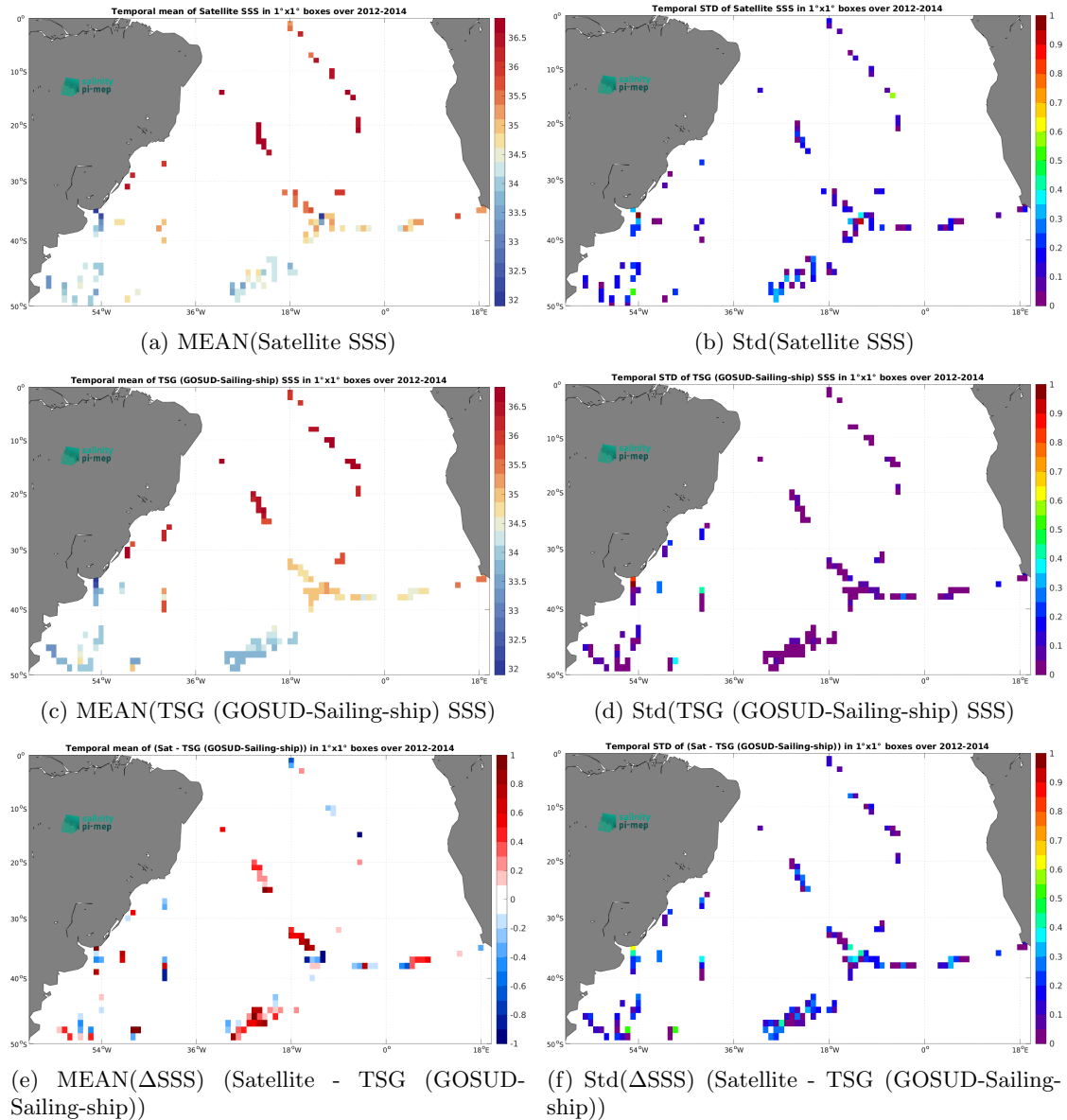
Figure 7: Temporal mean (left) and Std (right) of SSS from Aquarius SSS L2 OR v5 (NASA-GSFC) (top), TSG (GOSUD-Sailing-ship) (middle), and of \Delta SSS (Satellite - TSG (GOSUD-Sailing-ship)). Only match-up pairs are used to generate these maps.
