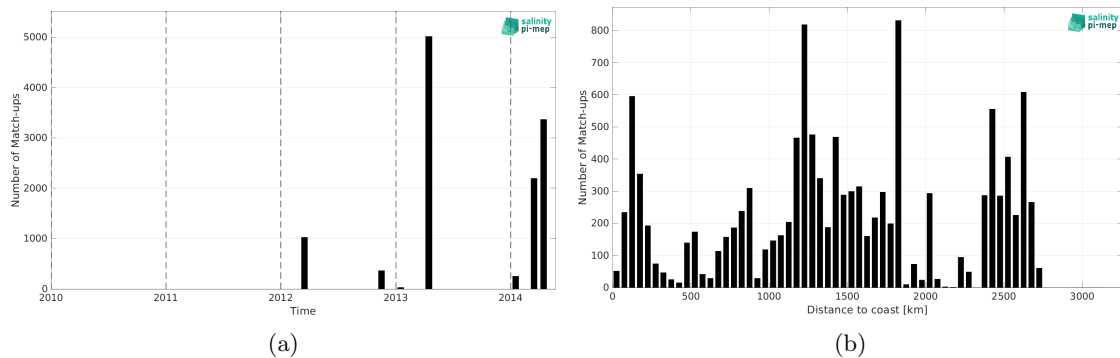
Figure 2: Number of match-ups between TSG (GOSUD-Sailing-ship) and Aquarius SSS L2 OR v5 (NASA-GSFC) SSS as a function of time (a) and as function of the distance to coast (b) over the South Atlantic Ocean Pi-MEP region and for the full satellite product period.
