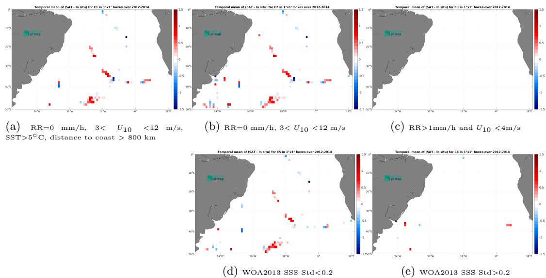
Figure 14: Temporal mean gridded over spatial boxes of size 1^\circ \times 1^\circ of \Delta\text{SSS} (Aquarius SSS L2 OR v5 (NASA-GSFC) - TSG (GOSUD-Sailing-ship)) for 5 different subdatasets corresponding to:RR=0 mm/h, 3 < U_{10} < 12 m/s, SST >5^\circ\text{C} , distance to coast > 800 km (a), RR=0 mm/h, 3 < U_{10} < 12 m/s (b), RR >1 mm/h and U_{10} < 4 m/s (c), WOA2013 SSS Std <0.2 (d), WOA2013 SSS Std >0.2 (e).
