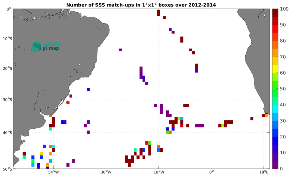
Figure 5: Number of SSS match-ups between TSG (GOSUD-Sailing-ship) SSS and the Aquarius SSS L2 OR v5 (NASA-GSFC) SSS product for the South Atlantic Ocean Pi-MEP region over 1^\circ \times 1^\circ boxes and for the full satellite product period.
