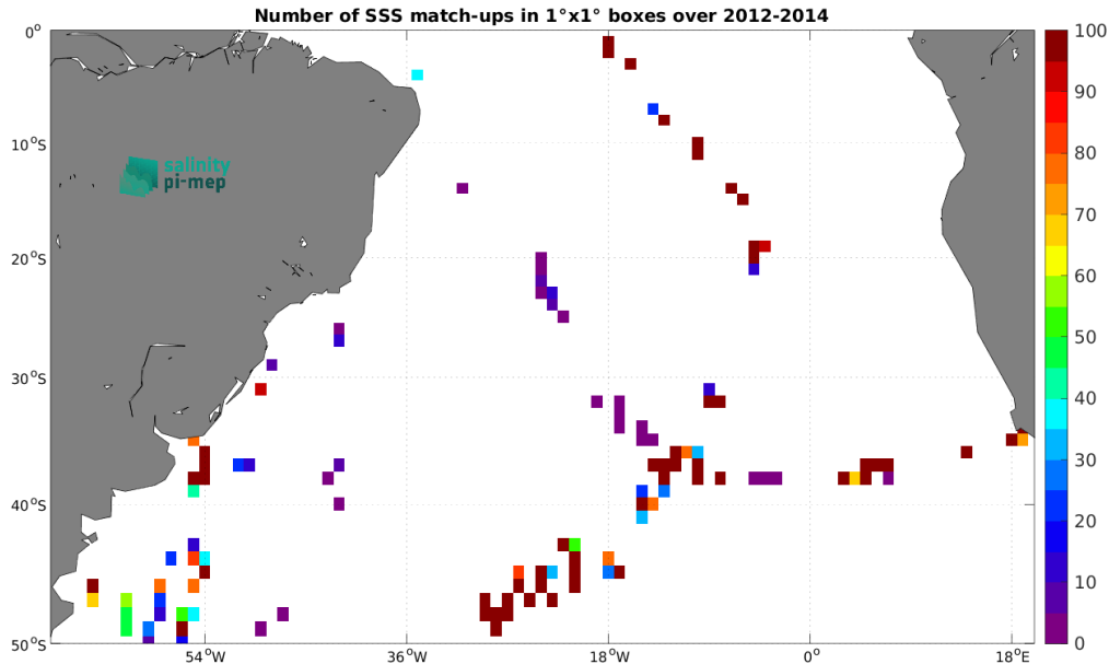
Figure 4: Number of SSS match-ups between TSG (GOSUD-Sailing-ship) SSS and the Aquarius SSS L2 OR v5 (NASA-GSFC) SSS product for the South Atlantic Ocean Pi-MEP region over 1^\circ \times 1^\circ boxes and for the full satellite product period.
