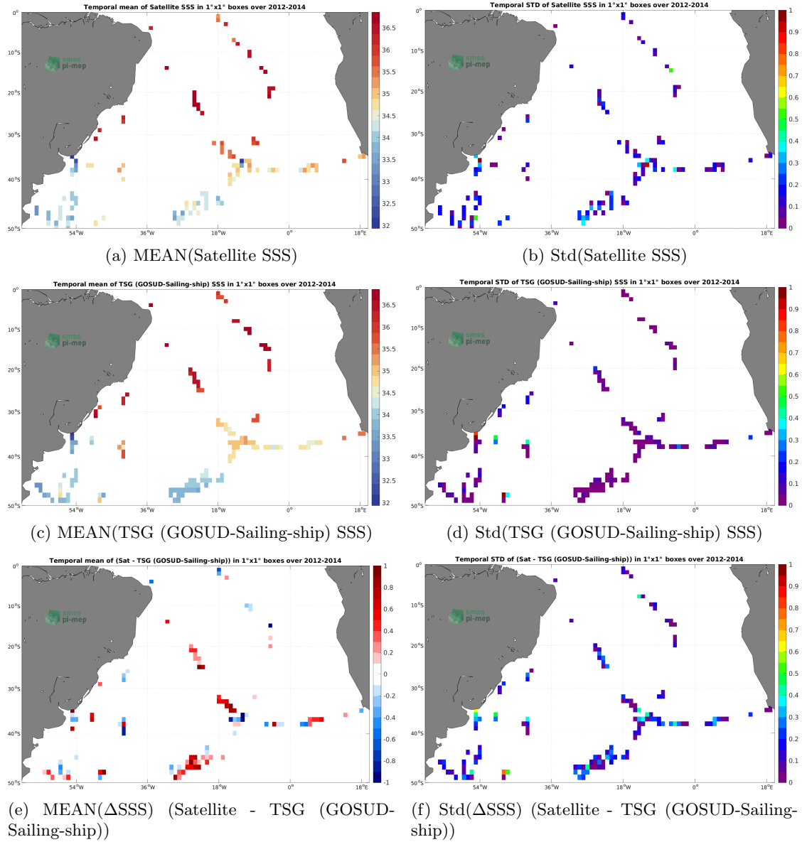
Figure 6: Temporal mean (left) and Std (right) of SSS from Aquarius SSS L2 OR v5 (NASA-GSFC) (top), TSG (GOSUD-Sailing-ship) (middle), and of \Delta SSS (Satellite - TSG (GOSUD-Sailing-ship)). Only match-up pairs are used to generate these maps.
