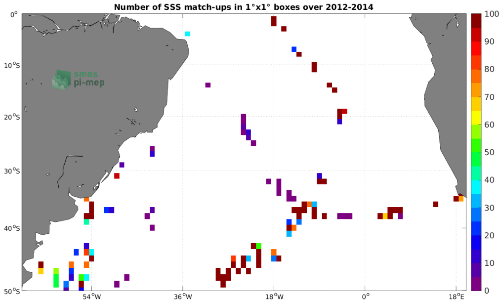
Figure 4: Number of SSS match-ups between TSG (GOSUD-Sailing-ship) SSS and the Aquarius SSS L2 OR v5 (NASA-GSFC) SSS product for the South Atlantic Ocean Pi-MEP region over 1^{\circ} \times 1^{\circ} boxes and for the full satellite product period.
