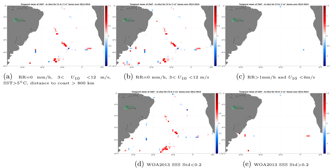
Figure 12: Temporal mean gridded over spatial boxes of size 1^\circ \times 1^\circ of \Delta SSS (Aquarius SSS L2 OR v5 (NASA-GSFC) - TSG (GOSUD-Sailing-ship)) for 5 different subdatasets corresponding to:RR=0 mm/h, 3 < U_{10} < 12 m/s, SST>5°C, distance to coast > 800 km (a), RR=0 mm/h, 3 < U_{10} < 12 m/s (b), RR>1mm/h and U_{10} < 4 m/s (c), WOA2013 SSS Std<0.2 (d), WOA2013 SSS Std>0.2 (e).
