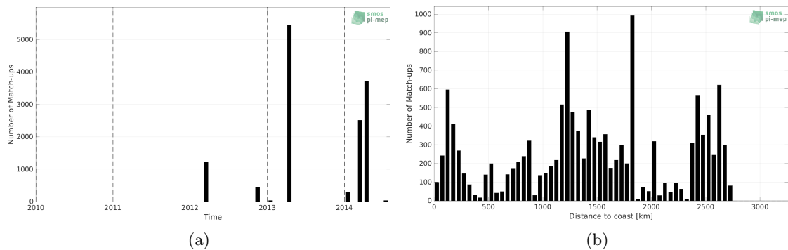
Figure 1: Number of match-ups between TSG (GOSUD-Sailing-ship) and Aquarius SSS L2 OR v5 (NASA-GSFC) SSS as a function of time (a) and as function of the distance to coast (b) over the South Atlantic Ocean Pi-MEP region and for the full satellite product period.
