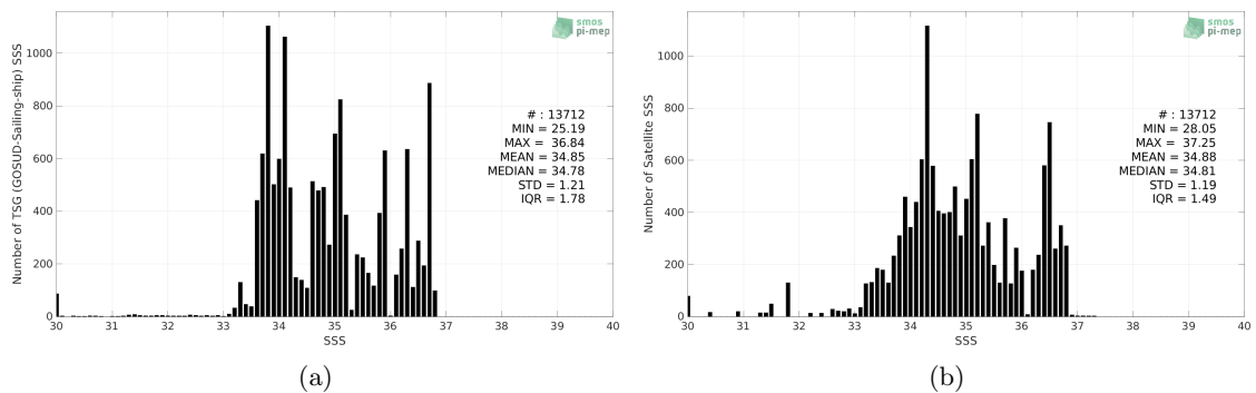
Figure 2: Histograms of SSS from TSG (GOSUD-Sailing-ship) (a) and Aquarius SSS L2 OR v5 (NASA-GSFC) (b) considering all match-up pairs per bins of 0.1 over the South Atlantic Ocean Pi-MEP region and for the full satellite product period.
