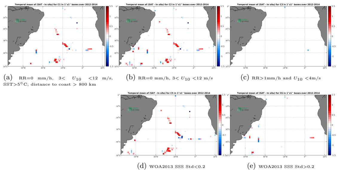
Figure 12: Temporal mean gridded over spatial boxes of size 1^\circ \times 1^\circ of \Delta SSS (Aquarius-L2-OR-V5 - TSG-GOSUD-Sailing-ship) for 5 different subdatasets corresponding to:RR=0 mm/h, 3 < U_{10} < 12 m/s, SST >5^\circ C, distance to coast > 800 km (a), RR=0 mm/h, 3 < U_{10} < 12 m/s (b), RR >1 mm/h and U_{10} < 4 m/s (c), WOA2013 SSS Std <0.2 (d), WOA2013 SSS Std >0.2 (e).
