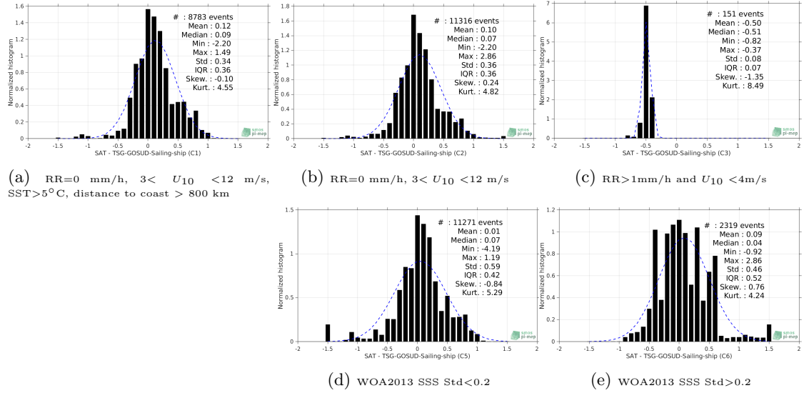
Figure 13: Normalized histogram of \Delta SSS (Aquarius-L2-OR-V5 - TSG-GOSUD-Sailing-ship) for 5 different subdatasets corresponding to: RR=0 mm/h, 3 < U_{10} < 12 m/s, SST > 5°C, distance to coast > 800 km (a), RR=0 mm/h, 3 < U_{10} < 12 m/s (b), RR > 1mm/h and U_{10} < 4 m/s (c), WOA2013 SSS Std < 0.2 (d), WOA2013 SSS Std > 0.2 (e).
