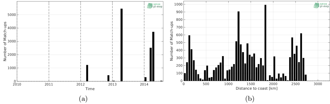
Figure 1: Number of match-ups between TSG-GOSUD-Sailing-ship and Aquarius-L2-OR-V5 SSS as a function of time (a) and as function of the distance to coast (b) over the South Atlantic Ocean Pi-MEP region and for the full satellite product period.
