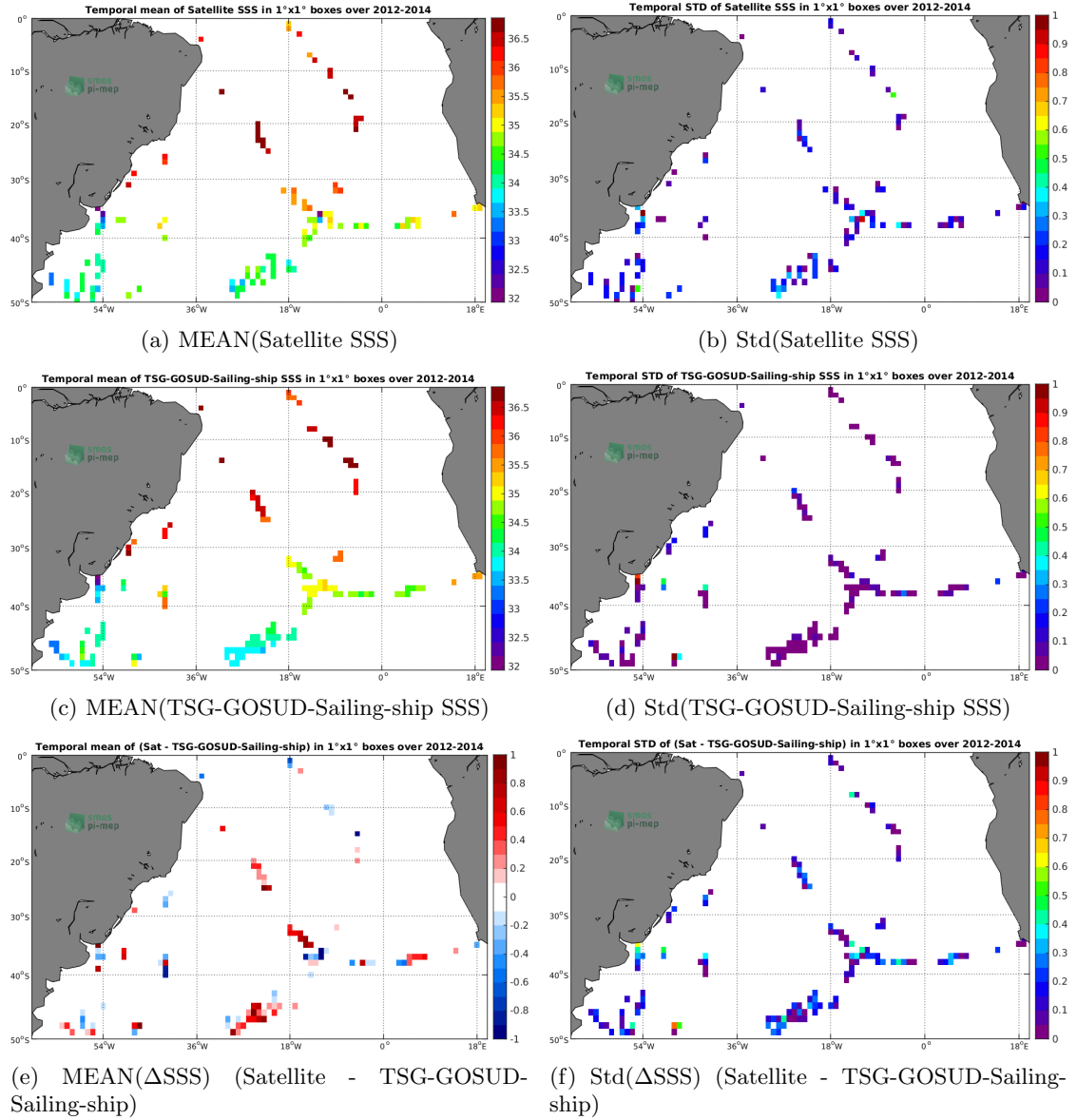
Figure 6: Temporal mean (left) and Std (right) of SSS from Aquarius-L2-OR-V5 (top), TSG-GOSUD-Sailing-ship (middle), and of \Delta SSS (Satellite - TSG-GOSUD-Sailing-ship). Only match-up pairs are used to generate these maps.
