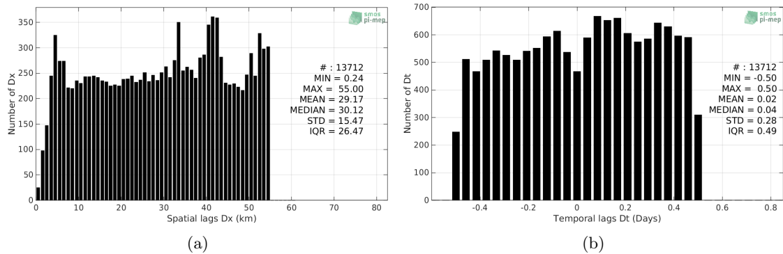
Figure 5: Histograms of the spatial (a) and temporal (b) lags between the time of the TSG-GOSUD-Sailing-ship measurements and the date of the corresponding Aquarius-L2-OR-V5 SSS product.
