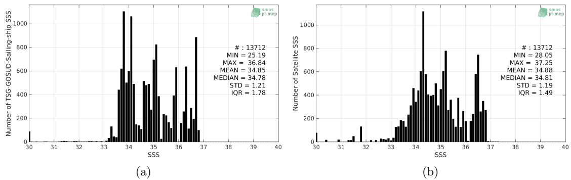
Figure 2: Histograms of SSS from TSG-GOSUD-Sailing-ship (a) and Aquarius-L2-OR-V5 (b) considering all match-up pairs per bins of 0.1 over the South Atlantic Ocean Pi-MEP region and for the full satellite product period.
