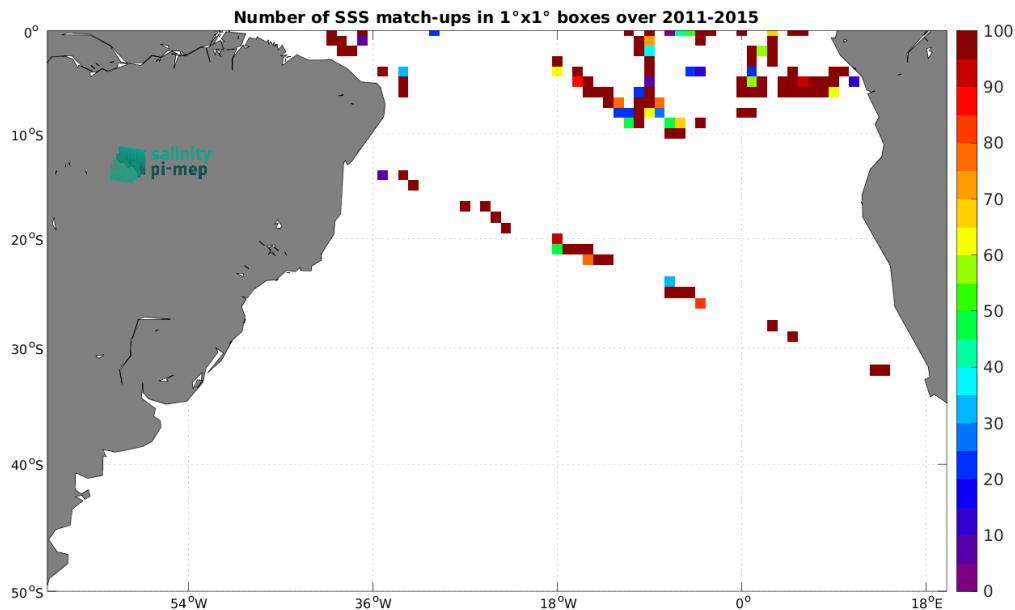
Figure 5: Number of SSS match-ups between TSG (GOSUD-Research-vessel) SSS and the Aquarius SSS L2 OR v5 (NASA-GSFC) SSS product for the South Atlantic Ocean Pi-MEP region over 1^\circ \times 1^\circ boxes and for the full satellite product period.
