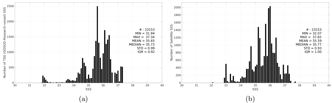
Figure 3: Histograms of SSS from TSG (GOSUD-Research-vessel) (a) and Aquarius SSS L2 OR v5 (NASA-GSFC) (b) considering all match-up pairs per bins of 0.1 over the South Atlantic Ocean Pi-MEP region and for the full satellite product period.
