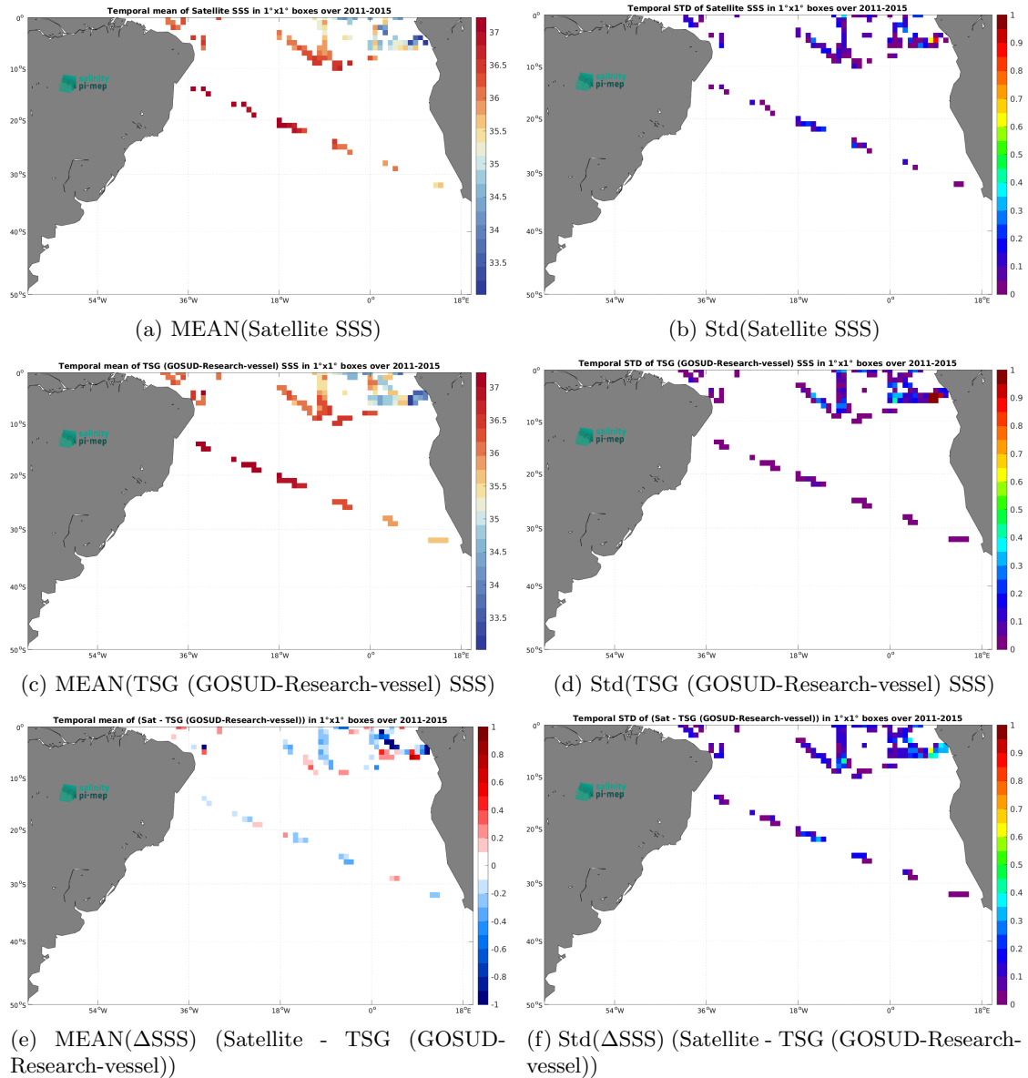
Figure 7: Temporal mean (left) and Std (right) of SSS from Aquarius SSS L2 OR v5 (NASA-GSFC) (top), TSG (GOSUD-Research-vessel) (middle), and of \Delta SSS (Satellite - TSG (GOSUD-Research-vessel)). Only match-up pairs are used to generate these maps.
