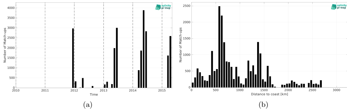
Figure 2: Number of match-ups between TSG (GOSUD-Research-vessel) and Aquarius SSS L2 OR v5 (NASA-GSFC) SSS as a function of time (a) and as function of the distance to coast (b) over the South Atlantic Ocean Pi-MEP region and for the full satellite product period.
