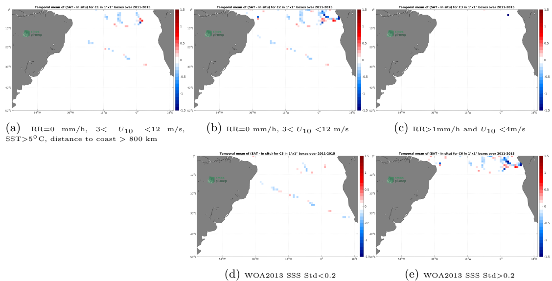
Figure 12: Temporal mean gridded over spatial boxes of size 1^\circ \times 1^\circ of \Delta SSS (Aquarius SSS L2 OR v5 (NASA-GSFC) - TSG (GOSUD-Research-vessel)) for 5 different subdatasets corresponding to: RR=0 mm/h, 3 < U_{10} < 12 m/s, SST > 5°C, distance to coast > 800 km (a), RR=0 mm/h, 3 < U_{10} < 12 m/s (b), RR > 1mm/h and U_{10} < 4 m/s (c), WOA2013 SSS Std < 0.2 (d), WOA2013 SSS Std > 0.2 (e).
