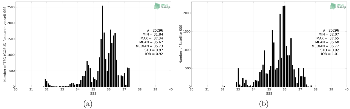
Figure 2: Histograms of SSS from TSG (GOSUD-Research-vessel) (a) and Aquarius SSS L2 OR v5 (NASA-GSFC) (b) considering all match-up pairs per bins of 0.1 over the South Atlantic Ocean Pi-MEP region and for the full satellite product period.
