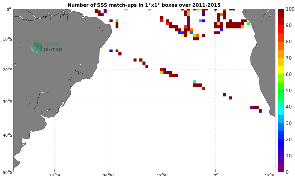
Figure 4: Number of SSS match-ups between TSG (GOSUD-Research-vessel) SSS and the Aquarius SSS L2 OR v5 (NASA-GSFC) SSS product for the South Atlantic Ocean Pi-MEP region over 1^\circ \times 1^\circ boxes and for the full satellite product period.
