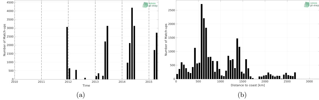
Figure 1: Number of match-ups between TSG (GOSUD-Research-vessel) and Aquarius SSS L2 OR v5 (NASA-GSFC) SSS as a function of time (a) and as function of the distance to coast (b) over the South Atlantic Ocean Pi-MEP region and for the full satellite product period.
