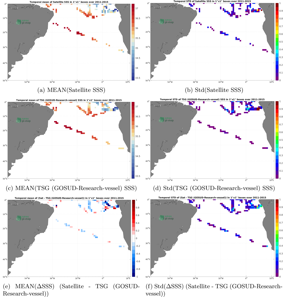
Figure 6: Temporal mean (left) and Std (right) of SSS from Aquarius SSS L2 OR v5 (NASA-GSFC) (top), TSG (GOSUD-Research-vessel) (middle), and of \Delta SSS (Satellite - TSG (GOSUD-Research-vessel)). Only match-up pairs are used to generate these maps.
