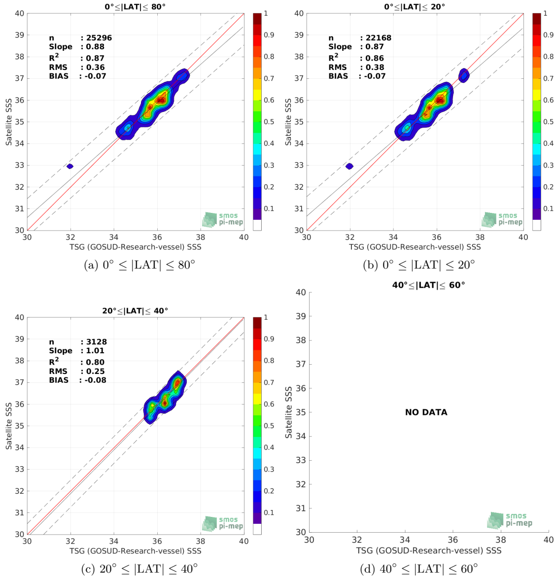
Figure 9: Contour maps of the concentration of Aquarius SSS L2 OR v5 (NASA-GSFC) SSS (y-axis) versus TSG (GOSUD-Research-vessel) SSS (x-axis) at match-up pairs for different latitude bands. For each plot, the red line shows x=y . The black thin and dashed lines indicate a linear fit through the data cloud and the \pm 95\% confidence levels, respectively. The number match-up pairs n , the slope and R^2 coefficient of the linear fit, the root mean square (RMS) and the mean bias between satellite and in situ data are indicated for each latitude band in each plots.
