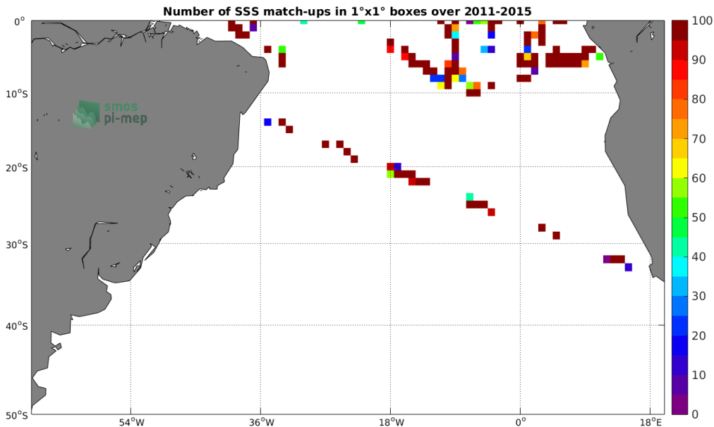
Figure 4: Number of SSS match-ups between TSG-GOSUD-Research-vessel SSS and the Aquarius-L2-OR-V5 SSS product for the South Atlantic Ocean Pi-MEP region over 1°x1° boxes and for the full satellite product period.
