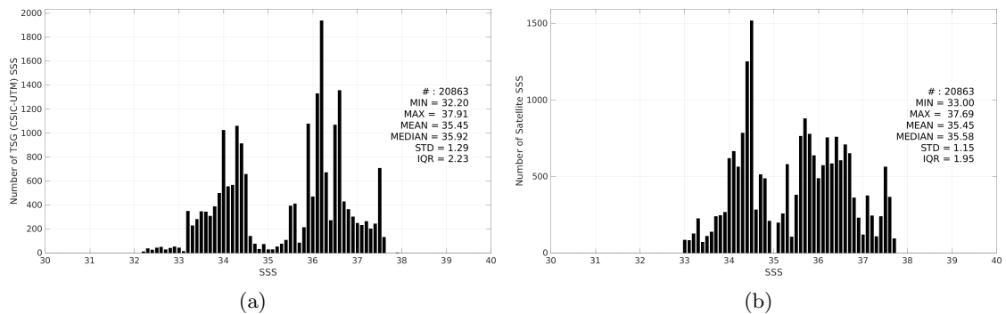
Figure 3: Histograms of SSS from TSG (CSIC-UTM) (a) and Aquarius SSS L2 OR v5 (NASA-GSFC) (b) considering all match-up pairs per bins of 0.1 over the South Atlantic Ocean Pi-MEP region and for the full satellite product period.
