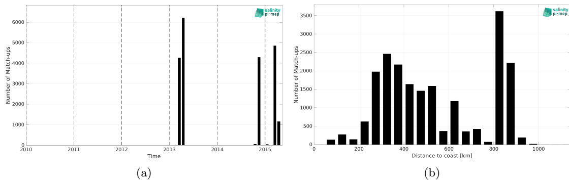
Figure 2: Number of match-ups between TSG (CSIC-UTM) and Aquarius SSS L2 OR v5 (NASA-GSFC) SSS as a function of time (a) and as function of the distance to coast (b) over the South Atlantic Ocean Pi-MEP region and for the full satellite product period.
