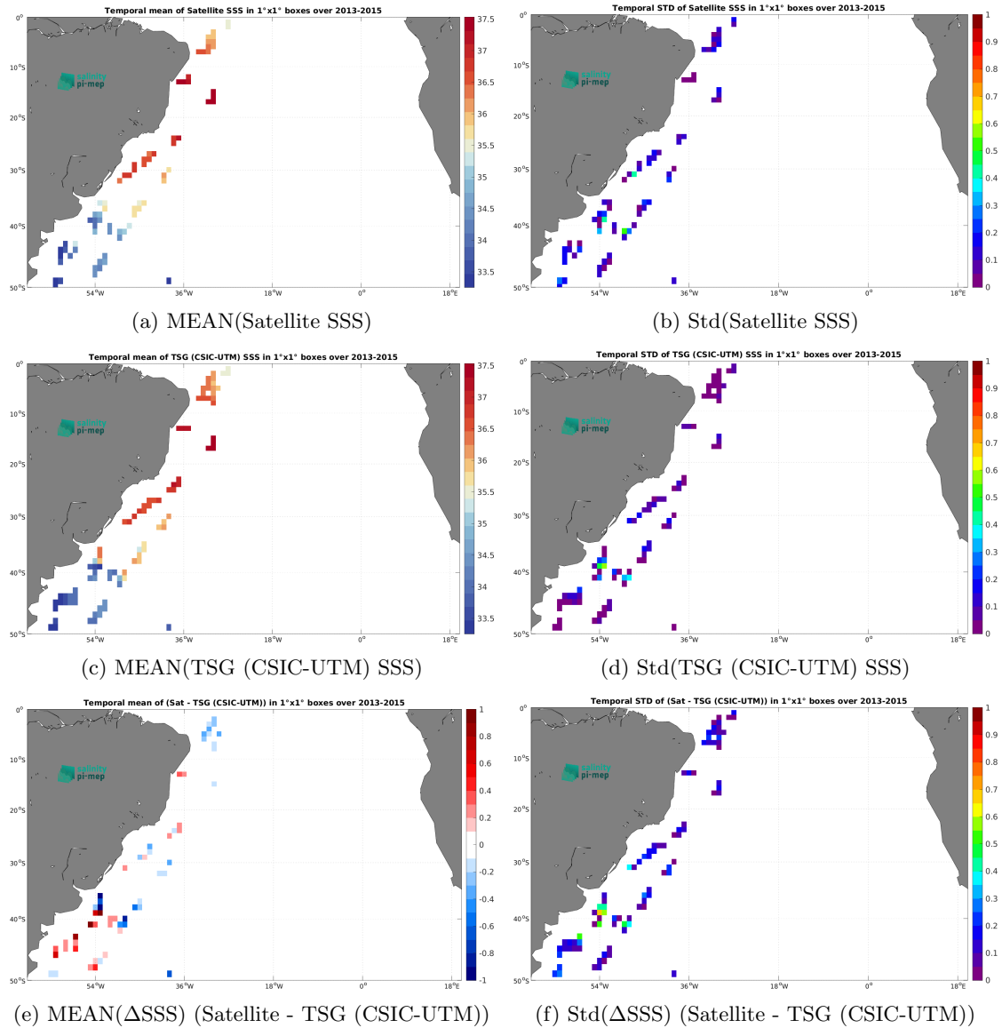
Figure 7: Temporal mean (left) and Std (right) of SSS from Aquarius SSS L2 OR v5 (NASA-GSFC) (top), TSG (CSIC-UTM) (middle), and of \Delta SSS (Satellite - TSG (CSIC-UTM)). Only match-up pairs are used to generate these maps.
