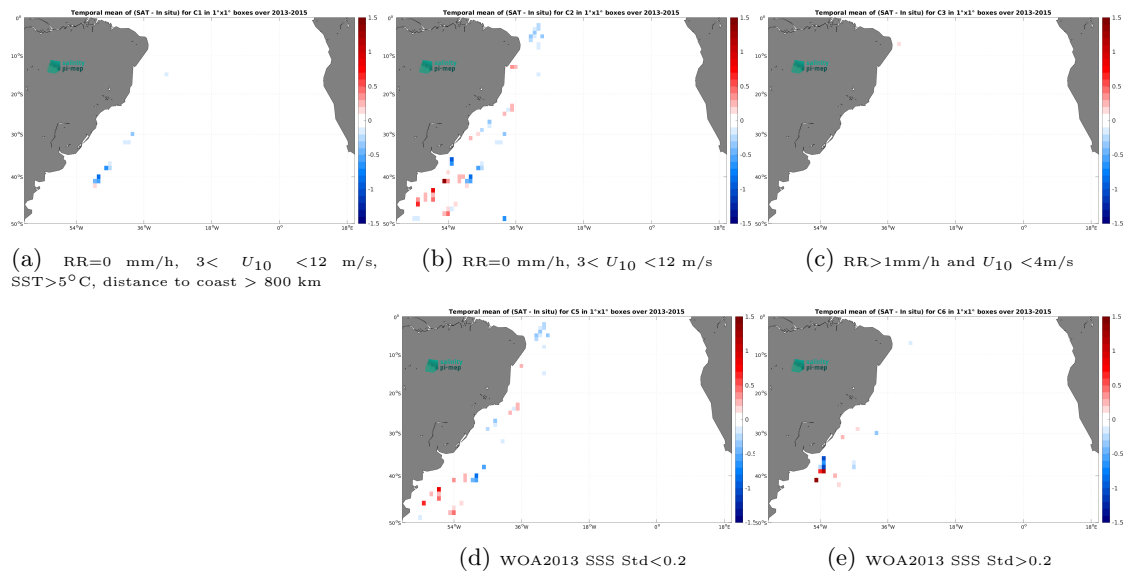
Figure 14: Temporal mean gridded over spatial boxes of size 1^\circ \times 1^\circ of \Delta SSS (Aquarius SSS L2 OR v5 (NASA-GSFC) - TSG (CSIC-UTM)) for 5 different subdatasets corresponding to:RR=0 mm/h, 3 < U_{10} < 12 m/s, SST >5^\circ\text{C} , distance to coast > 800 km (a), RR=0 mm/h, 3 < U_{10} < 12 m/s (b), RR >1 mm/h and U_{10} < 4 m/s (c), WOA2013 SSS Std <0.2 (d), WOA2013 SSS Std >0.2 (e).
