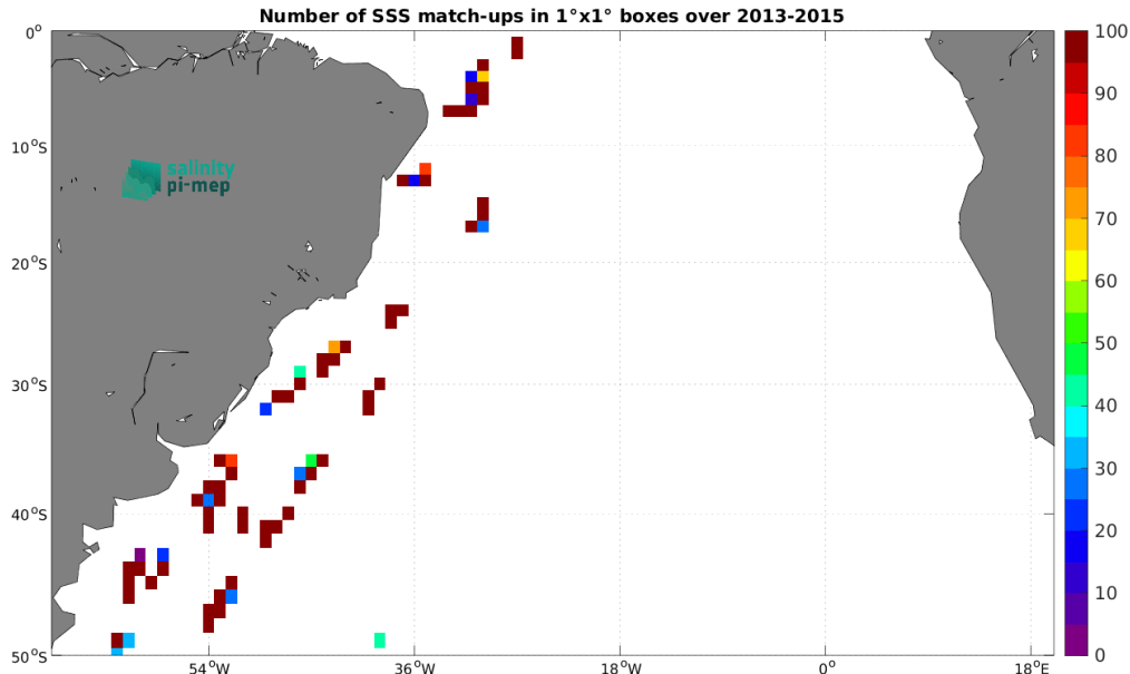
Figure 5: Number of SSS match-ups between TSG (CSIC-UTM) SSS and the Aquarius SSS L2 OR v5 (NASA-GSFC) SSS product for the South Atlantic Ocean Pi-MEP region over 1^\circ \times 1^\circ boxes and for the full satellite product period.
