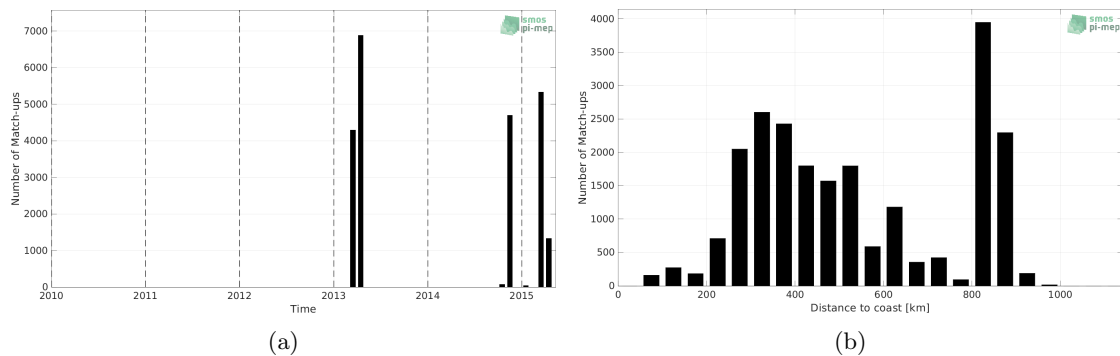
Figure 1: Number of match-ups between TSG (CSIC-UTM) and Aquarius SSS L2 OR v5 (NASA-GSFC) SSS as a function of time (a) and as function of the distance to coast (b) over the South Atlantic Ocean Pi-MEP region and for the full satellite product period.
