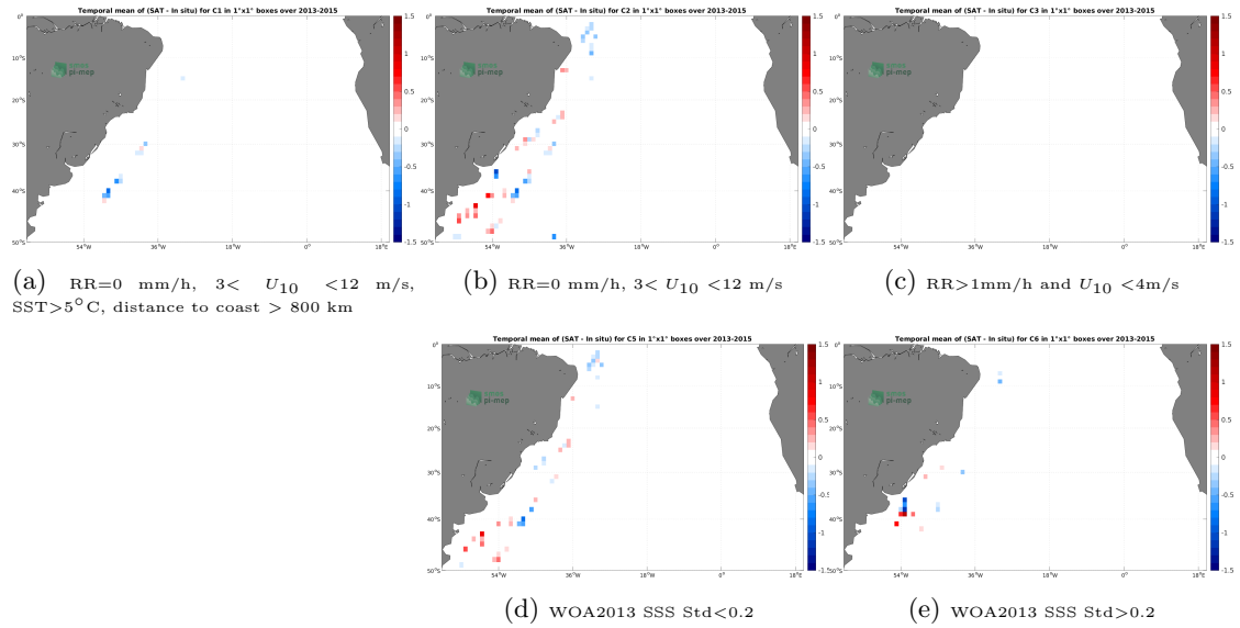
Figure 12: Temporal mean gridded over spatial boxes of size 1^\circ \times 1^\circ of \Delta SSS (Aquarius SSS L2 OR v5 (NASA-GSFC) - TSG (CSIC-UTM)) for 5 different subdatasets corresponding to:RR=0 mm/h, 3 < U_{10} < 12 m/s, SST >5^\circ\text{C} , distance to coast > 800 km (a), RR=0 mm/h, 3 < U_{10} < 12 m/s (b), RR >1 mm/h and U_{10} < 4 m/s (c), WOA2013 SSS Std <0.2 (d), WOA2013 SSS Std >0.2 (e).
