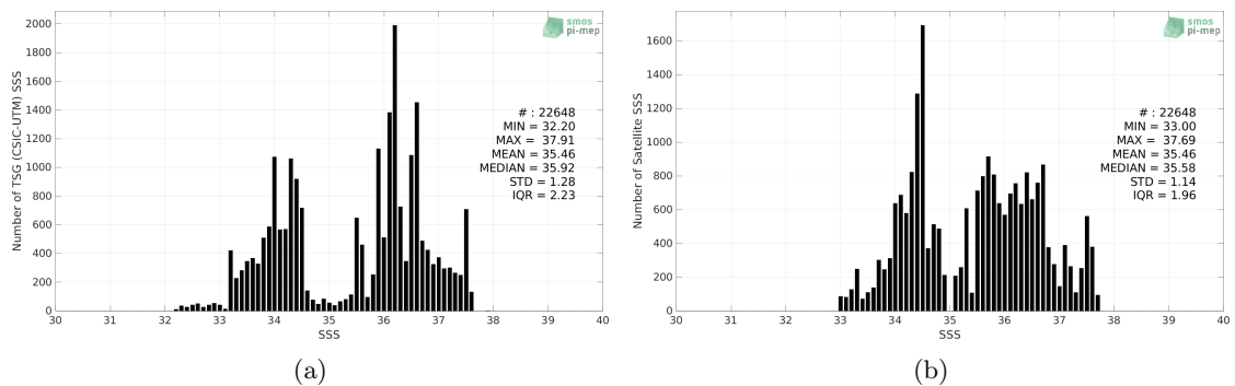
Figure 2: Histograms of SSS from TSG (CSIC-UTM) (a) and Aquarius SSS L2 OR v5 (NASA-GSFC) (b) considering all match-up pairs per bins of 0.1 over the South Atlantic Ocean Pi-MEP region and for the full satellite product period.
