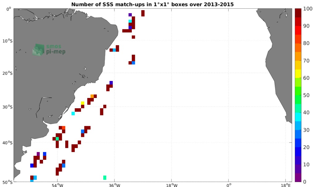
Figure 4: Number of SSS match-ups between TSG (CSIC-UTM) SSS and the Aquarius SSS L2 OR v5 (NASA-GSFC) SSS product for the South Atlantic Ocean Pi-MEP region over 1^\circ \times 1^\circ boxes and for the full satellite product period.
