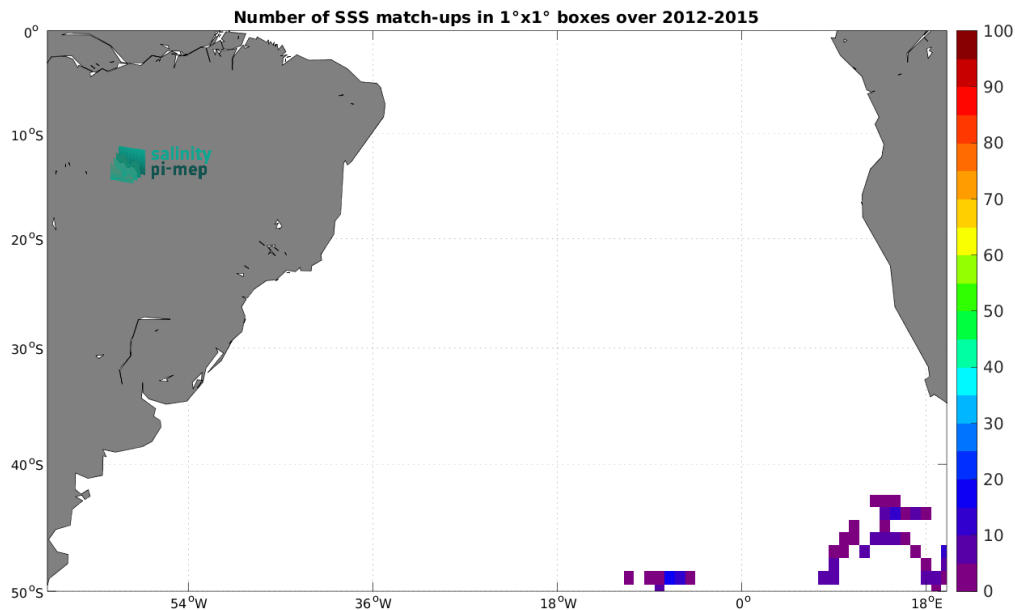
Figure 4: Number of SSS match-ups between Marine mammals SSS and the Aquarius SSS L2 OR v5 (NASA-GSFC) SSS product for the South Atlantic Ocean Pi-MEP region over 1^\circ \times 1^\circ boxes and for the full satellite product period.
