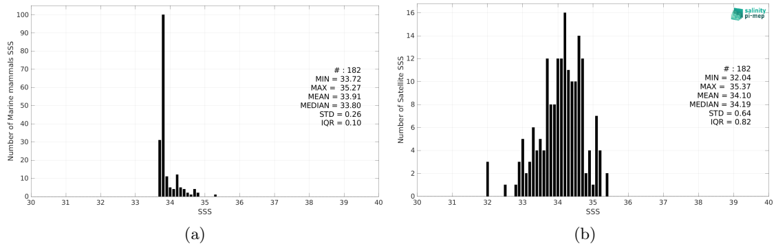
Figure 2: Histograms of SSS from Marine mammals (a) and Aquarius SSS L2 OR v5 (NASA-GSFC) (b) considering all match-up pairs per bins of 0.1 over the South Atlantic Ocean Pi-MEP region and for the full satellite product period.
