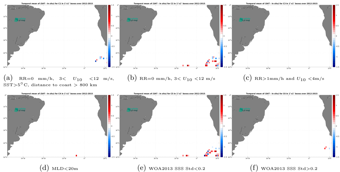
Figure 12: Temporal mean gridded over spatial boxes of size 1^{\circ}\times 1^{\circ} of \Delta\text{SSS} (Aquarius SSS L2 OR v5 (NASA-GSFC) - Marine mammals) for 6 different subdatasets corresponding to:RR=0 mm/h, 3 < U_{10} < 12 m/s, SST > 5^{\circ}\text{C} , distance to coast > 800 km (a), RR=0 mm/h, 3 < U_{10} < 12 m/s (b), RR > 1\text{mm/h} and U_{10} < 4\text{m/s} (c),MLD < 20\text{m} (d),WOA2013 SSS Std < 0.2 (e),WOA2013 SSS Std > 0.2 (f).
