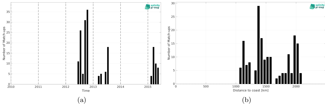
Figure 1: Number of match-ups between Marine mammals and Aquarius SSS L2 OR v5 (NASA-GSFC) SSS as a function of time (a) and as function of the distance to coast (b) over the South Atlantic Ocean Pi-MEP region and for the full satellite product period.
