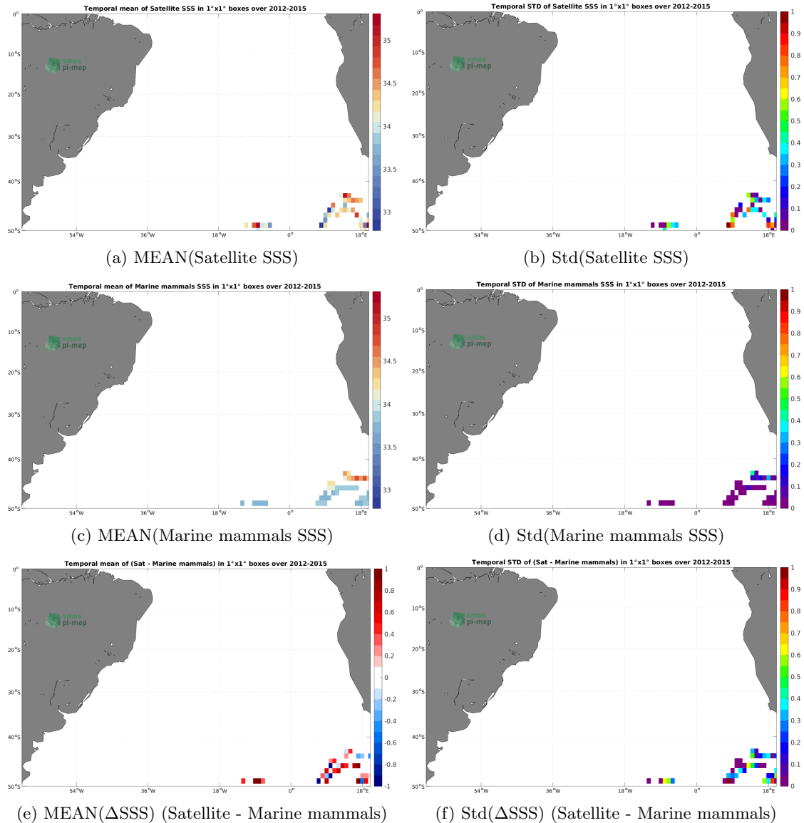
Figure 6: Temporal mean (left) and Std (right) of SSS from Aquarius SSS L2 OR v5 (NASA-GSFC) (top), Marine mammals (middle), and of \Delta SSS (Satellite - Marine mammals). Only match-up pairs are used to generate these maps.
