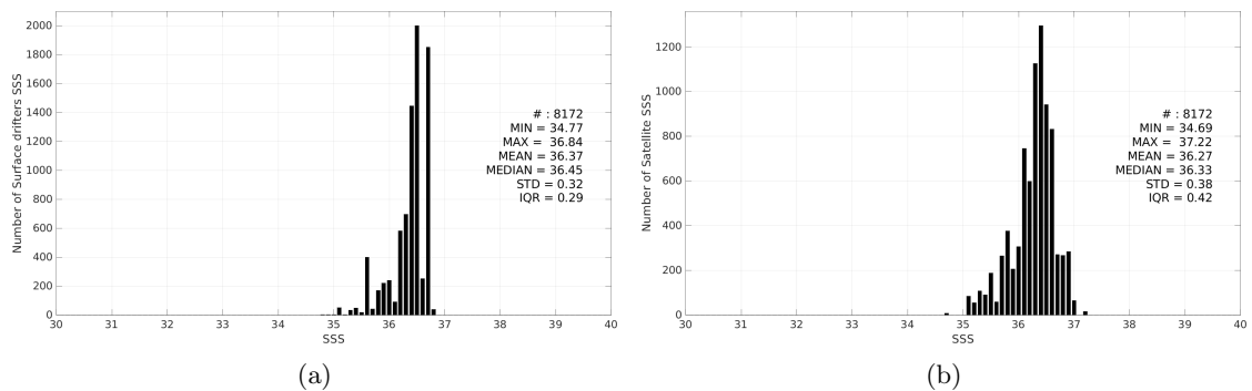
Figure 3: Histograms of SSS from Surface drifters (a) and Aquarius SSS L2 OR v5 (NASA-GSFC) (b) considering all match-up pairs per bins of 0.1 over the South Atlantic Ocean Pi-MEP region and for the full satellite product period.
