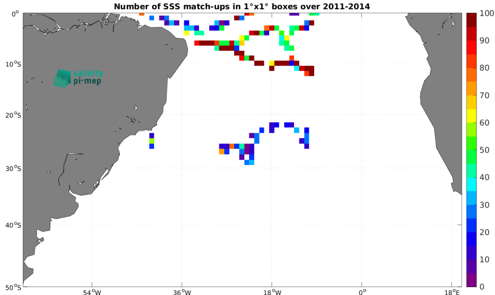
Figure 4: Number of SSS match-ups between Surface drifters SSS and the Aquarius SSS L2 OR v5 (NASA-GSFC) SSS product for the South Atlantic Ocean Pi-MEP region over 1^\circ \times 1^\circ boxes and for the full satellite product period.
