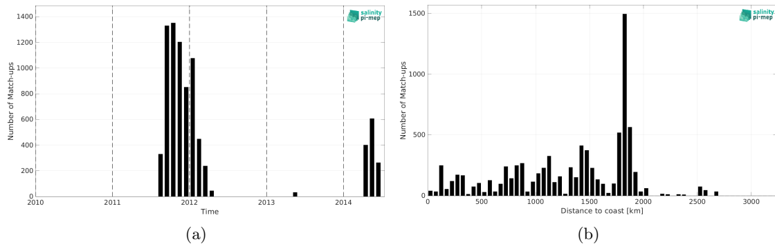
Figure 2: Number of match-ups between Surface drifters and Aquarius SSS L2 OR v5 (NASA-GSFC) SSS as a function of time (a) and as function of the distance to coast (b) over the South Atlantic Ocean Pi-MEP region and for the full satellite product period.
