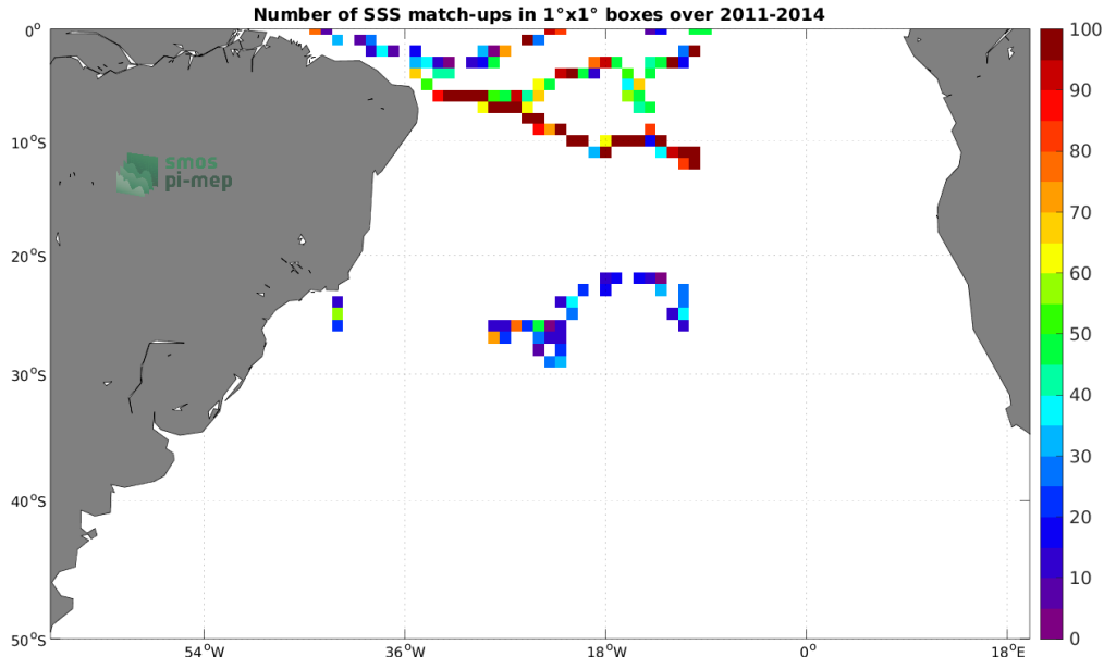
Figure 3: Number of SSS match-ups between Surface drifters SSS and the Aquarius SSS L2 OR v5 (NASA-GSFC) SSS product for the South Atlantic Ocean Pi-MEP region over 1^\circ \times 1^\circ boxes and for the full satellite product period.
