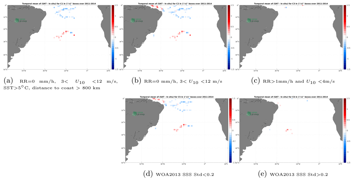
Figure 11: Temporal mean gridded over spatial boxes of size 1^\circ \times 1^\circ of \Delta SSS (Aquarius SSS L2 OR v5 (NASA-GSFC) - Surface drifters) for 5 different subdatasets corresponding to:RR=0 mm/h, 3 < U_{10} < 12 m/s, SST >5^\circ C, distance to coast > 800 km (a), RR=0 mm/h, 3 < U_{10} < 12 m/s (b), RR >1 mm/h and U_{10} < 4 m/s (c), WOA2013 SSS Std <0.2 (d), WOA2013 SSS Std >0.2 (e).
