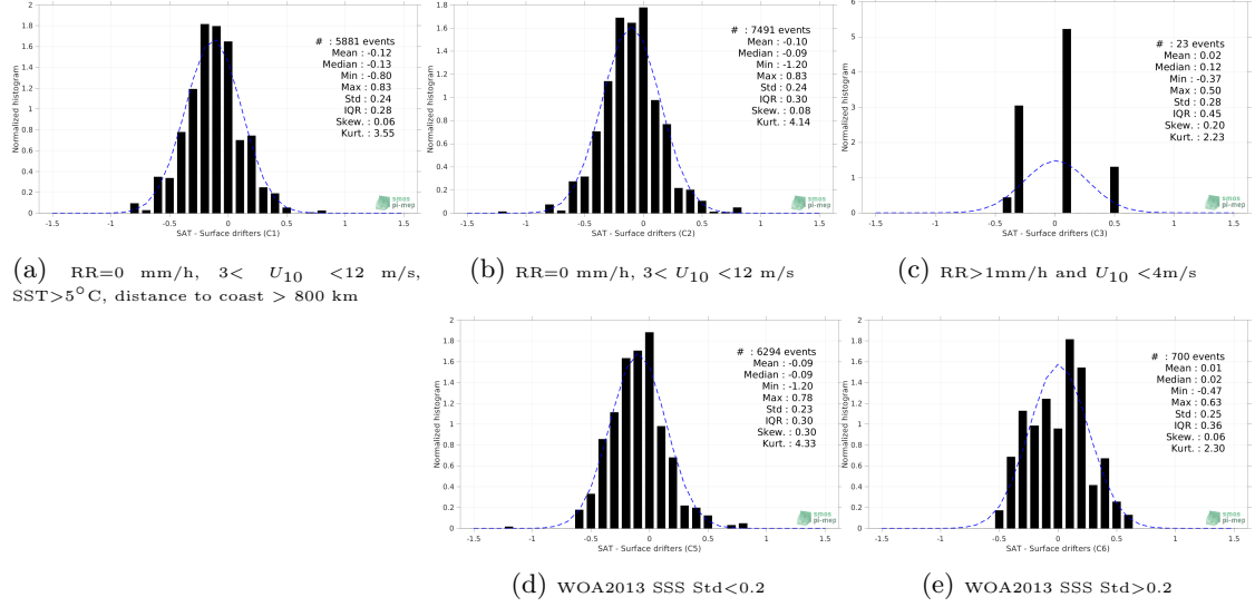
Figure 12: Normalized histogram of \Delta SSS (Aquarius SSS L2 OR v5 (NASA-GSFC) - Surface drifters) for 5 different subdatasets corresponding to: RR=0 mm/h, 3 < U_{10} < 12 m/s, SST > 5°C, distance to coast > 800 km (a), RR=0 mm/h, 3 < U_{10} < 12 m/s (b), RR > 1mm/h and U_{10} < 4 m/s (c), WOA2013 SSS Std < 0.2 (d), WOA2013 SSS Std > 0.2 (e).
