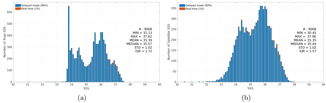
Figure 3: Histograms of SSS from Argo (a) and Aquarius SSS L2 OR v5 (NASA-GSFC) (b) considering all match-up pairs per bins of 0.1 over the South Atlantic Ocean Pi-MEP region and for the full satellite product period.
