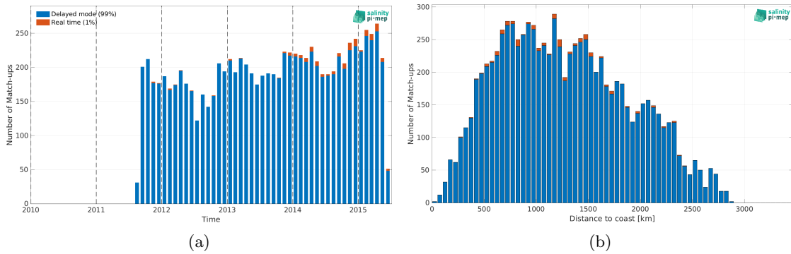
Figure 2: Number of match-ups between Argo and Aquarius SSS L2 OR v5 (NASA-GSFC) SSS as a function of time (a) and as function of the distance to coast (b) over the South Atlantic Ocean Pi-MEP region and for the full satellite product period.
