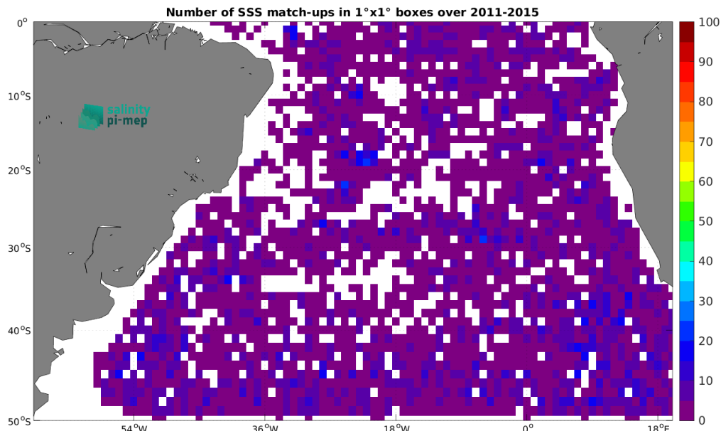
Figure 5: Number of SSS match-ups between Argo SSS and the Aquarius SSS L2 OR v5 (NASA-GSFC) SSS product for the South Atlantic Ocean Pi-MEP region over 1^\circ \times 1^\circ boxes and for the full satellite product period.
