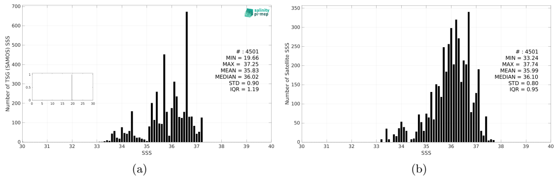
Figure 3: Histograms of SSS from TSG (SAMOS) (a) and Aquarius SSS L2 CAP v5 (JPL) (b) considering all match-up pairs per bins of 0.1 over the South Atlantic Ocean Pi-MEP region and for the full satellite product period.
