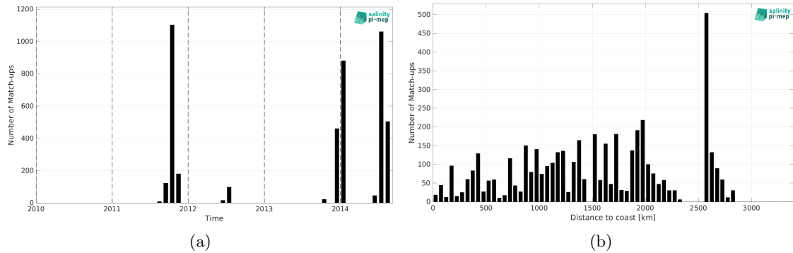
Figure 2: Number of match-ups between TSG (SAMOS) and Aquarius SSS L2 CAP v5 (JPL) SSS as a function of time (a) and as function of the distance to coast (b) over the South Atlantic Ocean Pi-MEP region and for the full satellite product period.
