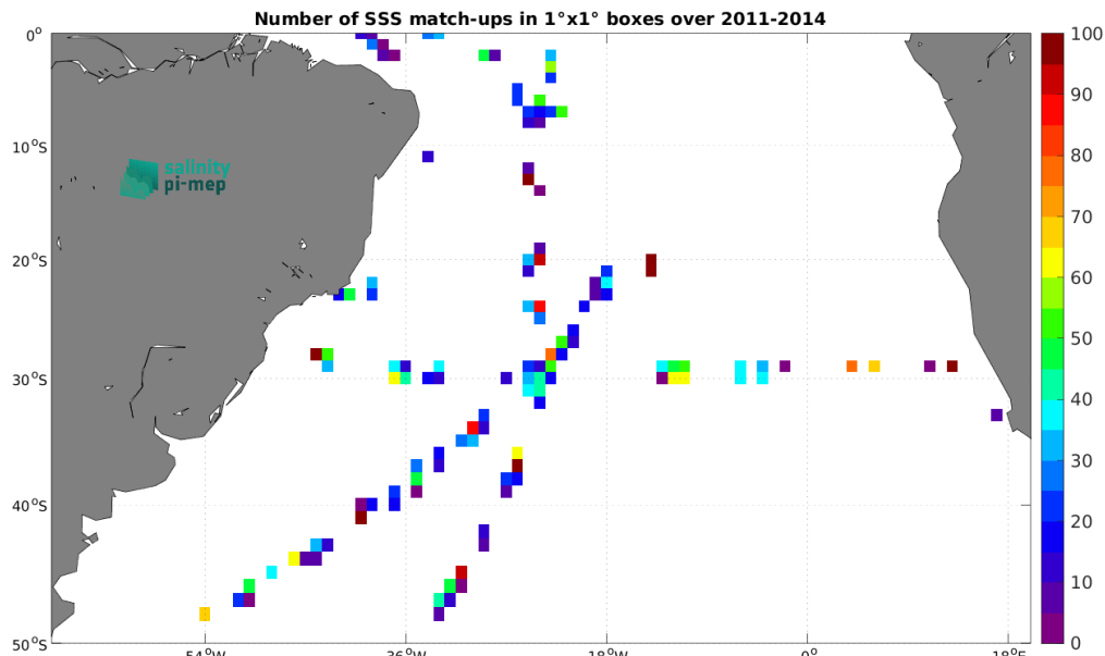
Figure 5: Number of SSS match-ups between TSG (SAMOS) SSS and the Aquarius SSS L2 CAP v5 (JPL) SSS product for the South Atlantic Ocean Pi-MEP region over 1^\circ \times 1^\circ boxes and for the full satellite product period.
