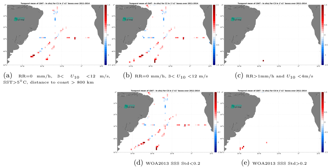
Figure 12: Temporal mean gridded over spatial boxes of size 1^\circ \times 1^\circ of \Delta\text{SSS} (Aquarius SSS L2 CAP v5 (JPL) - TSG (SAMOS)) for 5 different subdatasets corresponding to:RR=0 mm/h, 3 < U_{10} < 12 m/s, SST >5^\circ\text{C} , distance to coast > 800 km (a), RR=0 mm/h, 3 < U_{10} < 12 m/s (b), RR >1 mm/h and U_{10} < 4 m/s (c), WOA2013 SSS Std <0.2 (d), WOA2013 SSS Std >0.2 (e).
