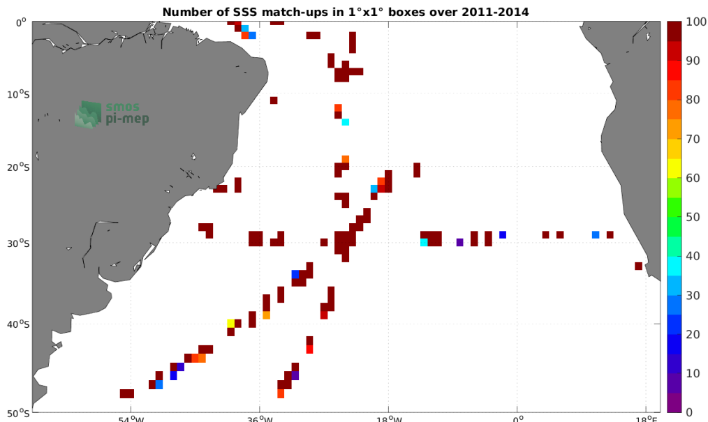
Figure 4: Number of SSS match-ups between TSG (SAMOS) SSS and the Aquarius SSS L2 CAP v5 (JPL) SSS product for the South Atlantic Ocean Pi-MEP region over 1^\circ \times 1^\circ boxes and for the full satellite product period.
