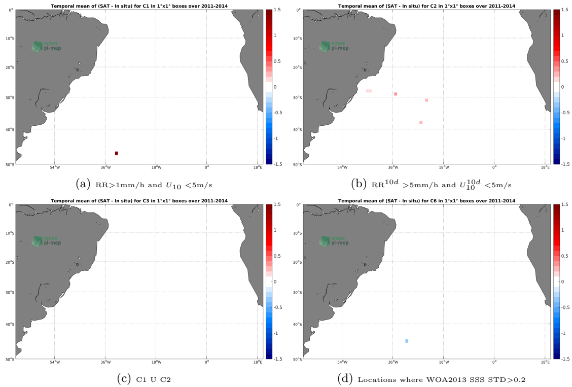
Figure 12: Temporal mean gridded over spatial boxes of size 1^\circ \times 1^\circ of \Delta SSS (Aquarius-L2-JPL-V5 - TSG-SAMOS) for 4 different subdatasets corresponding to: RR > 1mm/h and U_{10} < 5\text{m/s} (a), RR^{10d} > 5\text{mm/h} and U_{10}^{10d} < 5\text{m/s} (b), C1 U C2 (c), Locations where WOA2013 SSS STD > 0.2 (d).
