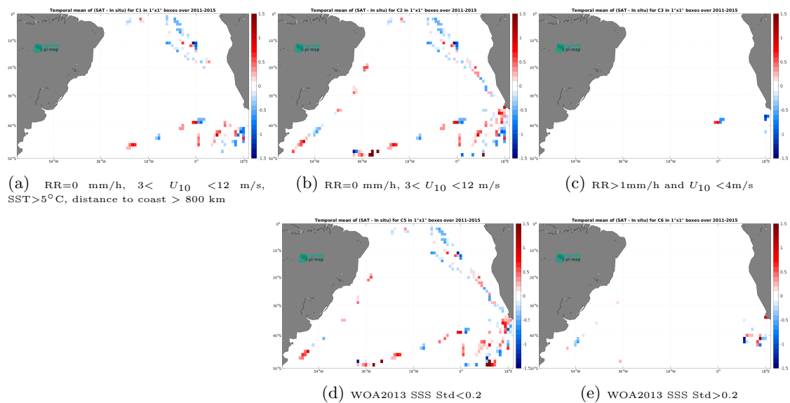
Figure 14: Temporal mean gridded over spatial boxes of size 1^\circ \times 1^\circ of \Delta\text{SSS} (Aquarius SSS L2 CAP v5 (JPL) - TSG (Polarstern)) for 5 different subdatasets corresponding to:RR=0 mm/h, 3 < U_{10} < 12 m/s, SST >5^\circ\text{C} , distance to coast > 800 km (a), RR=0 mm/h, 3 < U_{10} < 12 m/s (b), RR >1 mm/h and U_{10} < 4 m/s (c), WOA2013 SSS Std <0.2 (d), WOA2013 SSS Std >0.2 (e).
