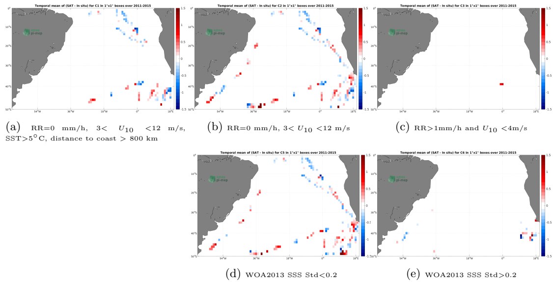
Figure 12: Temporal mean gridded over spatial boxes of size 1^\circ \times 1^\circ of \Delta\text{SSS} (Aquarius SSS L2 CAP v5 (JPL) - TSG (Polarstern)) for 5 different subdatasets corresponding to:RR=0 mm/h, 3 < U_{10} < 12 m/s, SST >5^\circ\text{C} , distance to coast > 800 km (a), RR=0 mm/h, 3 < U_{10} < 12 m/s (b), RR >1 mm/h and U_{10} < 4 m/s (c), WOA2013 SSS Std <0.2 (d), WOA2013 SSS Std >0.2 (e).
