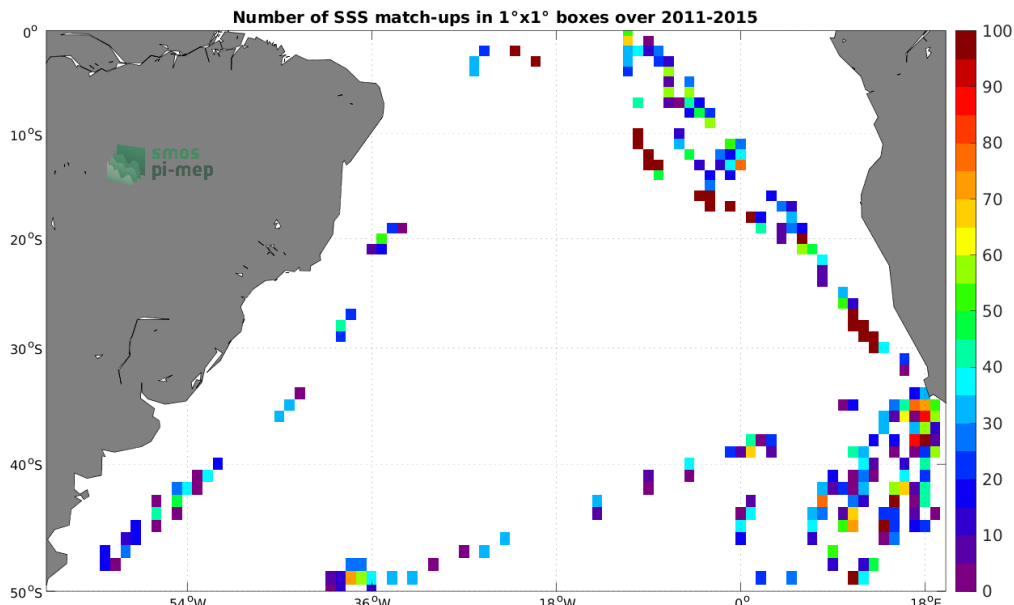
Figure 4: Number of SSS match-ups between TSG (Polarstern) SSS and the Aquarius SSS L2 CAP v5 (JPL) SSS product for the South Atlantic Ocean Pi-MEP region over 1^\circ \times 1^\circ boxes and for the full satellite product period.
