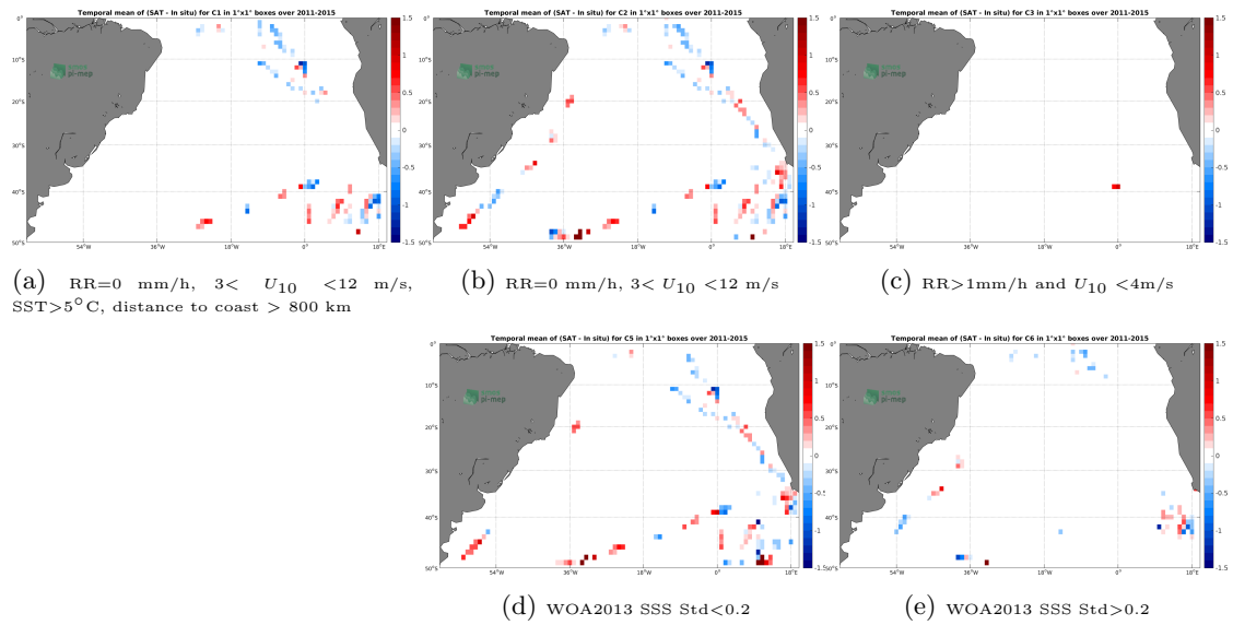
Figure 12: Temporal mean gridded over spatial boxes of size 1^\circ \times 1^\circ of \Delta SSS (Aquarius-L2-JPL-V5 - TSG-POLARSTERN) for 5 different subdatasets corresponding to:RR=0 mm/h, 3 < U_{10} < 12 m/s, SST >5^\circ\text{C} , distance to coast > 800 km (a), RR=0 mm/h, 3 < U_{10} < 12 m/s (b), RR >1 mm/h and U_{10} < 4 m/s (c), WOA2013 SSS Std <0.2 (d), WOA2013 SSS Std >0.2 (e).
