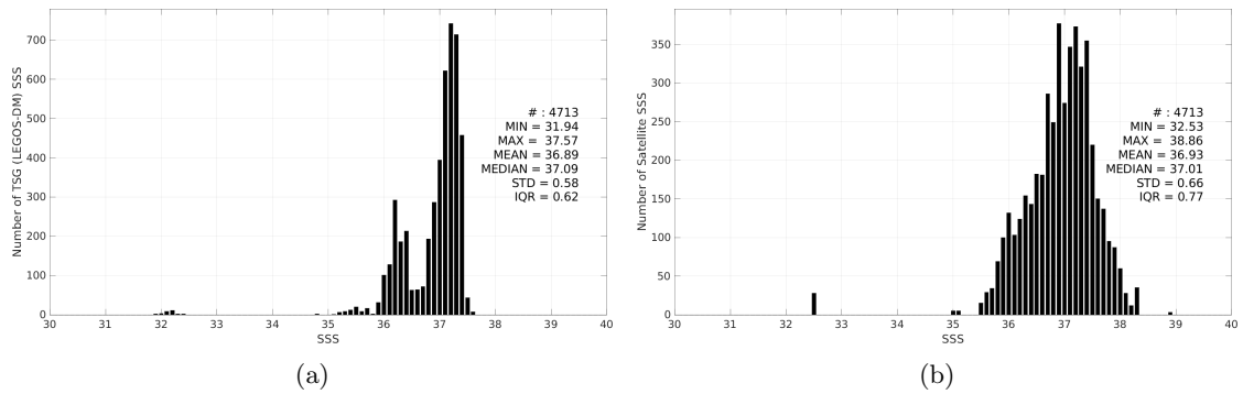
Figure 3: Histograms of SSS from TSG (LEGOS-DM) (a) and Aquarius SSS L2 CAP v5 (JPL) (b) considering all match-up pairs per bins of 0.1 over the South Atlantic Ocean Pi-MEP region and for the full satellite product period.
