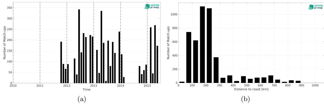
Figure 2: Number of match-ups between TSG (LEGOS-DM) and Aquarius SSS L2 CAP v5 (JPL) SSS as a function of time (a) and as function of the distance to coast (b) over the South Atlantic Ocean Pi-MEP region and for the full satellite product period.
