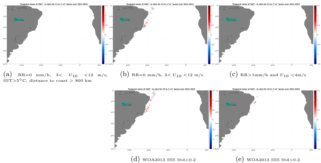
Figure 14: Temporal mean gridded over spatial boxes of size 1^\circ \times 1^\circ of \Delta SSS (Aquarius SSS L2 CAP v5 (JPL) - TSG (LEGOS-DM)) for 5 different subdatasets corresponding to:RR=0 mm/h, 3 < U_{10} < 12 m/s, SST >5^\circ\text{C} , distance to coast > 800 km (a), RR=0 mm/h, 3 < U_{10} < 12 m/s (b), RR >1 mm/h and U_{10} < 4 m/s (c), WOA2013 SSS Std <0.2 (d), WOA2013 SSS Std >0.2 (e).
