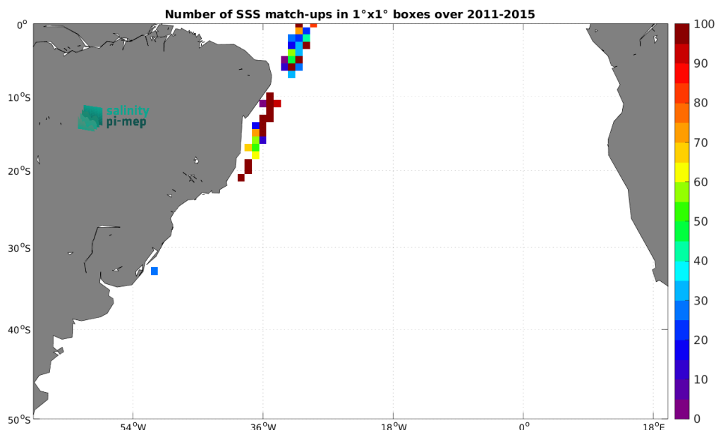
Figure 5: Number of SSS match-ups between TSG (LEGOS-DM) SSS and the Aquarius SSS L2 CAP v5 (JPL) SSS product for the South Atlantic Ocean Pi-MEP region over 1^\circ \times 1^\circ boxes and for the full satellite product period.
