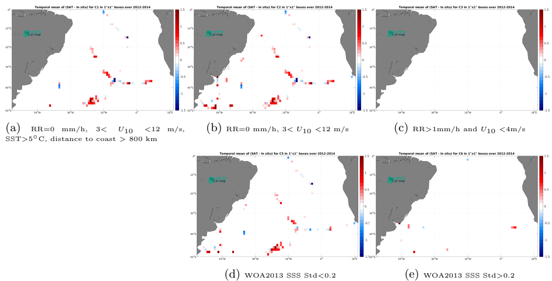
Figure 14: Temporal mean gridded over spatial boxes of size 1^\circ \times 1^\circ of \Delta\text{SSS} (Aquarius SSS L2 CAP v5 (JPL) - TSG (GOSUD-Sailing-ship)) for 5 different subdatasets corresponding to:RR=0 mm/h, 3 < U_{10} < 12 m/s, SST >5^\circ\text{C} , distance to coast > 800 km (a), RR=0 mm/h, 3 < U_{10} < 12 m/s (b), RR >1 mm/h and U_{10} < 4 m/s (c), WOA2013 SSS Std <0.2 (d), WOA2013 SSS Std >0.2 (e).
