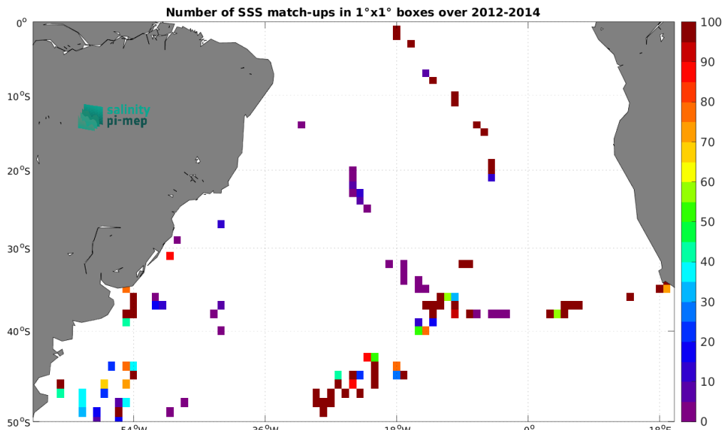
Figure 5: Number of SSS match-ups between TSG (GOSUD-Sailing-ship) SSS and the Aquarius SSS L2 CAP v5 (JPL) SSS product for the South Atlantic Ocean Pi-MEP region over 1^\circ \times 1^\circ boxes and for the full satellite product period.
