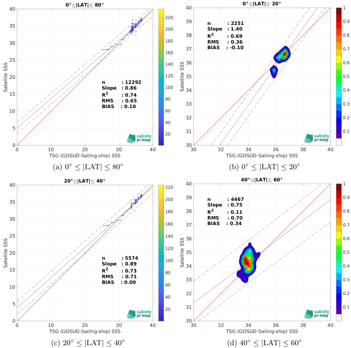
Figure 10: Contour maps of the concentration of Aquarius SSS L2 CAP v5 (JPL) SSS (y-axis) versus TSG (GOSUD-Sailing-ship) SSS (x-axis) at match-up pairs for different latitude bands. For each plot, the red line shows x=y . The black thin and dashed lines indicate a linear fit through the data cloud and the \pm 95\% confidence levels, respectively. The number match-up pairs n , the slope and R^2 coefficient of the linear fit, the root mean square (RMS) and the mean bias between satellite and in situ data are indicated for each latitude band in each plots.
