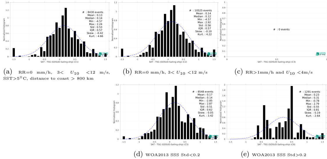
Figure 15: Normalized histogram of \Delta SSS (Aquarius SSS L2 CAP v5 (JPL) - TSG (GOSUD-Sailing-ship)) for 5 different subdatasets corresponding to: RR=0 mm/h, 3 < U_{10} < 12 m/s, SST > 5°C, distance to coast > 800 km (a), RR=0 mm/h, 3 < U_{10} < 12 m/s (b), RR > 1mm/h and U_{10} < 4 m/s (c), WOA2013 SSS Std < 0.2 (d), WOA2013 SSS Std > 0.2 (e).
