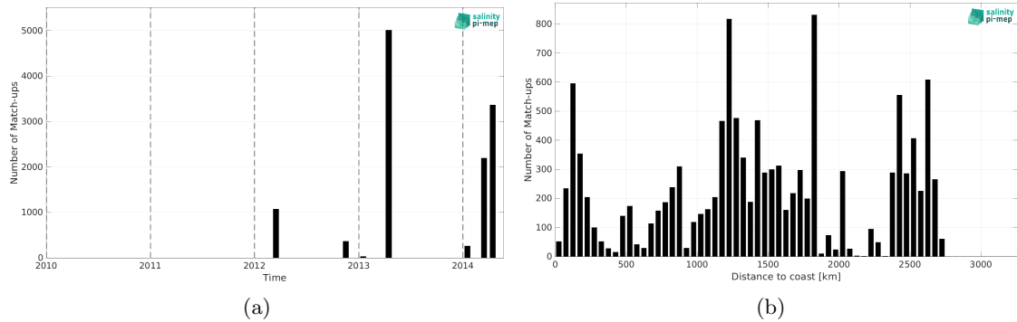
Figure 2: Number of match-ups between TSG (GOSUD-Sailing-ship) and Aquarius SSS L2 CAP v5 (JPL) SSS as a function of time (a) and as function of the distance to coast (b) over the South Atlantic Ocean Pi-MEP region and for the full satellite product period.
