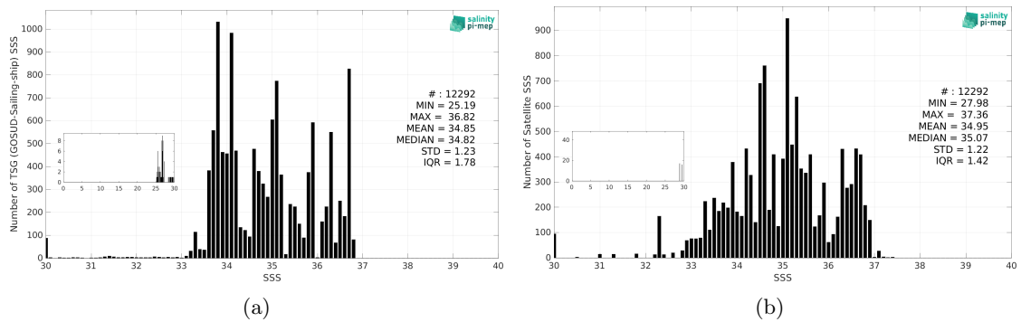
Figure 3: Histograms of SSS from TSG (GOSUD-Sailing-ship) (a) and Aquarius SSS L2 CAP v5 (JPL) (b) considering all match-up pairs per bins of 0.1 over the South Atlantic Ocean Pi-MEP region and for the full satellite product period.
