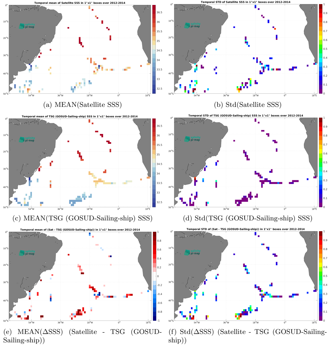
Figure 7: Temporal mean (left) and Std (right) of SSS from Aquarius SSS L2 CAP v5 (JPL) (top), TSG (GOSUD-Sailing-ship) (middle), and of \Delta SSS (Satellite - TSG (GOSUD-Sailing-ship)). Only match-up pairs are used to generate these maps.
