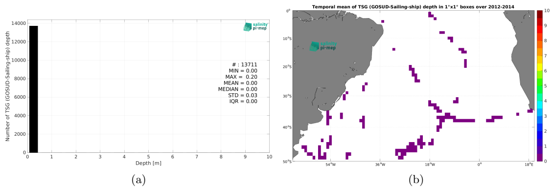
Figure 3: Histograms of the depth of the upper level SSS measurements from TSG (GOSUD-Sailing-ship) in the Match-up DataBase for the South Atlantic Ocean Pi-MEP region (a) and temporal mean spatial distribution of pressure of the in situ SSS data over 1^\circ \times 1^\circ boxes and for the full satellite product period (b).
