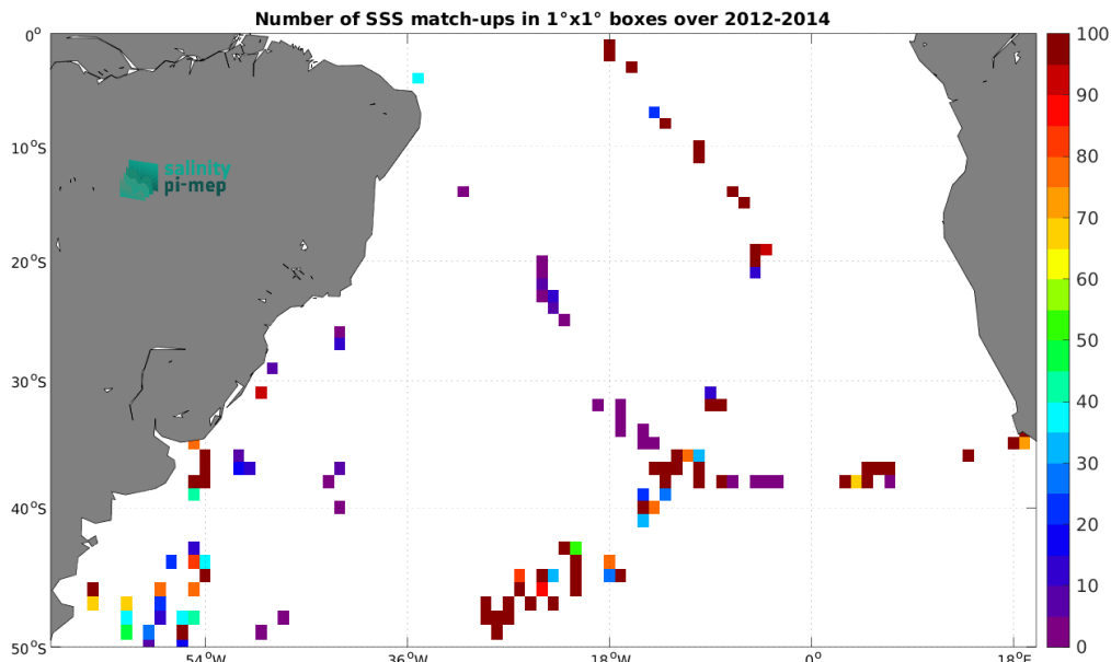
Figure 4: Number of SSS match-ups between TSG (GOSUD-Sailing-ship) SSS and the Aquarius SSS L2 CAP v5 (JPL) SSS product for the South Atlantic Ocean Pi-MEP region over 1^\circ \times 1^\circ boxes and for the full satellite product period.
