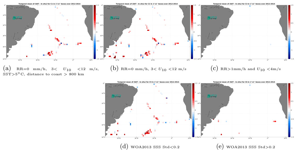
Figure 12: Temporal mean gridded over spatial boxes of size 1^\circ \times 1^\circ of \Delta\text{SSS} (Aquarius SSS L2 CAP v5 (JPL) - TSG (GOSUD-Sailing-ship)) for 5 different subdatasets corresponding to:RR=0 mm/h, 3 < U_{10} < 12 m/s, SST > 5^\circ\text{C} , distance to coast > 800 km (a), RR=0 mm/h, 3 < U_{10} < 12 m/s (b), RR > 1 mm/h and U_{10} < 4 m/s (c), WOA2013 SSS Std < 0.2 (d), WOA2013 SSS Std > 0.2 (e).
