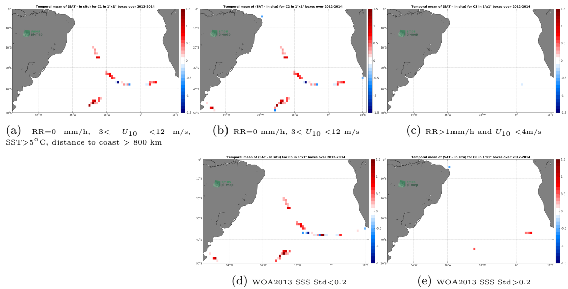
Figure 12: Temporal mean gridded over spatial boxes of size 1^\circ \times 1^\circ of \Delta SSS (Aquarius-L2-JPL-V5 - TSG-GOSUD-Sailing-ship) for 5 different subdatasets corresponding to: RR=0 mm/h, 3 < U_{10} < 12 m/s, SST > 5^\circ C , distance to coast > 800 km (a), RR=0 mm/h, 3 < U_{10} < 12 m/s (b), RR > 1 mm/h and U_{10} < 4 m/s (c), WOA2013 SSS Std < 0.2 (d), WOA2013 SSS Std > 0.2 (e).
