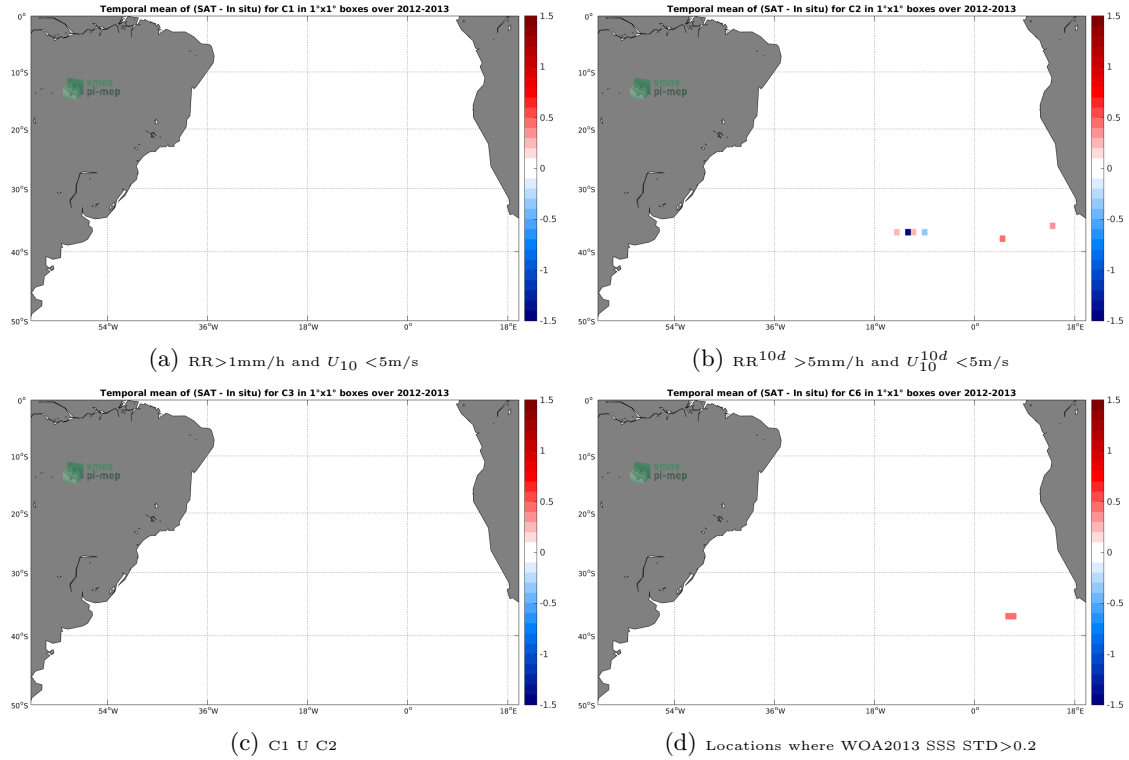
Figure 12: Temporal mean gridded over spatial boxes of size 1^\circ \times 1^\circ of \Delta SSS (Aquarius-L2-JPL-V5 - TSG-GOSUD-Sailing-ship) for 4 different subdatasets corresponding to: RR > 1\text{mm/h} and U_{10} < 5\text{m/s} (a), RR^{10d} > 5\text{mm/h} and U_{10}^{10d} < 5\text{m/s} (b), C1 U C2 (c), Locations where WOA2013 SSS STD > 0.2 (d).
