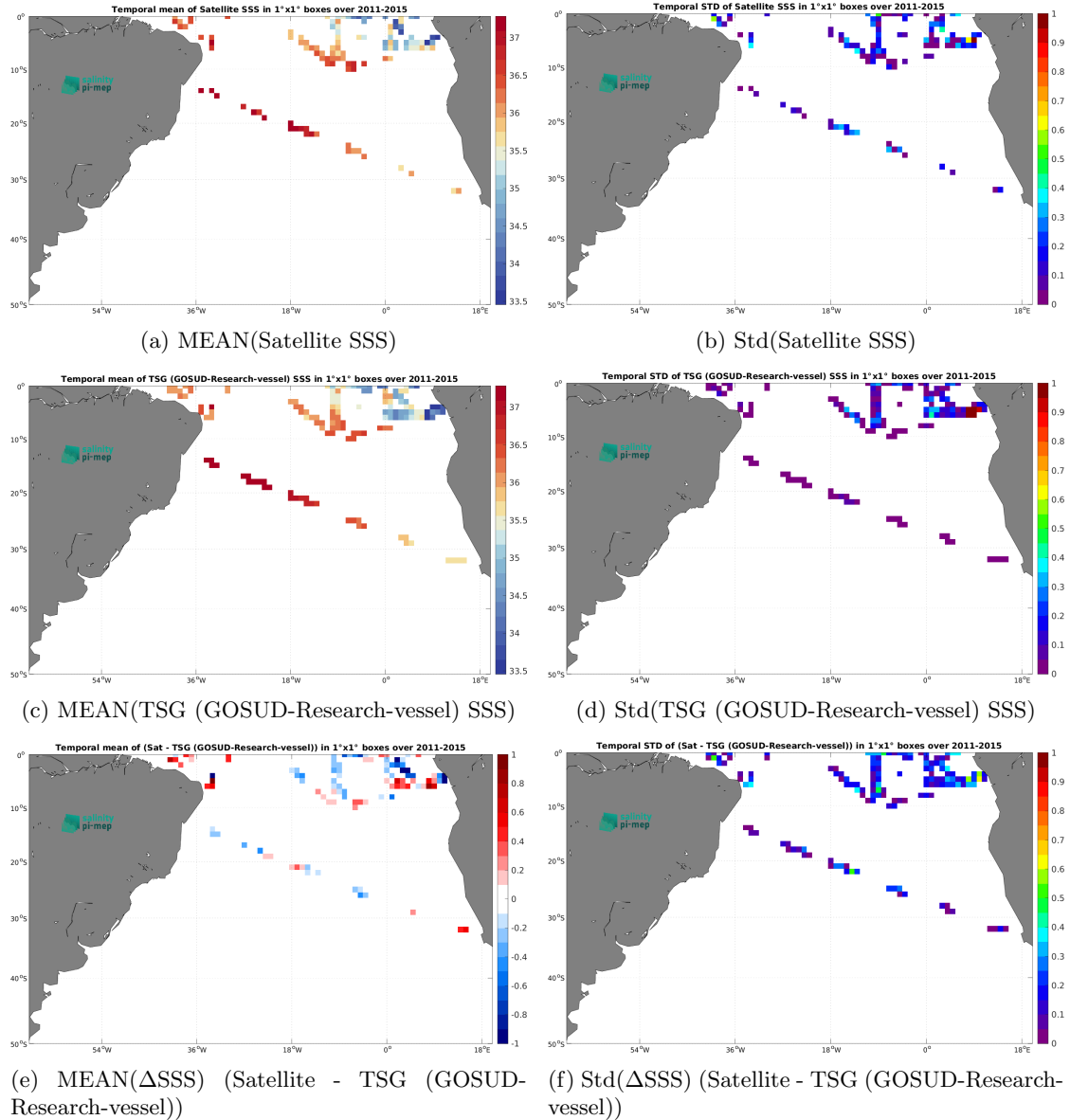
Figure 7: Temporal mean (left) and Std (right) of SSS from Aquarius SSS L2 CAP v5 (JPL) (top), TSG (GOSUD-Research-vessel) (middle), and of \Delta SSS (Satellite - TSG (GOSUD-Research-vessel)). Only match-up pairs are used to generate these maps.
