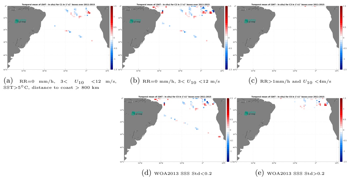
Figure 14: Temporal mean gridded over spatial boxes of size 1^\circ \times 1^\circ of \Delta SSS (Aquarius SSS L2 CAP v5 (JPL) - TSG (GOSUD-Research-vessel)) for 5 different subdatasets corresponding to:RR=0 mm/h, 3 < U_{10} < 12 m/s, SST >5^\circ\text{C} , distance to coast > 800 km (a), RR=0 mm/h, 3 < U_{10} < 12 m/s (b), RR >1 mm/h and U_{10} < 4 m/s (c), WOA2013 SSS Std <0.2 (d), WOA2013 SSS Std >0.2 (e).
