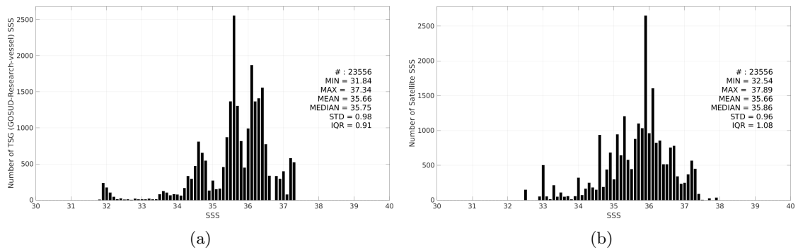
Figure 3: Histograms of SSS from TSG (GOSUD-Research-vessel) (a) and Aquarius SSS L2 CAP v5 (JPL) (b) considering all match-up pairs per bins of 0.1 over the South Atlantic Ocean Pi-MEP region and for the full satellite product period.
