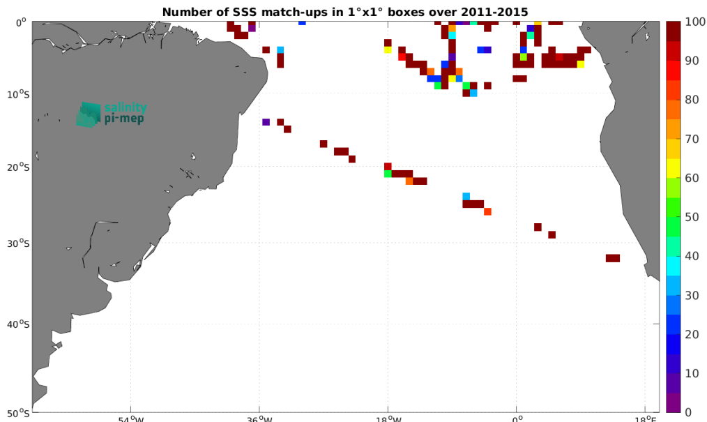
Figure 5: Number of SSS match-ups between TSG (GOSUD-Research-vessel) SSS and the Aquarius SSS L2 CAP v5 (JPL) SSS product for the South Atlantic Ocean Pi-MEP region over 1^\circ \times 1^\circ boxes and for the full satellite product period.
