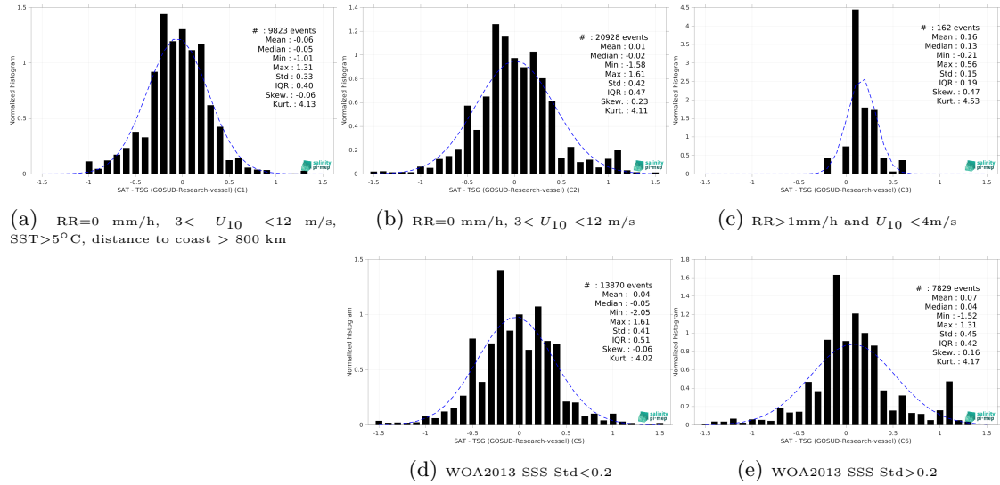
Figure 15: Normalized histogram of \Delta SSS (Aquarius SSS L2 CAP v5 (JPL) - TSG (GOSUD-Research-vessel)) for 5 different subdatasets corresponding to: RR=0 mm/h, 3 < U_{10} < 12 m/s, SST>5°C, distance to coast > 800 km (a), RR=0 mm/h, 3 < U_{10} < 12 m/s (b), RR>1mm/h and U_{10} < 4 m/s (c), WOA2013 SSS Std<0.2 (d), WOA2013 SSS Std>0.2 (e).
