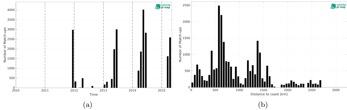
Figure 2: Number of match-ups between TSG (GOSUD-Research-vessel) and Aquarius SSS L2 CAP v5 (JPL) SSS as a function of time (a) and as function of the distance to coast (b) over the South Atlantic Ocean Pi-MEP region and for the full satellite product period.
