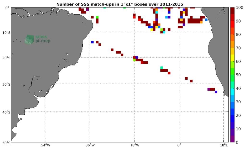
Figure 4: Number of SSS match-ups between TSG (GOSUD-Research-vessel) SSS and the Aquarius SSS L2 CAP v5 (JPL) SSS product for the South Atlantic Ocean Pi-MEP region over 1^\circ \times 1^\circ boxes and for the full satellite product period.
