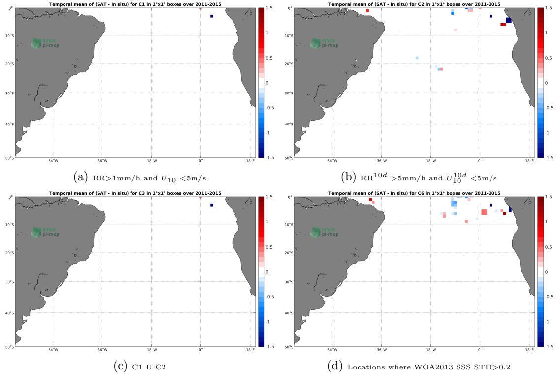
Figure 12: Temporal mean gridded over spatial boxes of size 1^\circ \times 1^\circ of \Delta SSS (Aquarius-L2-JPL-V5 - TSG-GOSUD-Research-vessel) for 4 different subdatasets corresponding to: RR > 1\text{mm/h} and U_{10} < 5\text{m/s} (a), RR^{10d} > 5\text{mm/h} and U_{10}^{10d} < 5\text{m/s} (b), C1 U C2 (c), Locations where WOA2013 SSS STD > 0.2 (d).
