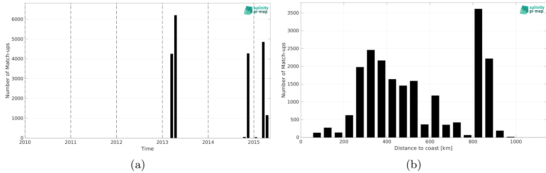
Figure 2: Number of match-ups between TSG (CSIC-UTM) and Aquarius SSS L2 CAP v5 (JPL) SSS as a function of time (a) and as function of the distance to coast (b) over the South Atlantic Ocean Pi-MEP region and for the full satellite product period.
