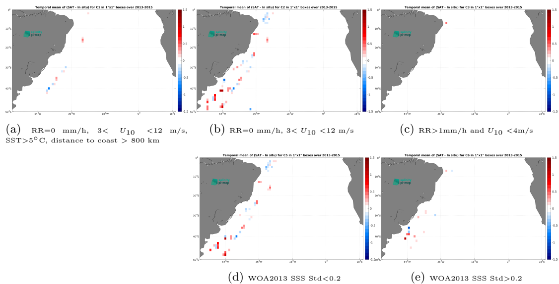
Figure 14: Temporal mean gridded over spatial boxes of size 1^\circ \times 1^\circ of \Delta\text{SSS} (Aquarius SSS L2 CAP v5 (JPL) - TSG (CSIC-UTM)) for 5 different subdatasets corresponding to:RR=0 mm/h, 3 < U_{10} < 12 m/s, SST >5^\circ\text{C} , distance to coast > 800 km (a), RR=0 mm/h, 3 < U_{10} < 12 m/s (b), RR >1 mm/h and U_{10} < 4 m/s (c), WOA2013 SSS Std <0.2 (d), WOA2013 SSS Std >0.2 (e).
