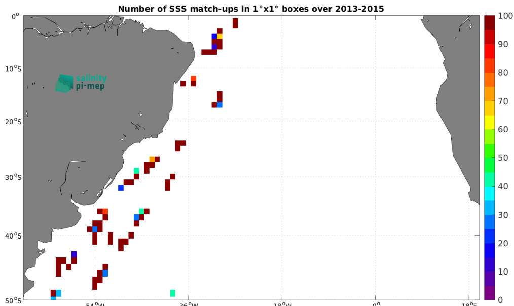
Figure 5: Number of SSS match-ups between TSG (CSIC-UTM) SSS and the Aquarius SSS L2 CAP v5 (JPL) SSS product for the South Atlantic Ocean Pi-MEP region over 1^\circ \times 1^\circ boxes and for the full satellite product period.
