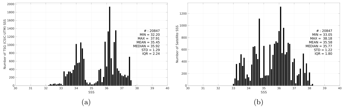
Figure 3: Histograms of SSS from TSG (CSIC-UTM) (a) and Aquarius SSS L2 CAP v5 (JPL) (b) considering all match-up pairs per bins of 0.1 over the South Atlantic Ocean Pi-MEP region and for the full satellite product period.
