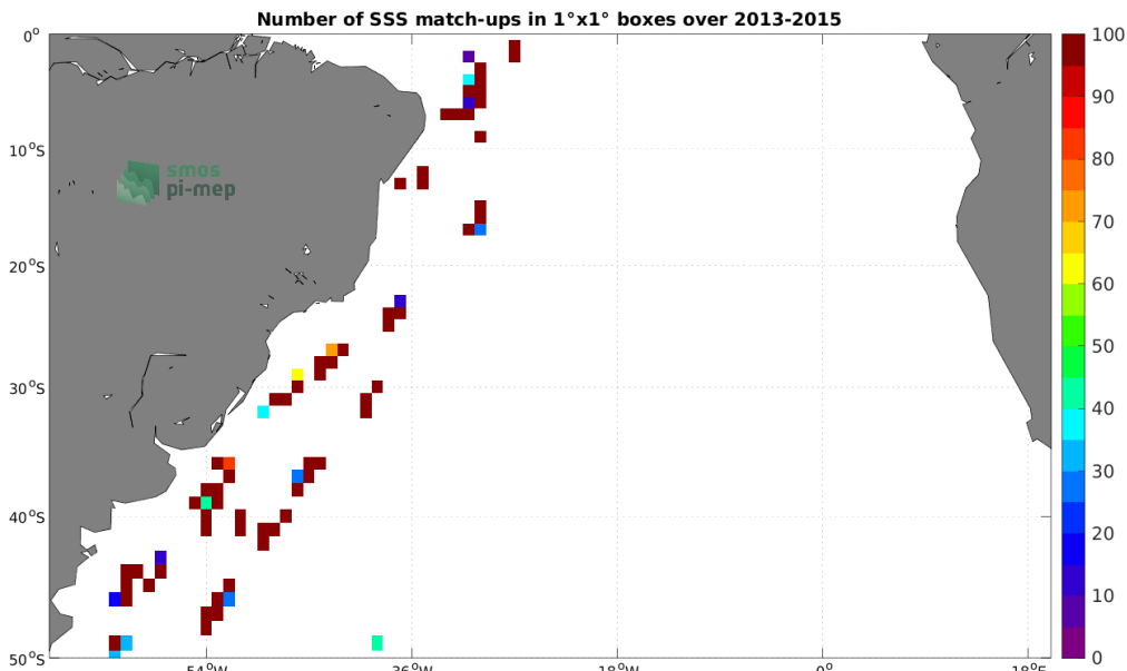
Figure 4: Number of SSS match-ups between TSG (CSIC-UTM) SSS and the Aquarius SSS L2 CAP v5 (JPL) SSS product for the South Atlantic Ocean Pi-MEP region over 1^\circ \times 1^\circ boxes and for the full satellite product period.
