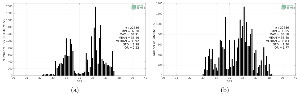
Figure 2: Histograms of SSS from TSG (CSIC-UTM) (a) and Aquarius SSS L2 CAP v5 (JPL) (b) considering all match-up pairs per bins of 0.1 over the South Atlantic Ocean Pi-MEP region and for the full satellite product period.
