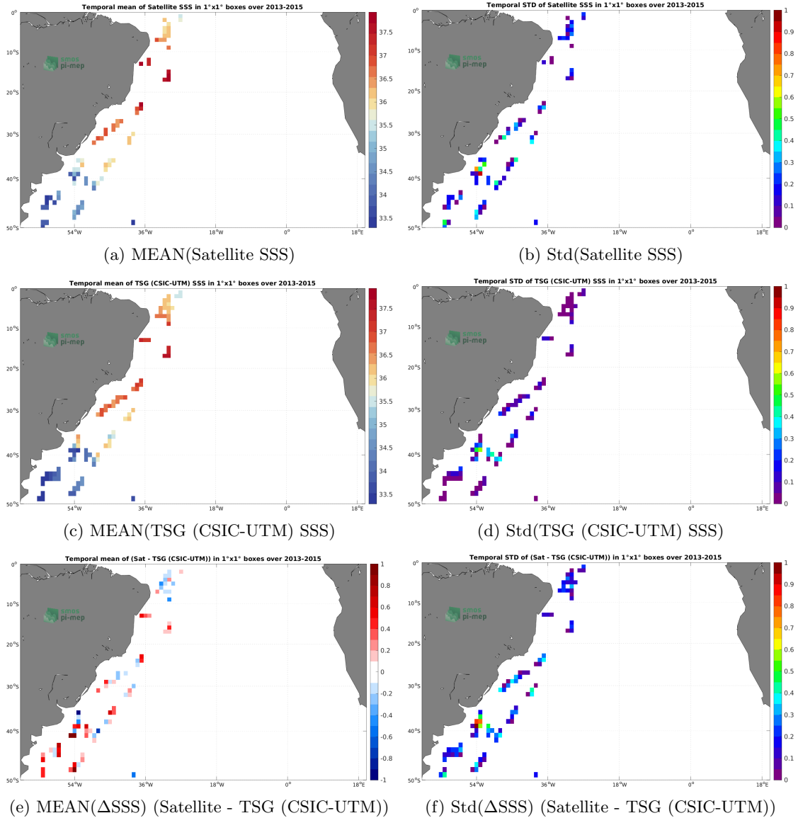
Figure 6: Temporal mean (left) and Std (right) of SSS from Aquarius SSS L2 CAP v5 (JPL) (top), TSG (CSIC-UTM) (middle), and of \Delta SSS (Satellite - TSG (CSIC-UTM)). Only match-up pairs are used to generate these maps.
