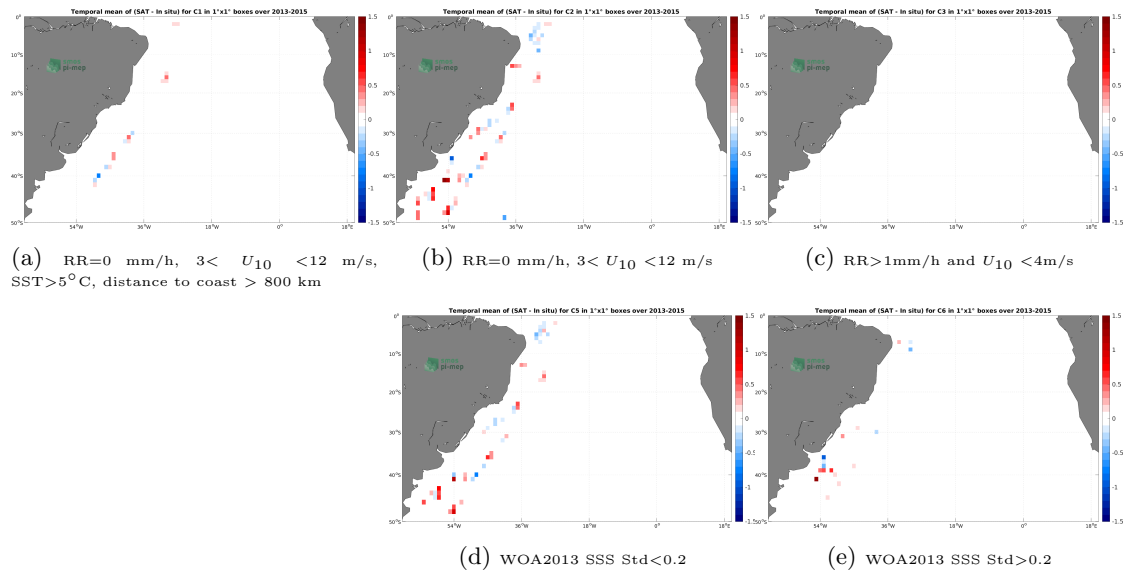
Figure 12: Temporal mean gridded over spatial boxes of size 1^\circ \times 1^\circ of \Delta SSS (Aquarius SSS L2 CAP v5 (JPL) - TSG (CSIC-UTM)) for 5 different subdatasets corresponding to:RR=0 mm/h, 3 < U_{10} < 12 m/s, SST >5^\circ\text{C} , distance to coast > 800 km (a), RR=0 mm/h, 3 < U_{10} < 12 m/s (b), RR >1 mm/h and U_{10} < 4 m/s (c), WOA2013 SSS Std <0.2 (d), WOA2013 SSS Std >0.2 (e).
