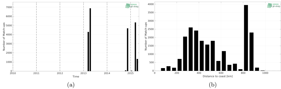
Figure 1: Number of match-ups between TSG (CSIC-UTM) and Aquarius SSS L2 CAP v5 (JPL) SSS as a function of time (a) and as function of the distance to coast (b) over the South Atlantic Ocean Pi-MEP region and for the full satellite product period.
