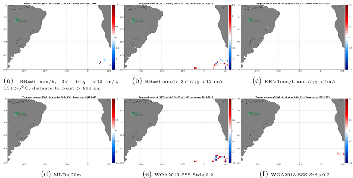
Figure 12: Temporal mean gridded over spatial boxes of size 1^{\circ}\times 1^{\circ} of \Delta\text{SSS} (Aquarius-L2-JPL-V5 - Sea mammals) for 6 different subdatasets corresponding to:RR=0 mm/h, 3 < U_{10} < 12 m/s, SST >5^{\circ}\text{C} , distance to coast > 800 km (a), RR=0 mm/h, 3 < U_{10} < 12 m/s (b), RR >1 mm/h and U_{10} < 4 m/s (c),MLD <20 m (d),WOA2013 SSS Std <0.2 (e),WOA2013 SSS Std >0.2 (f).
