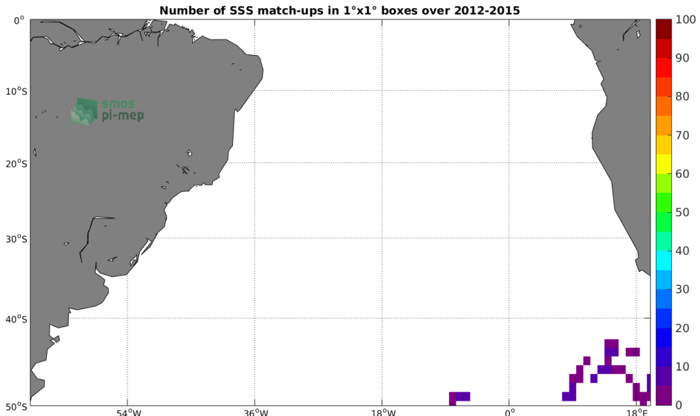
Figure 4: Number of SSS match-ups between Sea mammals SSS and the Aquarius-L2-JPL-V5 SSS product for the South Atlantic Ocean Pi-MEP region over 1°x1° boxes and for the full satellite product period.
