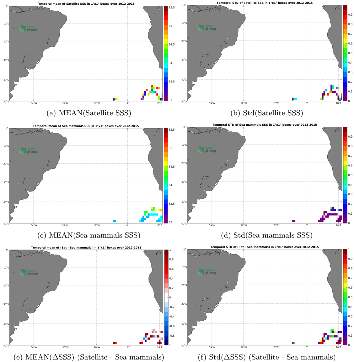
Figure 6: Temporal mean (left) and Std (right) of SSS from Aquarius-L2-JPL-V5 (top), Sea mammals (middle), and of \Delta SSS (Satellite - Sea mammals). Only match-up pairs are used to generate these maps.
