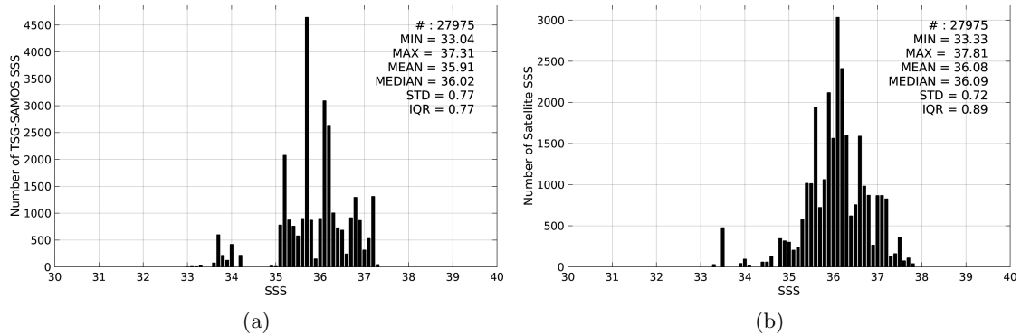
Figure 2: Histograms of SSS from TSG-SAMOS (a) and AQUARIUS-L2-JPL-V4 (b) considering all match-up pairs per bins of 0.1 over the South Atlantic Ocean Pi-MEP region and for the full satellite product period.
