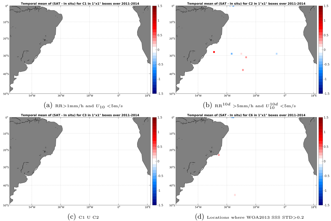
Figure 12: Temporal mean gridded over spatial boxes of size 1^\circ \times 1^\circ of \Delta SSS (AQUARIUS-L2-JPL-V4 - TSG-SAMOS) for 4 different subdatasets corresponding to: RR > 1\text{mm/h} and U_{10} < 5\text{m/s} (a), RR^{10d} > 5\text{mm/h} and U_{10}^{10d} < 5\text{m/s} (b), C1 U C2 (c), Locations where WOA2013 SSS STD > 0.2 (d).
