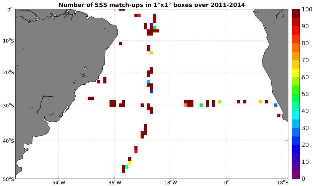
Figure 4: Number of SSS match-ups between TSG-SAMOS SSS and the AQUARIUS-L2-JPL-V4 SSS product for the South Atlantic Ocean Pi-MEP region over 1°x1° boxes and for the full satellite product period.
