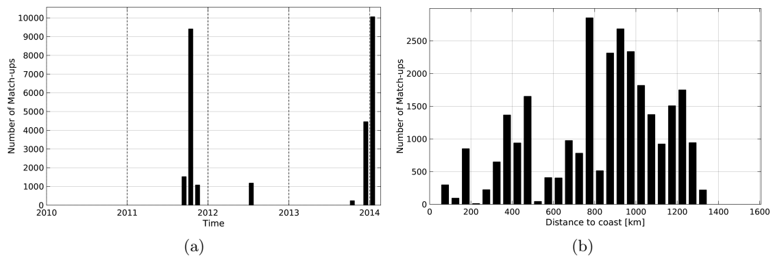
Figure 1: Number of match-ups between TSG-SAMOS and AQUARIUS-L2-JPL-V4 SSS as a function of time (a) and as function of the distance to coast (b) over the South Atlantic Ocean Pi-MEP region and for the full satellite product period.
