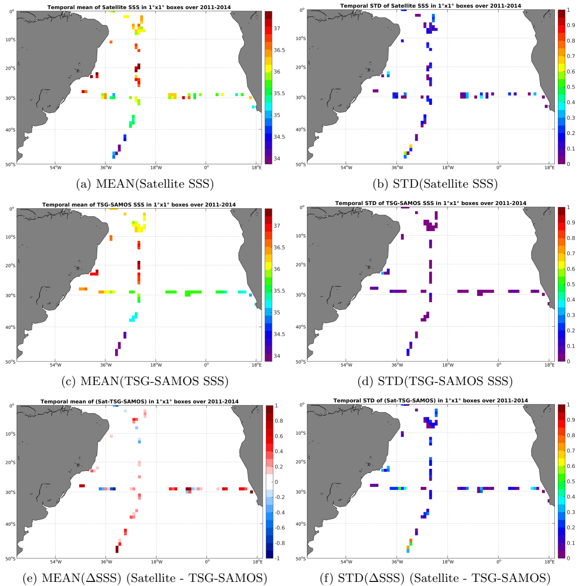
Figure 6: Temporal mean (left) and STD (right) of SSS from AQUARIUS-L2-JPL-V4 (top), TSG-SAMOS (middle), and of \Delta SSS (Satellite - TSG-SAMOS). Only match-up pairs are used to generate these maps.
