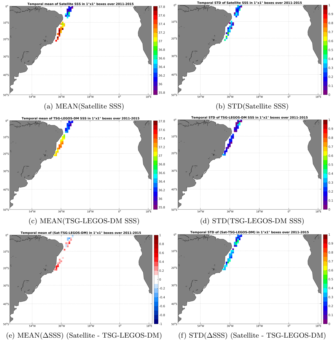
Figure 6: Temporal mean (left) and STD (right) of SSS from AQUARIUS-L2-JPL-V4 (top), TSG-LEGOS-DM (middle), and of \Delta SSS (Satellite - TSG-LEGOS-DM). Only match-up pairs are used to generate these maps.
