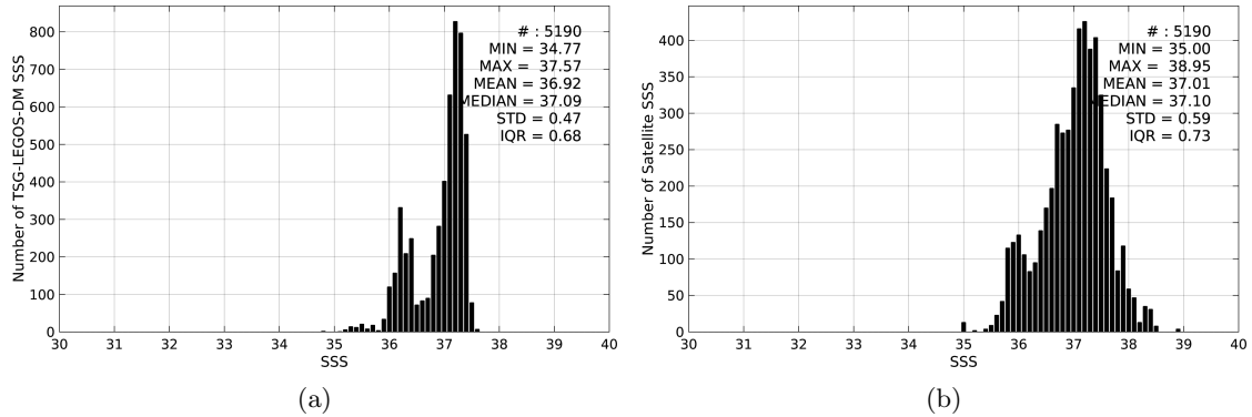
Figure 2: Histograms of SSS from TSG-LEGOS-DM (a) and AQUARIUS-L2-JPL-V4 (b) considering all match-up pairs per bins of 0.1 over the South Atlantic Ocean Pi-MEP region and for the full satellite product period.
