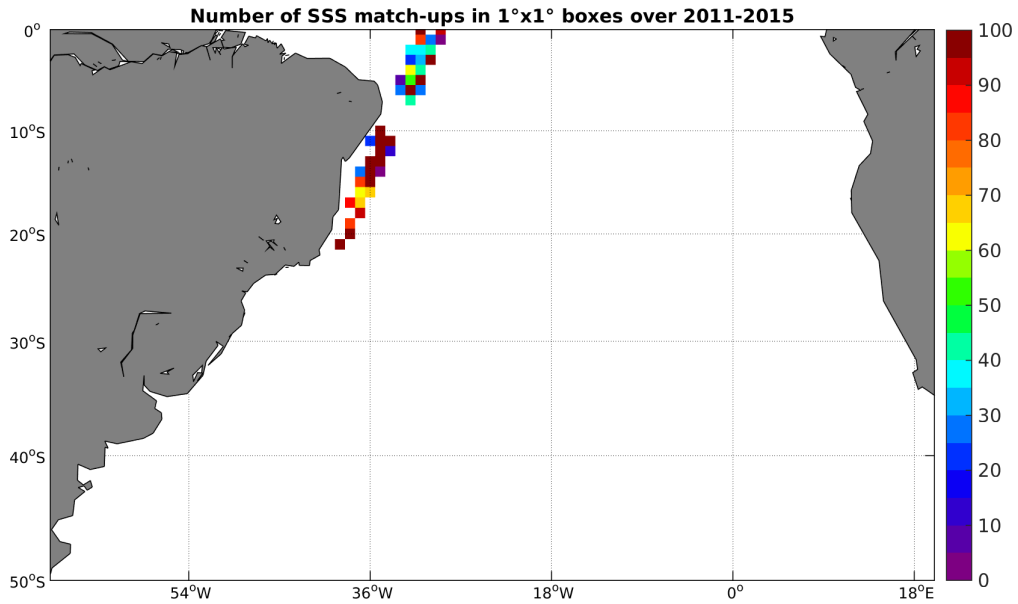
Figure 4: Number of SSS match-ups between TSG-LEGOS-DM SSS and the AQUARIUS-L2-JPL-V4 SSS product for the South Atlantic Ocean Pi-MEP region over 1^\circ \times 1^\circ boxes and for the full satellite product period.
