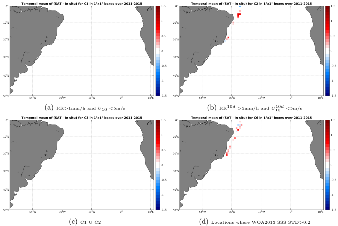
Figure 12: Temporal mean gridded over spatial boxes of size 1^\circ \times 1^\circ of \Delta SSS (AQUARIUS-L2-JPL-V4 - TSG-LEGOS-DM) for 4 different subdatasets corresponding to: RR > 1mm/h and U_{10} < 5\text{m/s} (a), RR^{10d} > 5\text{mm/h} and U_{10}^{10d} < 5\text{m/s} (b), C1 U C2 (c), Locations where WOA2013 SSS STD > 0.2 (d).
