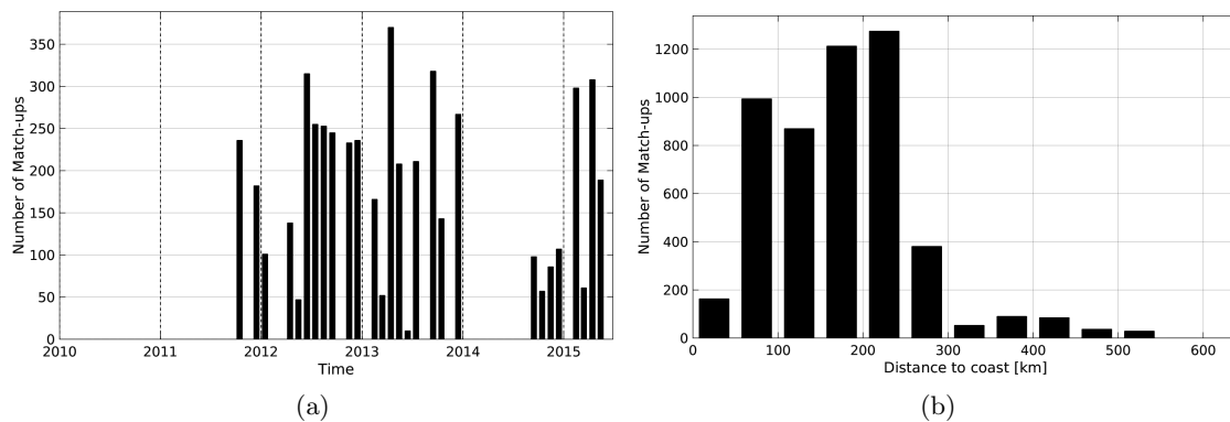
Figure 1: Number of match-ups between TSG-LEGOS-DM and AQUARIUS-L2-JPL-V4 SSS as a function of time (a) and as function of the distance to coast (b) over the South Atlantic Ocean Pi-MEP region and for the full satellite product period.
