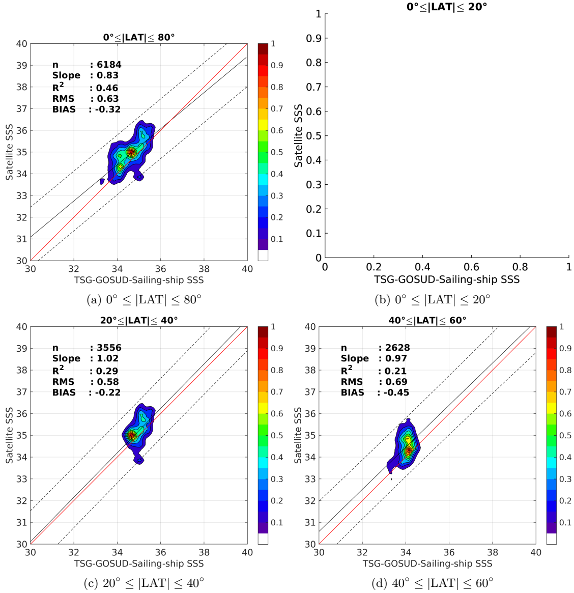
Figure 9: Contour maps of the concentration of AQUARIUS-L2-JPL-V4 SSS (y-axis) versus TSG-GOSUD-Sailing-ship SSS (x-axis) at match-up pairs for different latitude bands. For each plot, the red line shows x=y . The black thin and dashed lines indicate a linear fit through the data cloud and the \pm 95\% confidence levels, respectively. The number match-up pairs n , the slope and R^2 coefficient of the linear fit, the root mean square (RMS) and the mean bias between satellite and in situ data are indicated for each latitude band in each plots.
