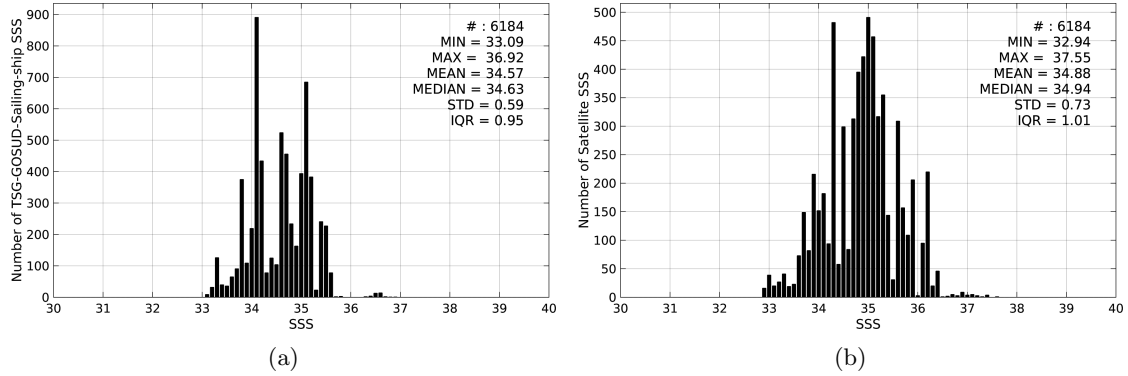
Figure 2: Histograms of SSS from TSG-GOSUD-Sailing-ship (a) and AQUARIUS-L2-JPL-V4 (b) considering all match-up pairs per bins of 0.1 over the South Atlantic Ocean Pi-MEP region and for the full satellite product period.
