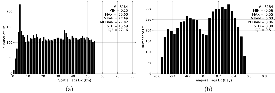
Figure 5: Histograms of the spatial (a) and temporal (b) lags between the time of the TSG-GOSUD-Sailing-ship measurements and the date of the corresponding AQUARIUS-L2-JPL-V4 SSS product.
