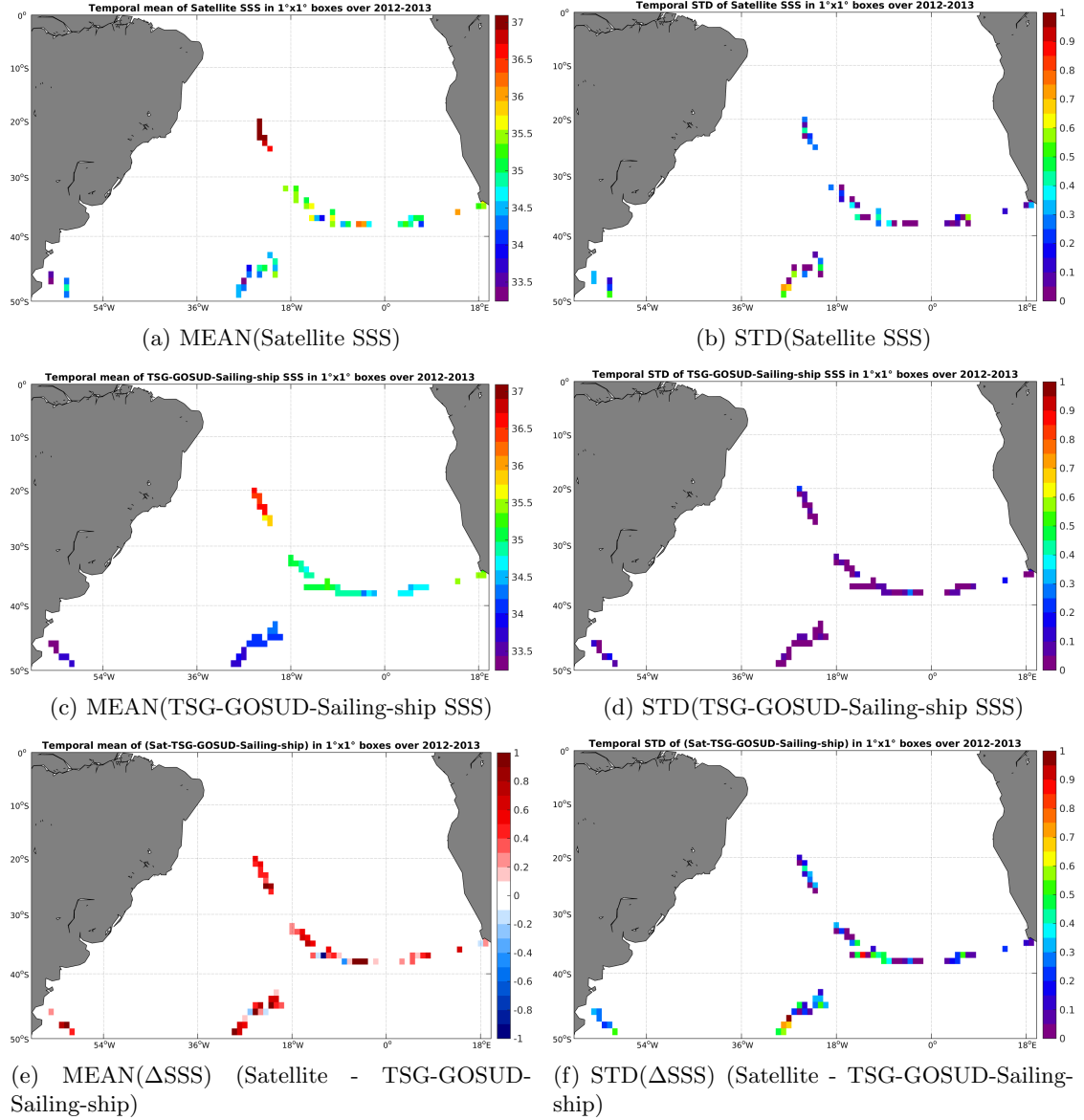
Figure 6: Temporal mean (left) and STD (right) of SSS from AQUARIUS-L2-JPL-V4 (top), TSG-GOSUD-Sailing-ship (middle), and of \Delta SSS (Satellite - TSG-GOSUD-Sailing-ship). Only match-up pairs are used to generate these maps.
