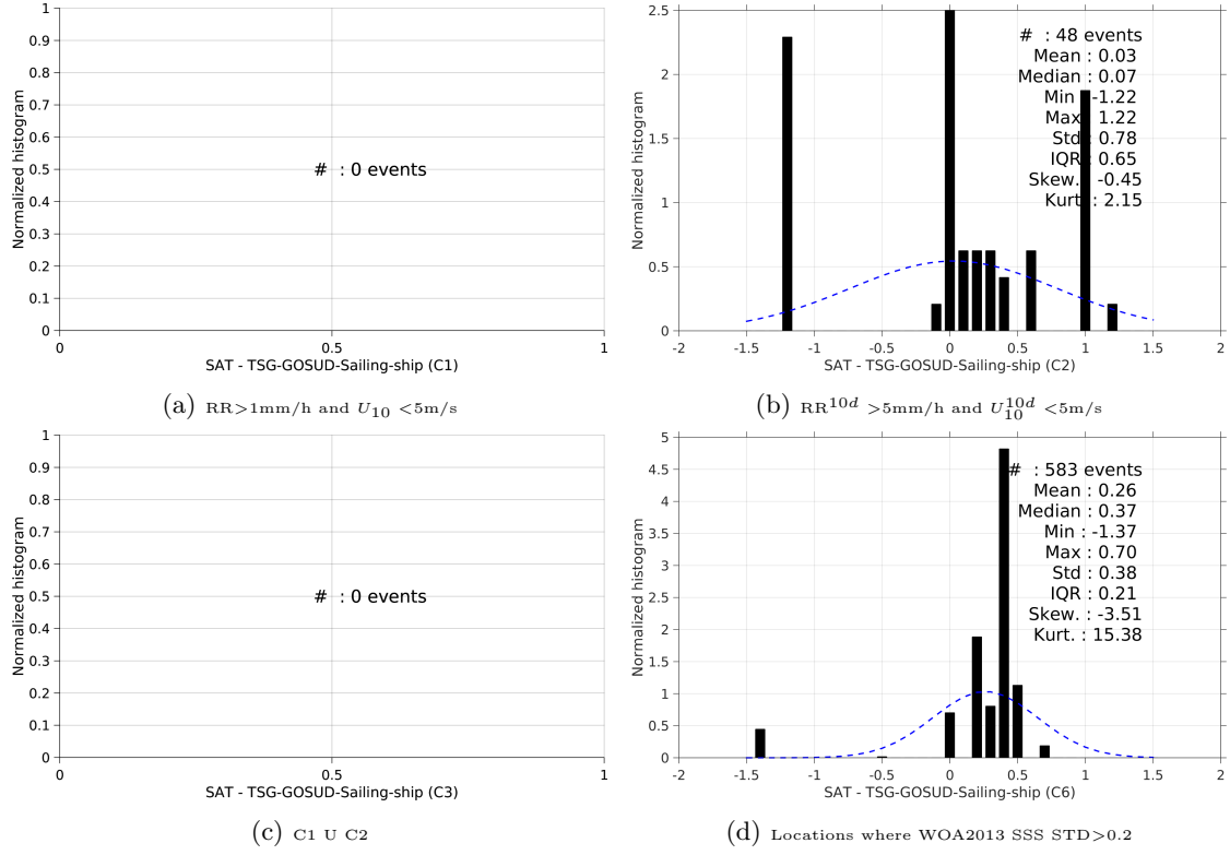
Figure 13: Normalized histogram of \Delta\text{SSS} (AQUARIUS-L2-JPL-V4 - TSG-GOSUD-Sailing-ship) for 6 different subdatasets corresponding to: RR > 1\text{mm/h} and U_{10} < 5\text{m/s} (a), RR^{10d} > 5\text{mm/h} and U_{10}^{10d} < 5\text{m/s} (b), C1 \cup C2 (c), Locations where WOA2013 SSS STD > 0.2 (d).
