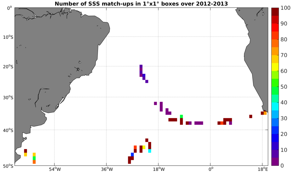
Figure 4: Number of SSS match-ups between TSG-GOSUD-Sailing-ship SSS and the AQUARIUS-L2-JPL-V4 SSS product for the South Atlantic Ocean Pi-MEP region over 1^\circ \times 1^\circ boxes and for the full satellite product period.
