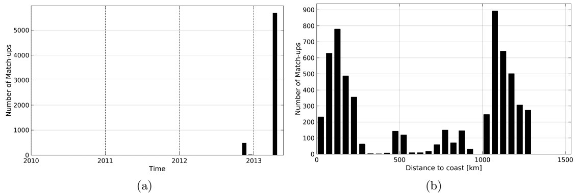
Figure 1: Number of match-ups between TSG-GOSUD-Sailing-ship and AQUARIUS-L2-JPL-V4 SSS as a function of time (a) and as function of the distance to coast (b) over the South Atlantic Ocean Pi-MEP region and for the full satellite product period.
