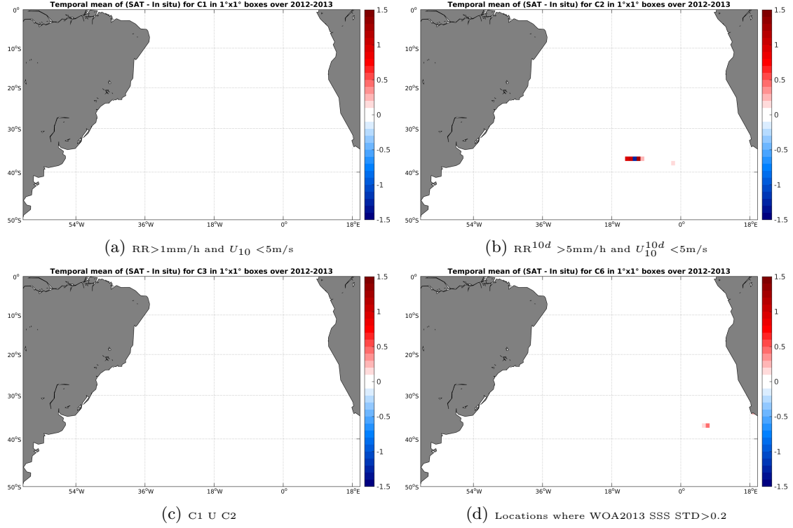
Figure 12: Temporal mean gridded over spatial boxes of size 1^\circ \times 1^\circ of \Delta SSS (AQUARIUS-L2-JPL-V4 - TSG-GOSUD-Sailing-ship) for 4 different subdatasets corresponding to: RR > 1\text{mm/h} and U_{10} < 5\text{m/s} (a), RR^{10d} > 5\text{mm/h} and U_{10}^{10d} < 5\text{m/s} (b), C1 U C2 (c), Locations where WOA2013 SSS STD > 0.2 (d).
