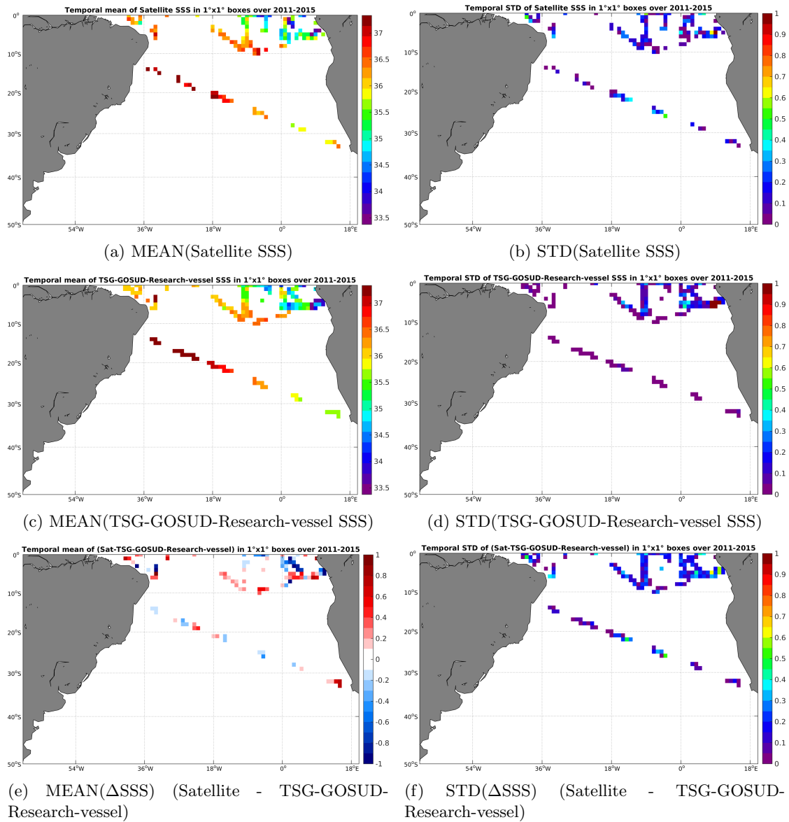
Figure 6: Temporal mean (left) and STD (right) of SSS from AQUARIUS-L2-JPL-V4 (top), TSG-GOSUD-Research-vessel (middle), and of \Delta SSS (Satellite - TSG-GOSUD-Research-vessel). Only match-up pairs are used to generate these maps.
