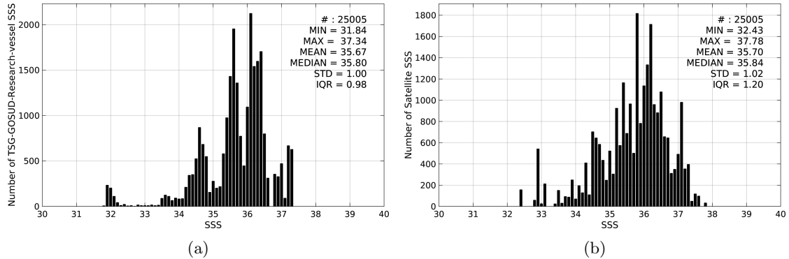
Figure 2: Histograms of SSS from TSG-GOSUD-Research-vessel (a) and AQUARIUS-L2-JPL-V4 (b) considering all match-up pairs per bins of 0.1 over the South Atlantic Ocean Pi-MEP region and for the full satellite product period.
