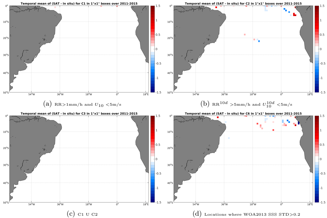
Figure 12: Temporal mean gridded over spatial boxes of size 1°x1° of \Delta SSS (AQUARIUS-L2-JPL-V4 - TSG-GOSUD-Research-vessel) for 4 different subdatasets corresponding to: RR > 1mm/h and U_{10} < 5 m/s (a), RR^{10d} > 5 mm/h and U_{10}^{10d} < 5 m/s (b), C1 U C2 (c), Locations where WOA2013 SSS STD > 0.2 (d).
