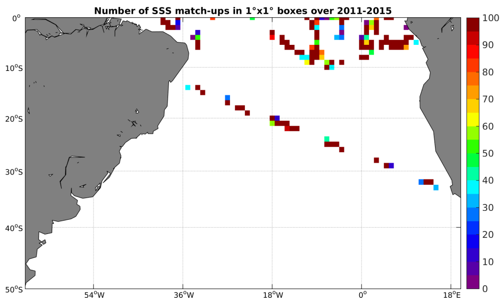
Figure 4: Number of SSS match-ups between TSG-GOSUD-Research-vessel SSS and the AQUARIUS-L2-JPL-V4 SSS product for the South Atlantic Ocean Pi-MEP region over 1°x1° boxes and for the full satellite product period.
