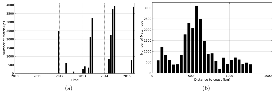
Figure 1: Number of match-ups between TSG-GOSUD-Research-vessel and AQUARIUS-L2-JPL-V4 SSS as a function of time (a) and as function of the distance to the coast (b) over the South Atlantic Ocean Pi-MEP region and for the full satellite product period.
