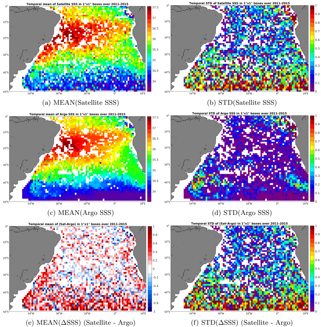
Figure 6: Temporal mean (left) and STD (right) of SSS from AQUARIUS-L2-JPL-V4 (top), Argo (middle), and of \Delta SSS (Satellite - Argo). Only match-up pairs are used to generate these maps.
