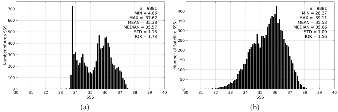
Figure 2: Histograms of SSS from Argo (a) and AQUARIUS-L2-JPL-V4 (b) considering all match-up pairs per bins of 0.1 over the South Atlantic Ocean Pi-MEP region and for the full satellite product period.
