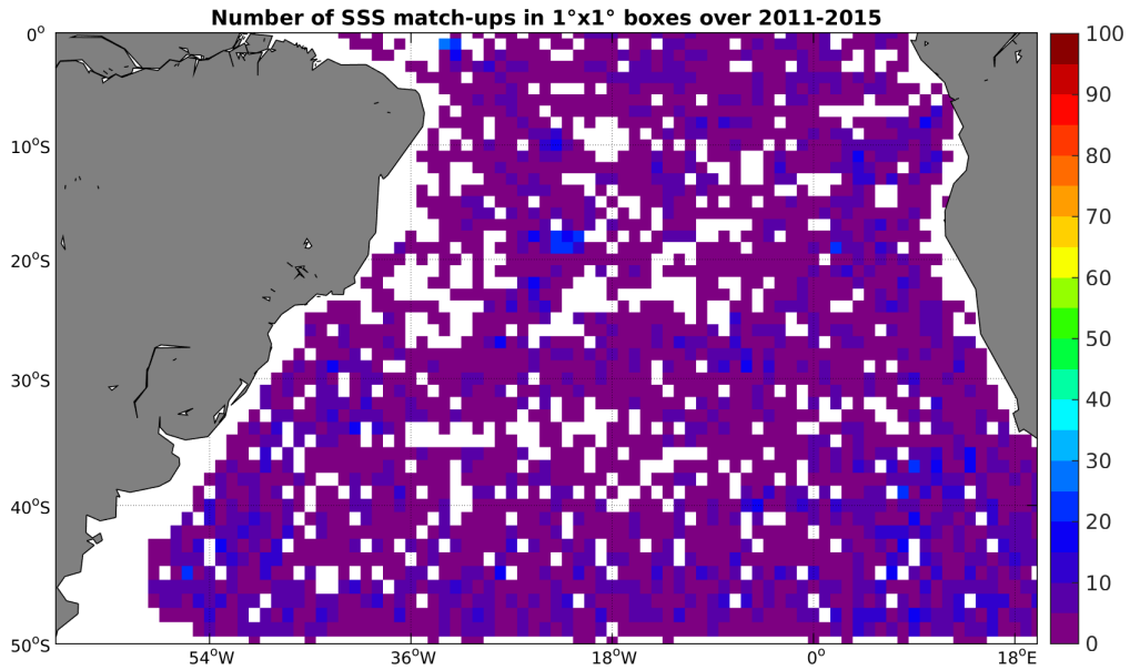
Figure 4: Number of SSS match-ups between Argo SSS and the AQUARIUS-L2-JPL-V4 SSS product for the South Atlantic Ocean Pi-MEP region over 1°x1° boxes and for the full satellite product period.
