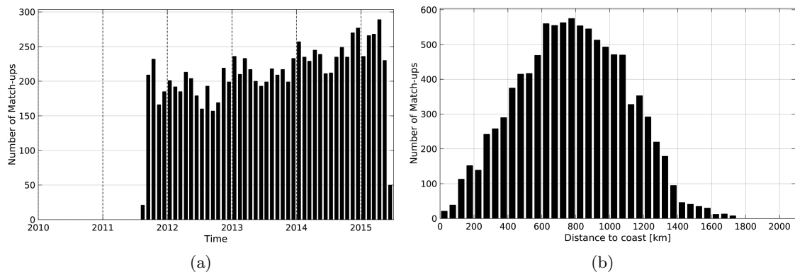
Figure 1: Number of match-ups between Argo and AQUARIUS-L2-JPL-V4 SSS as a function of time (a) and as function of the distance to coast (b) over the South Atlantic Ocean Pi-MEP region and for the full satellite product period.
