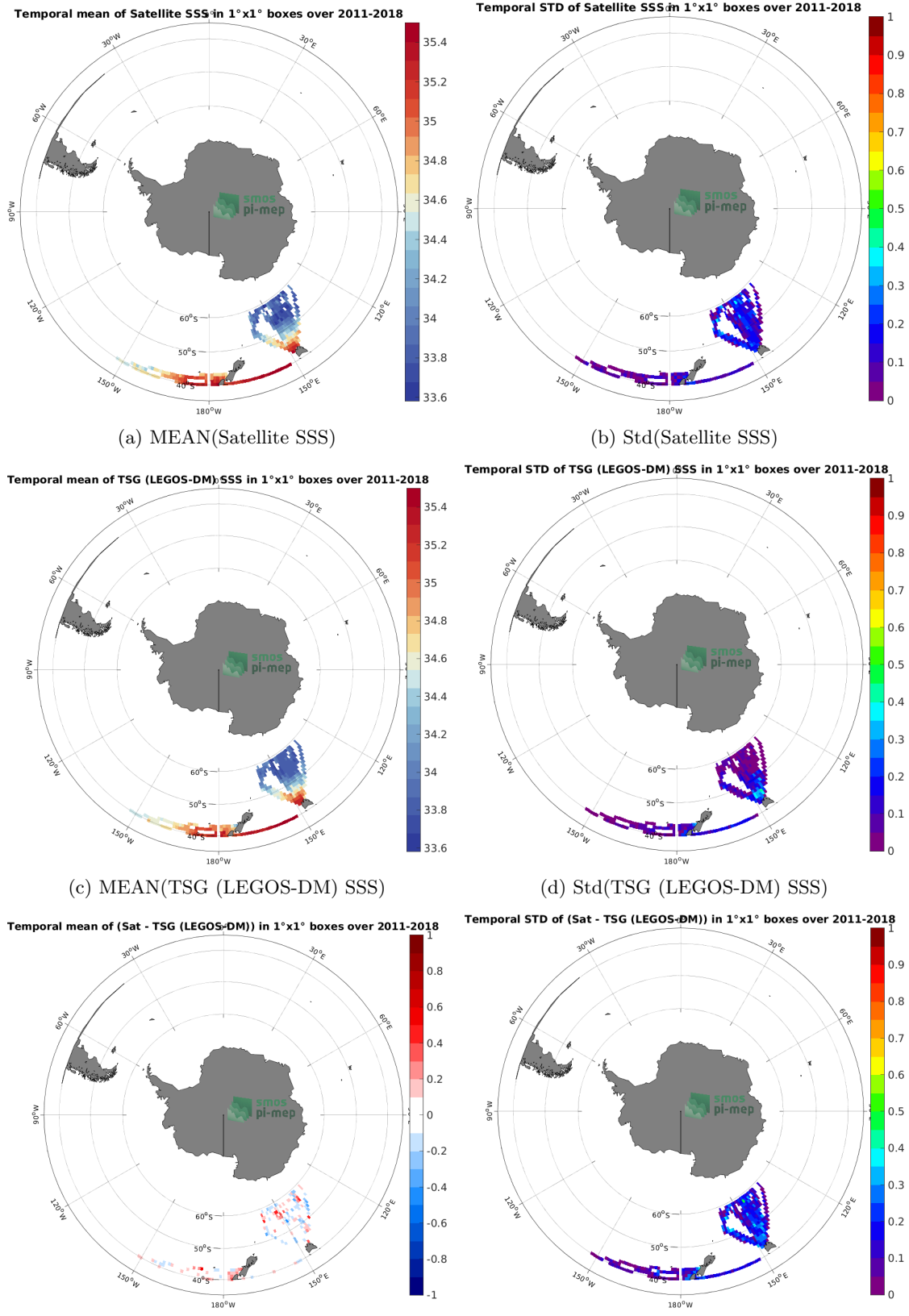
(e) MEAN( \Delta SSS) (Satellite - TSG (LEGOS-DM)) (f) Std( \Delta SSS) (Satellite - TSG (LEGOS-DM))
