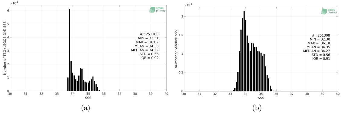
Figure 2: Histograms of SSS from TSG (LEGOS-DM) (a) and SMOS and SMAP SSS L4 OI v1 - 7 Days (LOPS) (b) considering all match-up pairs per bins of 0.1 over the Roaring Forties and Furious Fifties Pi-MEP region and for the full satellite product period.
