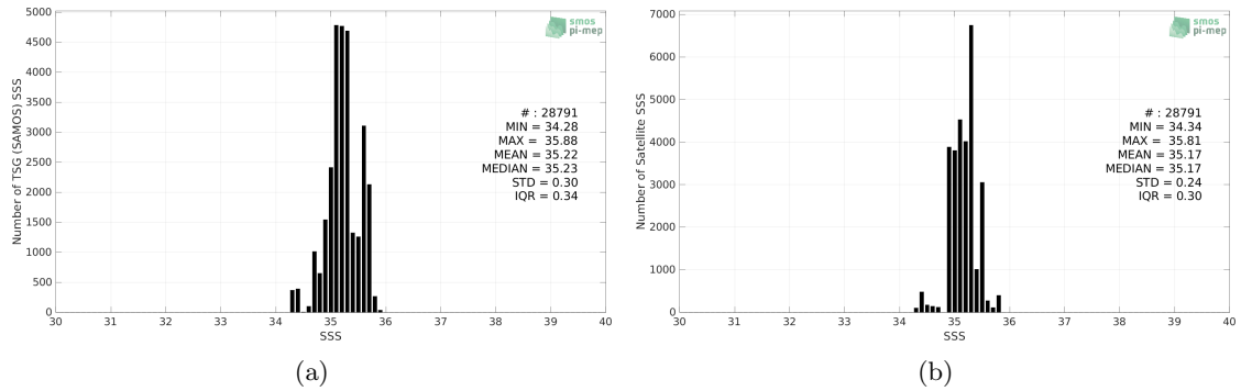
Figure 2: Histograms of SSS from TSG (SAMOS) (a) and SMOS SSS L4 v1 - Weekly (CMEMS-CNR) (b) considering all match-up pairs per bins of 0.1 over the Roaring Forties and Furious Fifties Pi-MEP region and for the full satellite product period.
