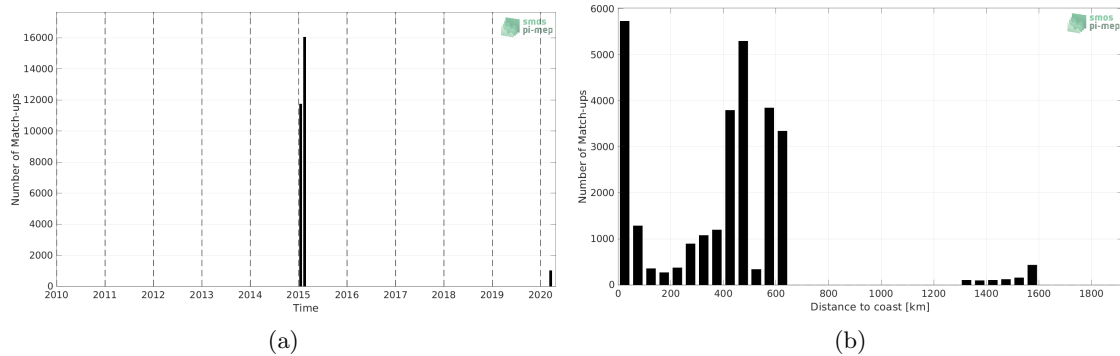
Figure 1: Number of match-ups between TSG (SAMOS) and SMOS SSS L4 v1 - Weekly (CMEMS-CNR) SSS as a function of time (a) and as function of the distance to coast (b) over the Roaring Forties and Furious Fifties Pi-MEP region and for the full satellite product period.
