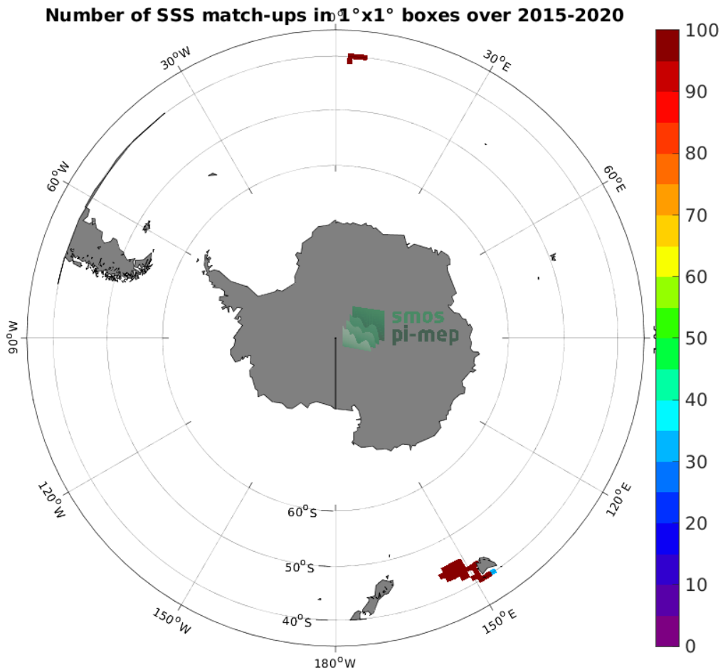
Figure 4: Number of SSS match-ups between TSG (SAMOS) SSS and the SMOS SSS L4 v1 - Weekly (CMEMS-CNR) SSS product for the Roaring Forties and Furious Fifties Pi-MEP region over 1^\circ \times 1^\circ boxes and for the full satellite product period.
