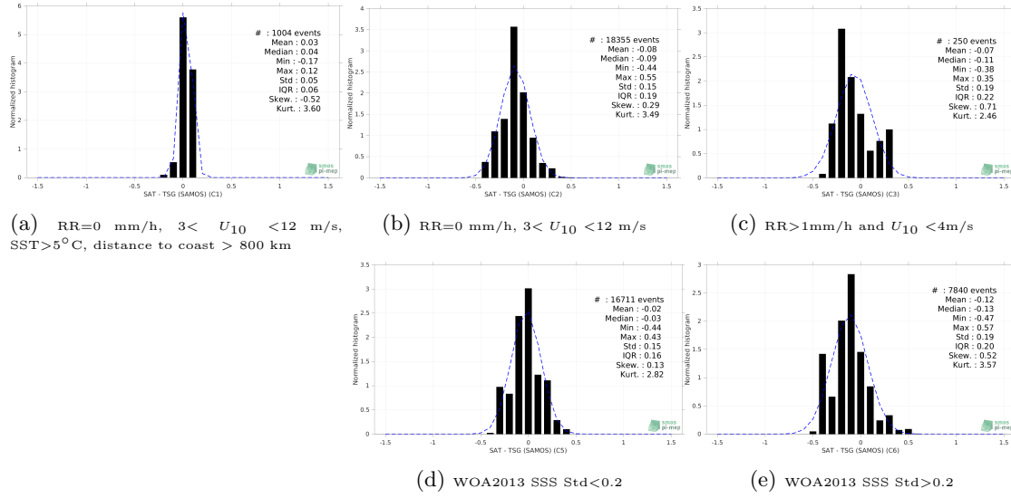
Figure 13: Normalized histogram of \Delta\text{SSS} (SMOS SSS L4 v1 - Weekly (CMEMS-CNR) - TSG (SAMOS)) for 5 different subdatasets corresponding to: RR=0 mm/h, 3 < U_{10} < 12 m/s, SST>5°C, distance to coast > 800 km (a), RR=0 mm/h, 3 < U_{10} < 12 m/s (b), RR>1mm/h and U_{10} < 4 m/s (c), WOA2013 SSS Std<0.2 (d), WOA2013 SSS Std>0.2 (e).
