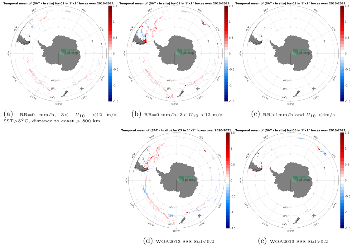
Figure 12: Temporal mean gridded over spatial boxes of size 1^\circ \times 1^\circ of \Delta\text{SSS} (SMOS SSS L4 v1 - Weekly (CMEMS-CNR) - TSG (GOSUD-Sailing-ship)) for 5 different subdatasets corresponding to: RR=0 mm/h, 3 < U_{10} < 12 m/s, SST > 5^\circ\text{C} , distance to coast > 800 km (a), RR=0 mm/h, 3 < U_{10} < 12 m/s (b), RR > 1 mm/h and U_{10} < 4 m/s (c), WOA2013 SSS Std < 0.2 (d), WOA2013 SSS Std > 0.2 (e).
