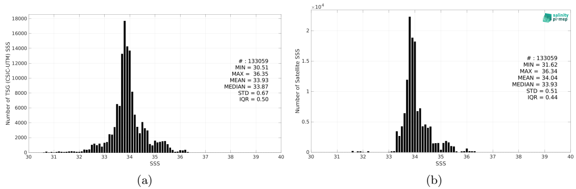
Figure 2: Histograms of SSS from TSG (CSIC-UTM) (a) and SMOS SSS L4 v1 - Weekly (CMEMS-CNR) (b) considering all match-up pairs per bins of 0.1 over the Roaring Forties and Furious Fifties Pi-MEP region and for the full satellite product period.
