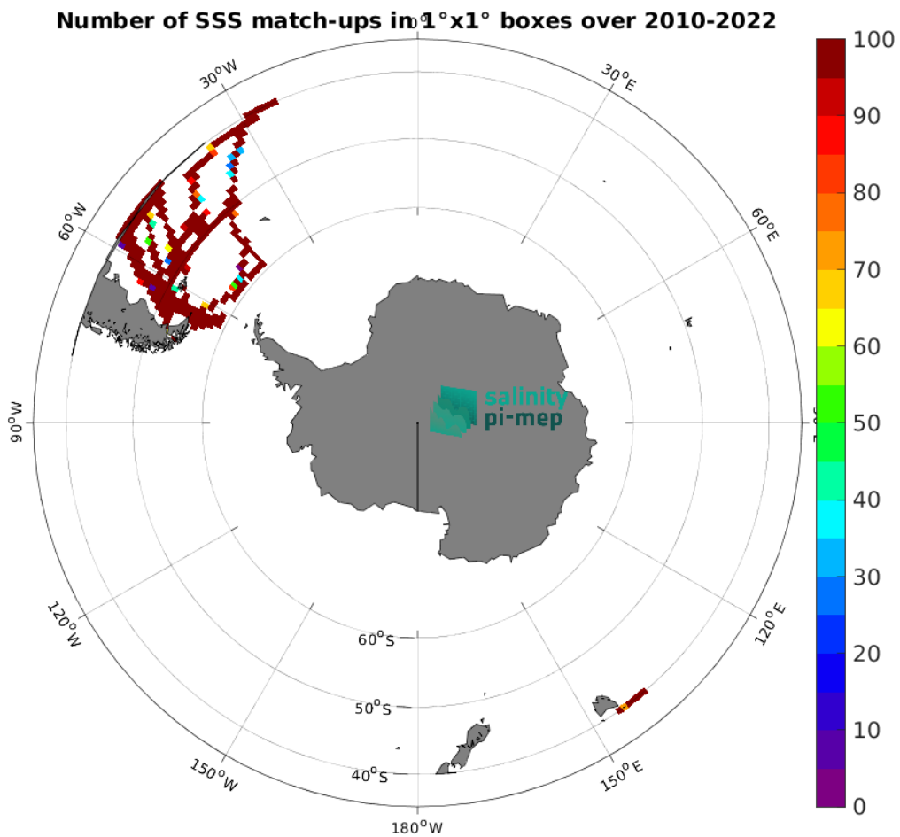
Figure 4: Number of SSS match-ups between TSG (CSIC-UTM) SSS and the SMOS SSS L4 v1 - Weekly (CMEMS-CNR) SSS product for the Roaring Forties and Furious Fifties Pi-MEP region over 1^\circ \times 1^\circ boxes and for the full satellite product period.
