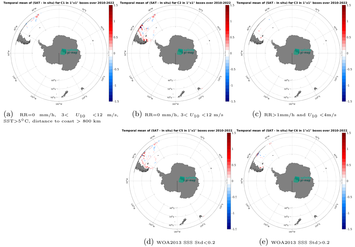
Figure 12: Temporal mean gridded over spatial boxes of size 1^{\circ}\times 1^{\circ} of \Delta\text{SSS} (SMOS SSS L4 v1 - Weekly (CMEMS-CNR) - TSG (CSIC-UTM)) for 5 different subdatasets corresponding to:RR=0 mm/h, 3 < U_{10} < 12 m/s, SST >5^{\circ}\text{C} , distance to coast > 800 km (a), RR=0 mm/h, 3 < U_{10} < 12 m/s (b), RR >1 mm/h and U_{10} < 4 m/s (c), WOA2013 SSS Std <0.2 (d), WOA2013 SSS Std >0.2 (e).
