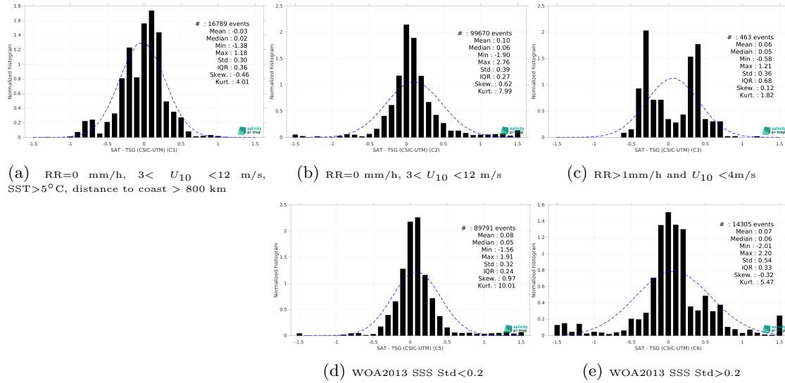
Figure 13: Normalized histogram of \Delta\text{SSS} (SMOS SSS L4 v1 - Weekly (CMEMS-CNR) - TSG (CSIC-UTM)) for 5 different subdatasets corresponding to: RR=0 mm/h, 3 < U_{10} < 12 m/s, SST>5°C, distance to coast > 800 km (a), RR=0 mm/h, 3 < U_{10} < 12 m/s (b), RR>1mm/h and U_{10} < 4 m/s (c), WOA2013 SSS Std<0.2 (d), WOA2013 SSS Std>0.2 (e).
