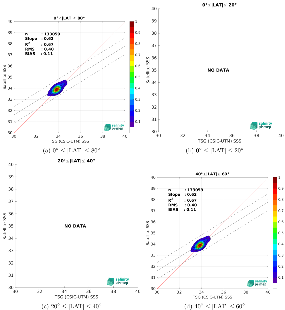
Figure 9: Contour maps of the concentration of SMOS SSS L4 v1 - Weekly (CMEMS-CNR) SSS (y-axis) versus TSG (CSIC-UTM) SSS (x-axis) at match-up pairs for different latitude bands. For each plot, the red line shows x=y . The black thin and dashed lines indicate a linear fit through the data cloud and the \pm 95\% confidence levels, respectively. The number match-up pairs n , the slope and R^2 coefficient of the linear fit, the root mean square (RMS) and the mean bias between satellite and in situ data are indicated for each latitude band in each plots.
