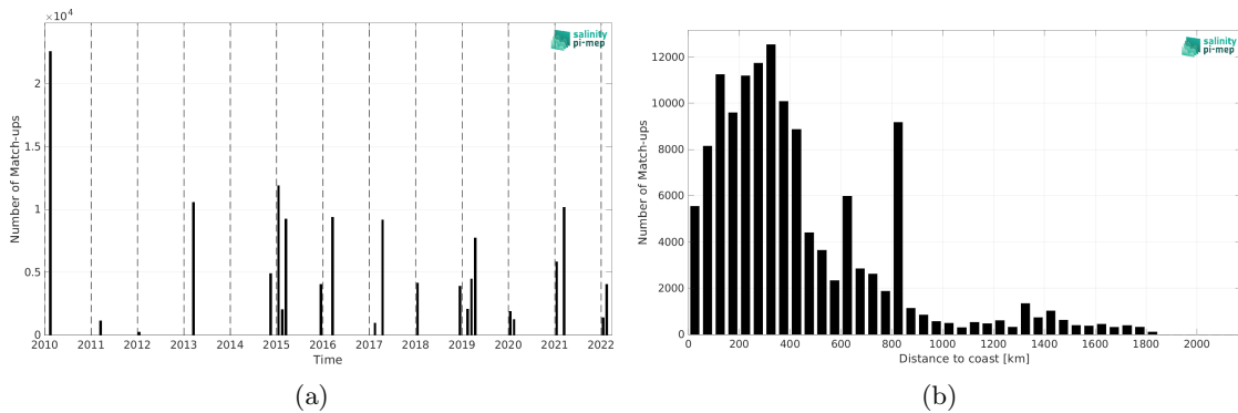
Figure 1: Number of match-ups between TSG (CSIC-UTM) and SMOS SSS L4 v1 - Weekly (CMEMS-CNR) SSS as a function of time (a) and as function of the distance to coast (b) over the Roaring Forties and Furious Fifties Pi-MEP region and for the full satellite product period.
