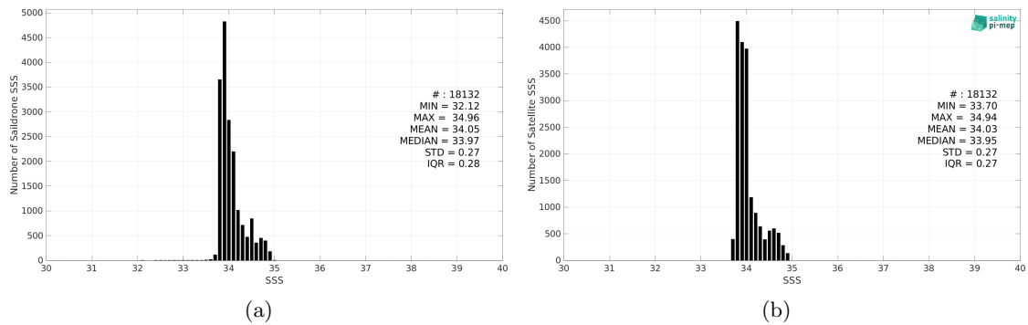
Figure 2: Histograms of SSS from Saildrone (a) and SMOS SSS L4 v1 - Weekly (CMEMS-CNR) (b) considering all match-up pairs per bins of 0.1 over the Roaring Forties and Furious Fifties Pi-MEP region and for the full satellite product period.
