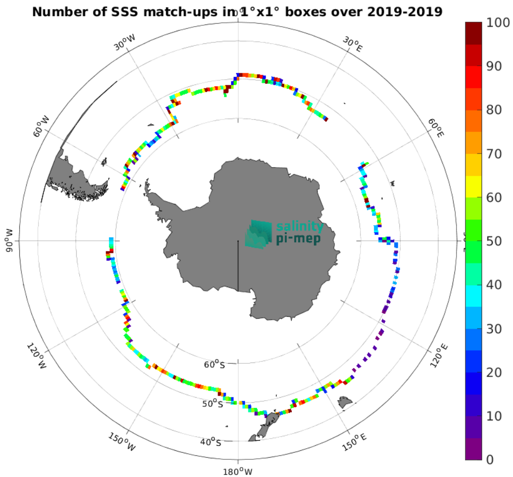
Figure 4: Number of SSS match-ups between Saildrone SSS and the SMOS SSS L4 v1 - Weekly (CMEMS-CNR) SSS product for the Roaring Forties and Furious Fifties Pi-MEP region over 1^\circ \times 1^\circ boxes and for the full satellite product period.
