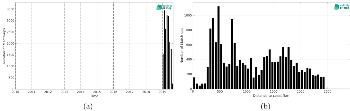
Figure 1: Number of match-ups between Saildrone and SMOS SSS L4 v1 - Weekly (CMEMS-CNR) SSS as a function of time (a) and as function of the distance to coast (b) over the Roaring Forties and Furious Fifties Pi-MEP region and for the full satellite product period.
