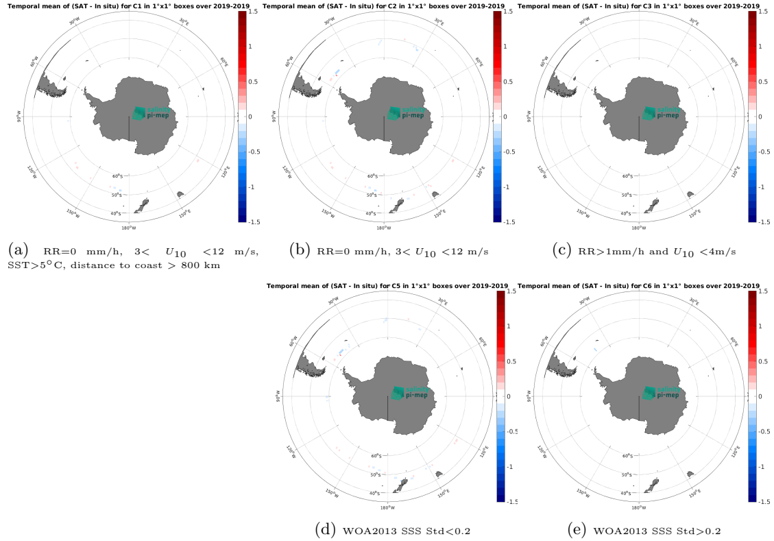
Figure 12: Temporal mean gridded over spatial boxes of size 1^{\circ}\times 1^{\circ} of \Delta\text{SSS} (SMOS SSS L4 v1 - Weekly (CMEMS-CNR) - Saildrone) for 5 different subdatasets corresponding to:RR=0 mm/h, 3 < U_{10} < 12 m/s, SST >5^{\circ}\text{C} , distance to coast > 800 km (a), RR=0 mm/h, 3 < U_{10} < 12 m/s (b), RR >1 mm/h and U_{10} < 4 m/s (c), WOA2013 SSS Std <0.2 (d), WOA2013 SSS Std >0.2 (e).
