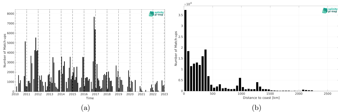
Figure 1: Number of match-ups between TSG (SAMOS) and SMOS SSS L4 v1 - Monthly (CMEMS-CNR) SSS as a function of time (a) and as function of the distance to coast (b) over the Roaring Forties and Furious Fifties Pi-MEP region and for the full satellite product period.
