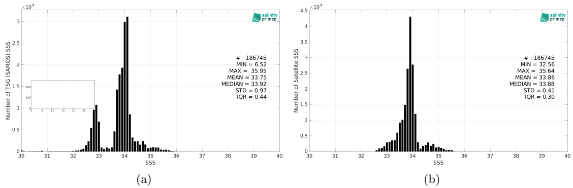
Figure 2: Histograms of SSS from TSG (SAMOS) (a) and SMOS SSS L4 v1 - Monthly (CMEMS-CNR) (b) considering all match-up pairs per bins of 0.1 over the Roaring Forties and Furious Fifties Pi-MEP region and for the full satellite product period.
