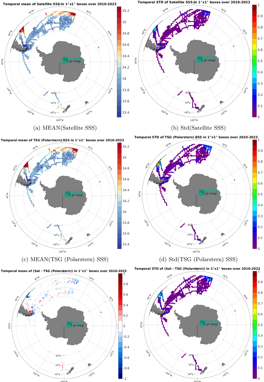
Figure 7: Temporal mean (left) and Std (right) of SSS from SMOS SSS L4 v1 - Monthly (CMEMS-CNR) (top), TSG (Polarstern) (middle), and of \Delta SSS (Satellite - TSG (Polarstern)). Only match-up pairs are used to generate these maps.
