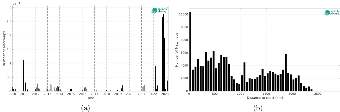
Figure 2: Number of match-ups between TSG (Polarstern) and SMOS SSS L4 v1 - Monthly (CMEMS-CNR) SSS as a function of time (a) and as function of the distance to coast (b) over the Roaring Forties and Furious Fifties Pi-MEP region and for the full satellite product period.
