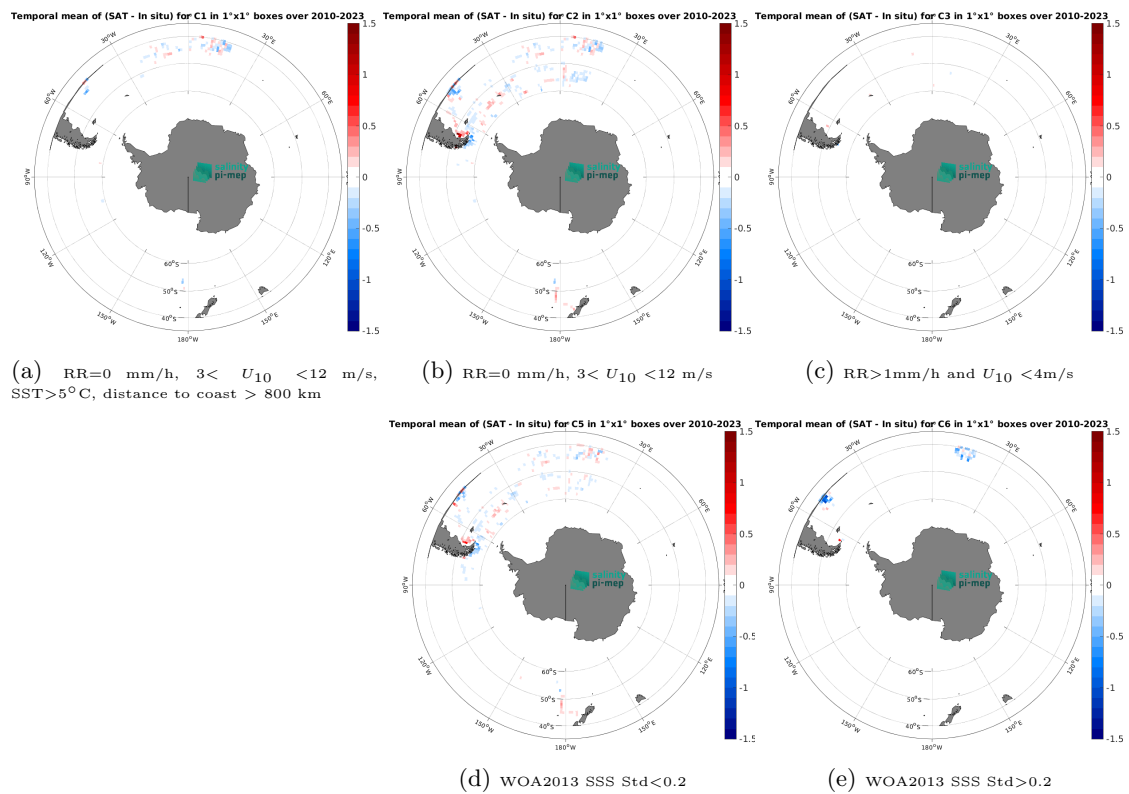
Figure 14: Temporal mean gridded over spatial boxes of size 1^\circ \times 1^\circ of \Delta SSS (SMOS SSS L4 v1 - Monthly (CMEMS-CNR) - TSG (Polarstern)) for 5 different subdatasets corresponding to:RR=0 mm/h, 3 < U_{10} < 12 m/s, SST>5°C, distance to coast > 800 km (a), RR=0 mm/h, 3 < U_{10} < 12 m/s (b), RR>1mm/h and U_{10} < 4 m/s (c), WOA2013 SSS Std<0.2 (d), WOA2013 SSS Std>0.2 (e).
